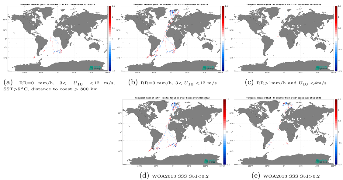
Figure 14: Temporal mean gridded over spatial boxes of size 1^\circ \times 1^\circ of \Delta SSS (SMAP SSS L2 v6 (RSS) - TSG (Polarstern)) for 5 different subdatasets corresponding to:RR=0 mm/h, 3 < U_{10} < 12 m/s, SST > 5^\circ\text{C} , distance to coast > 800 km (a), RR=0 mm/h, 3 < U_{10} < 12 m/s (b), RR > 1 mm/h and U_{10} < 4 m/s (c), WOA2013 SSS Std < 0.2 (d), WOA2013 SSS Std > 0.2 (e).
