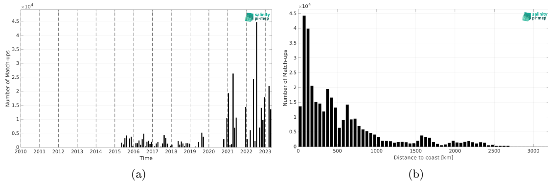
Figure 2: Number of match-ups between TSG (Polarstern) and SMAP SSS L2 v6 (RSS) SSS as a function of time (a) and as function of the distance to coast (b) over the Global Ocean Pi-MEP region and for the full satellite product period.
