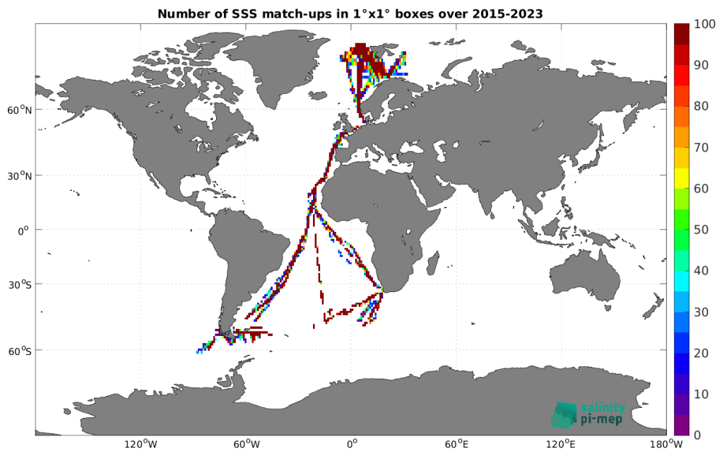
Figure 5: Number of SSS match-ups between TSG (Polarstern) SSS and the SMAP SSS L2 v6 (RSS) SSS product for the Global Ocean Pi-MEP region over 1^\circ \times 1^\circ boxes and for the full satellite product period.
