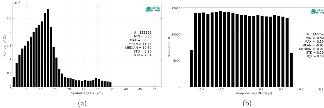
Figure 6: Histograms of the spatial (a) and temporal (b) lags between the location/time of the TSG (Polarstern) measurement and the date of the corresponding SMAP SSS L2 v6 (RSS) SSS pixel.
