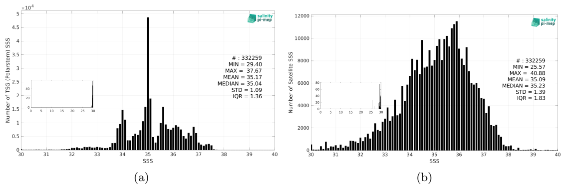
Figure 3: Histograms of SSS from TSG (Polarstern) (a) and SMAP SSS L2 v6 (RSS) (b) considering all match-up pairs per bins of 0.1 over the Global Ocean Pi-MEP region and for the full satellite product period.
