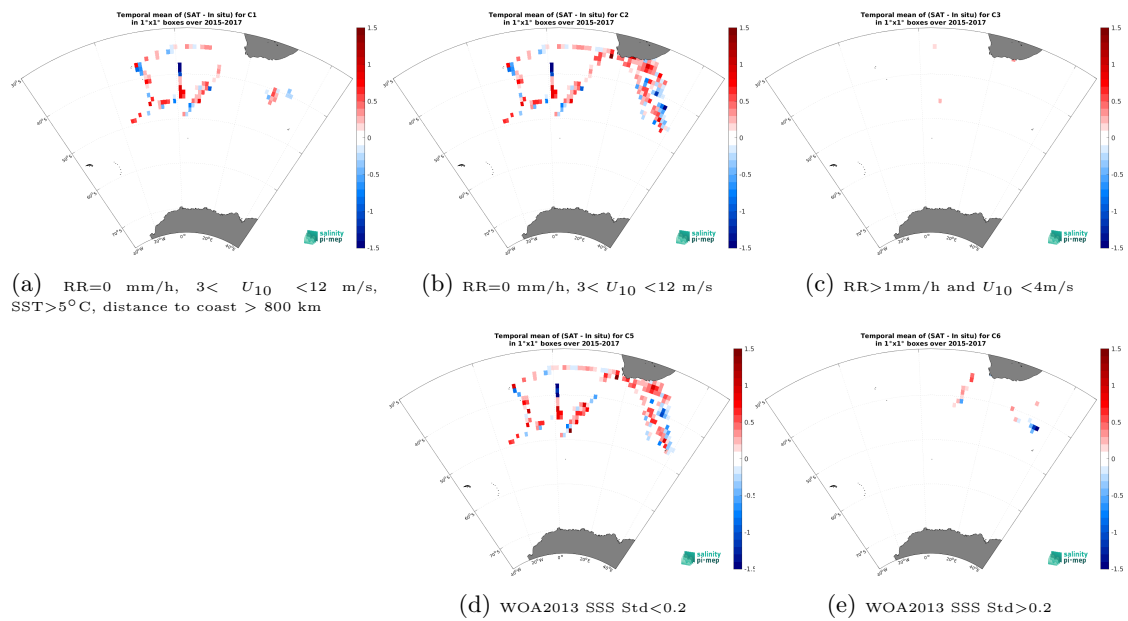
Figure 14: Temporal mean gridded over spatial boxes of size 1^\circ \times 1^\circ of \Delta SSS (SMAP SSS L2 v6 (RSS) - TSG (NCEI-0170743)) for 5 different subdatasets corresponding to:RR=0 mm/h, 3 < U_{10} < 12 m/s, SST >5^\circ\text{C} , distance to coast > 800 km (a), RR=0 mm/h, 3 < U_{10} < 12 m/s (b), RR >1 mm/h and U_{10} < 4 m/s (c), WOA2013 SSS Std <0.2 (d), WOA2013 SSS Std >0.2 (e).
