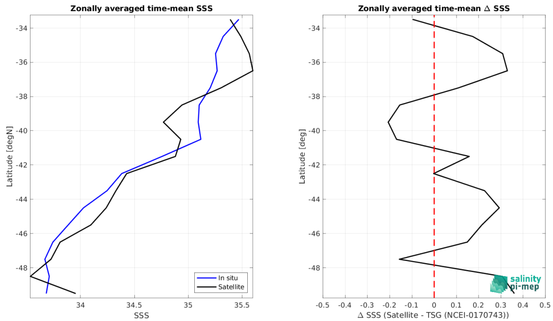
Figure 9: Left panel: Zonal mean SSS from SMAP SSS L2 v6 (RSS) satellite product (black) and from TSG (NCEI-0170743) (blue). Right panel: Zonal mean of \Delta SSS (Satellite - TSG (NCEI-0170743)) for all the collected Pi-MEP match-up pairs estimated over the full satellite product period.
