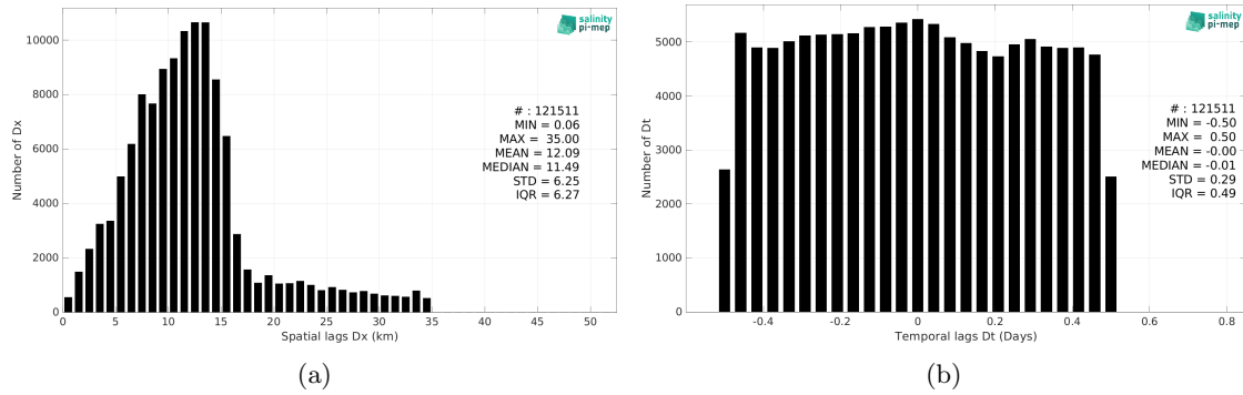
Figure 6: Histograms of the spatial (a) and temporal (b) lags between the location/time of the TSG (NCEI-0170743) measurement and the date of the corresponding SMAP SSS L2 v6 (RSS) SSS pixel.
