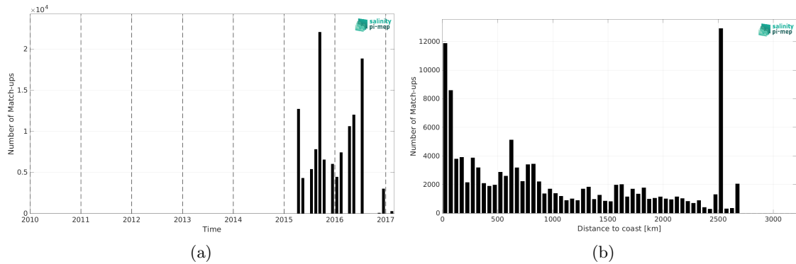
Figure 2: Number of match-ups between TSG (NCEI-0170743) and SMAP SSS L2 v6 (RSS) SSS as a function of time (a) and as function of the distance to coast (b) over the Global Ocean Pi-MEP region and for the full satellite product period.
