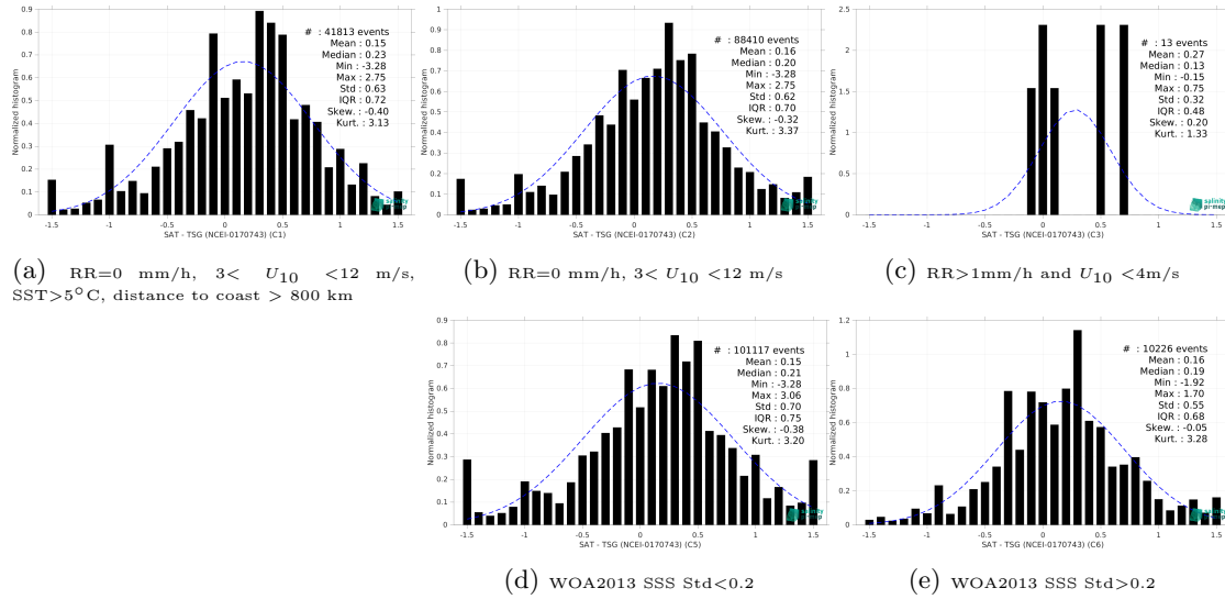
Figure 15: Normalized histogram of \Delta SSS (SMAP SSS L2 v6 (RSS) - TSG (NCEI-0170743)) for 5 different subdatasets corresponding to: RR=0 mm/h, 3 < U_{10} < 12 m/s, SST > 5°C, distance to coast > 800 km (a), RR=0 mm/h, 3 < U_{10} < 12 m/s (b), RR > 1mm/h and U_{10} < 4 m/s (c), WOA2013 SSS Std < 0.2 (d), WOA2013 SSS Std > 0.2 (e).
