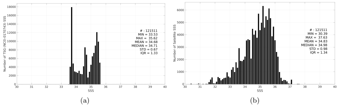
Figure 3: Histograms of SSS from TSG (NCEI-0170743) (a) and SMAP SSS L2 v6 (RSS) (b) considering all match-up pairs per bins of 0.1 over the Global Ocean Pi-MEP region and for the full satellite product period.
