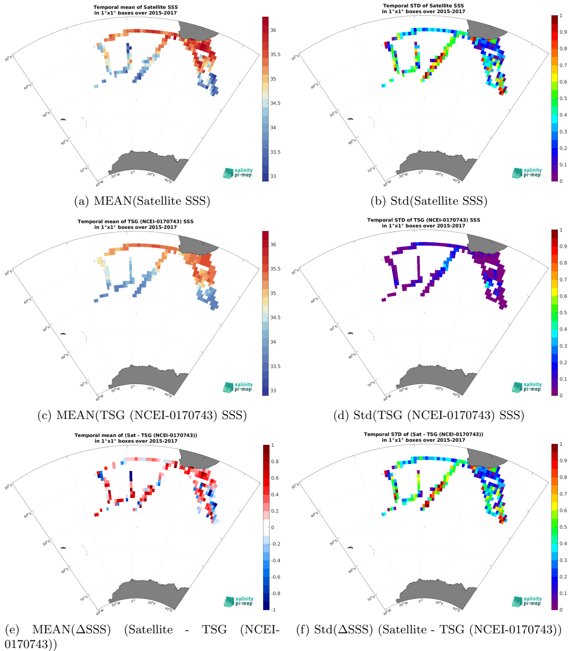
Figure 7: Temporal mean (left) and Std (right) of SSS from SMAP SSS L2 v6 (RSS) (top), TSG (NCEI-0170743) (middle), and of \Delta SSS (Satellite - TSG (NCEI-0170743)). Only match-up pairs are used to generate these maps.
