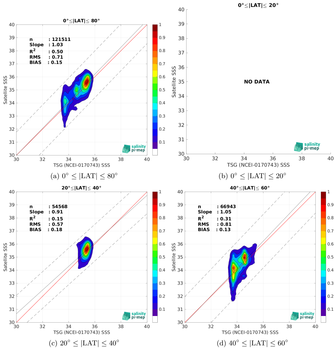
Figure 10: Contour maps of the concentration of SMAP SSS L2 v6 (RSS) SSS (y-axis) versus TSG (NCEI-0170743) SSS (x-axis) at match-up pairs for different latitude bands. For each plot, the red line shows x=y . The black thin and dashed lines indicate a linear fit through the data cloud and the \pm 95\% confidence levels, respectively. The number match-up pairs n , the slope and R^2 coefficient of the linear fit, the root mean square (RMS) and the mean bias between satellite and in situ data are indicated for each latitude band in each plots.
