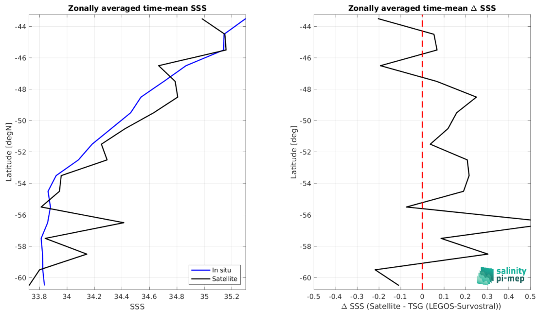
Figure 9: Left panel: Zonal mean SSS from SMAP SSS L2 v6 (RSS) satellite product (black) and from TSG (LEGOS-Survostral) (blue). Right panel: Zonal mean of \Delta SSS (Satellite - TSG (LEGOS-Survostral)) for all the collected Pi-MEP match-up pairs estimated over the full satellite product period.
