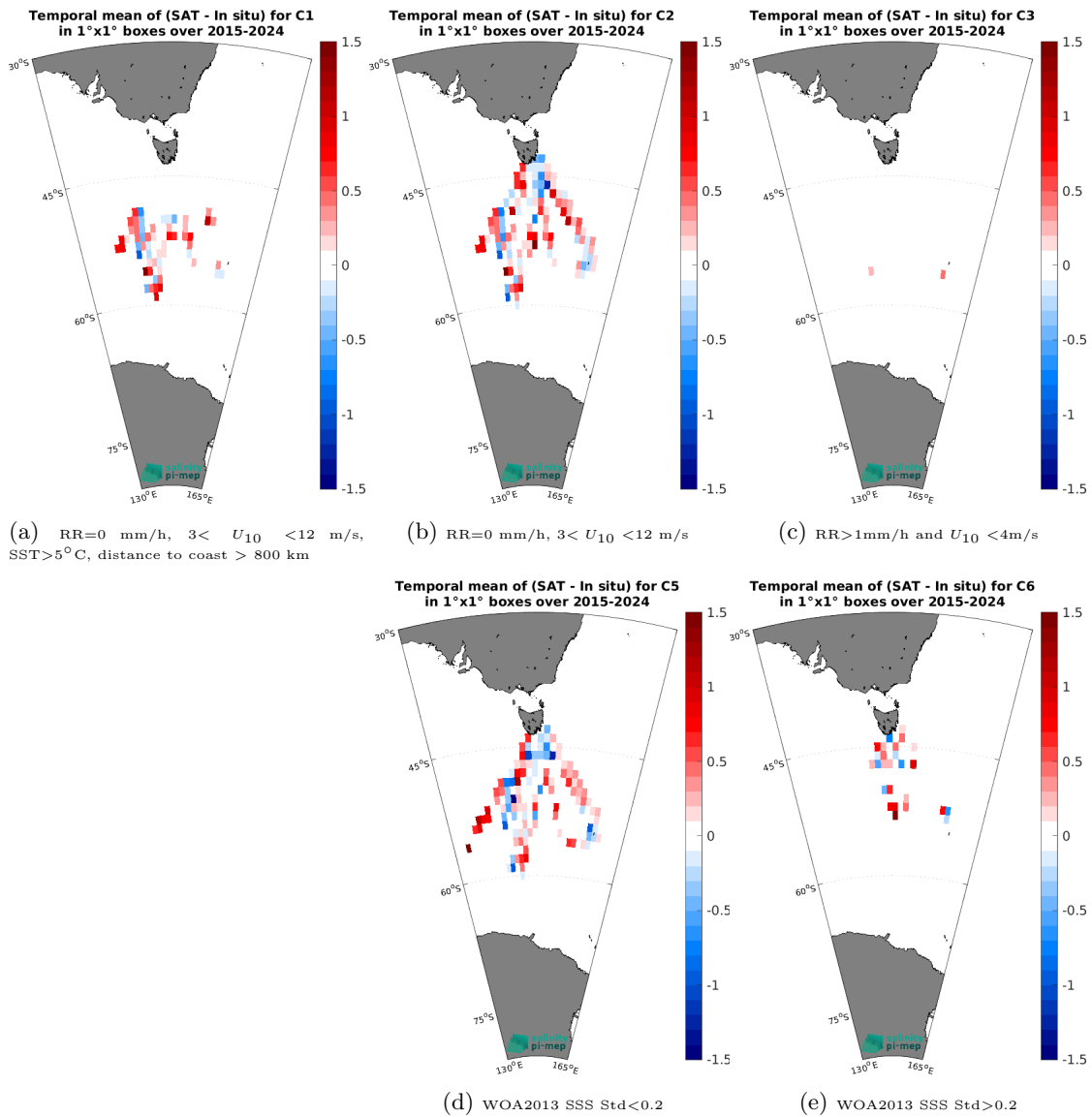
Figure 14: Temporal mean gridded over spatial boxes of size 1^{\circ} \times 1^{\circ} of \Delta\text{SSS} (SMAP SSS L2 v6 (RSS) - TSG (LEGOS-Survostral)) for 5 different subdatasets corresponding to: RR=0 mm/h, 3 < U_{10} < 12 m/s, SST > 5^{\circ}\text{C} , distance to coast > 800 km (a), RR=0 mm/h, 3 < U_{10} < 12 m/s (b), RR > 1\text{mm/h} and U_{10} < 4\text{m/s} (c), WOA2013 SSS Std < 0.2 (d), WOA2013 SSS Std > 0.2 (e).
