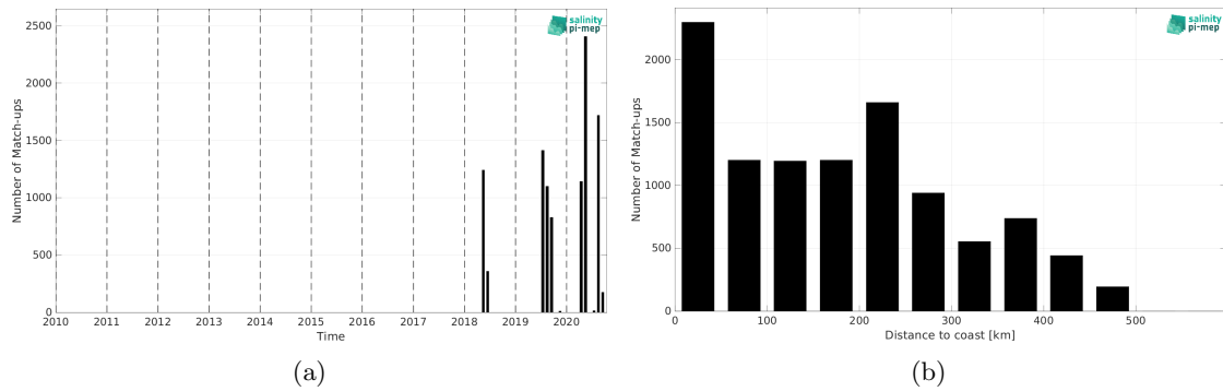
Figure 2: Number of match-ups between TSG (Lauge-Koch) and SMAP SSS L2 v6 (RSS) SSS as a function of time (a) and as function of the distance to coast (b) over the Global Ocean Pi-MEP region and for the full satellite product period.
