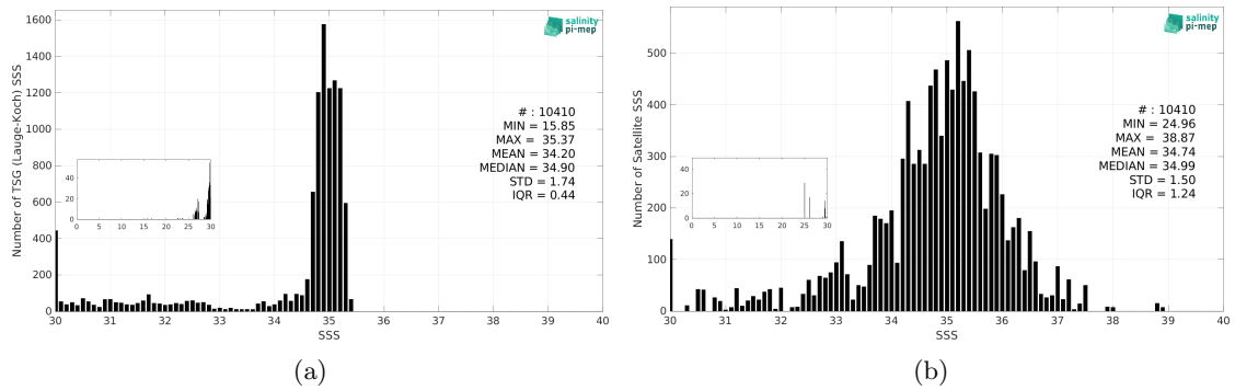
Figure 3: Histograms of SSS from TSG (Lauge-Koch) (a) and SMAP SSS L2 v6 (RSS) (b) considering all match-up pairs per bins of 0.1 over the Global Ocean Pi-MEP region and for the full satellite product period.
