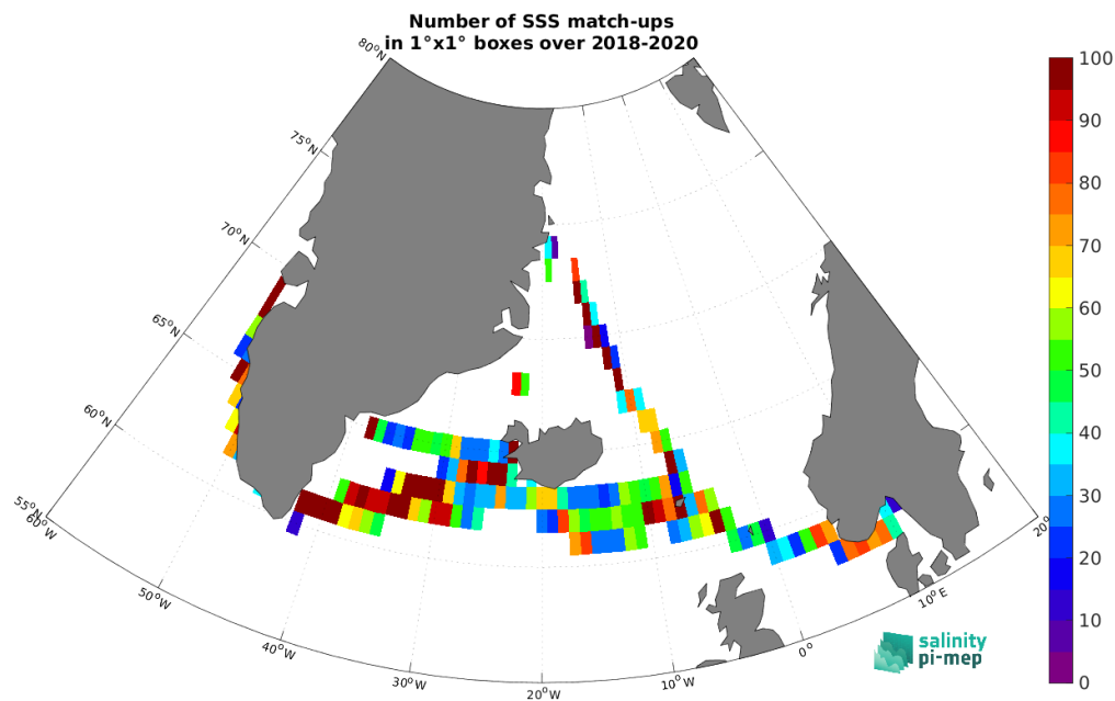
Figure 5: Number of SSS match-ups between TSG (Lauge-Koch) SSS and the SMAP SSS L2 v6 (RSS) SSS product for the Global Ocean Pi-MEP region over 1^\circ \times 1^\circ boxes and for the full satellite product period.
