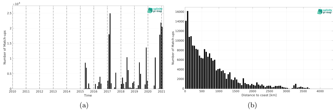
Figure 2: Number of match-ups between TSG (GOSUD-Sailing-ship) and SMAP SSS L2 v6 (RSS) SSS as a function of time (a) and as function of the distance to coast (b) over the Global Ocean Pi-MEP region and for the full satellite product period.
