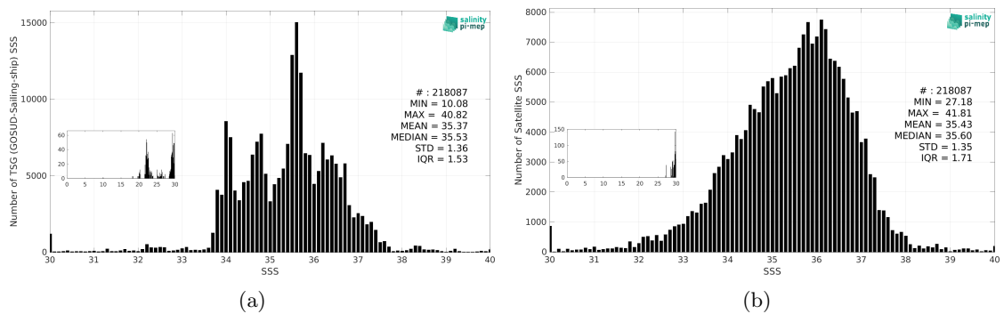
Figure 3: Histograms of SSS from TSG (GOSUD-Sailing-ship) (a) and SMAP SSS L2 v6 (RSS) (b) considering all match-up pairs per bins of 0.1 over the Global Ocean Pi-MEP region and for the full satellite product period.
