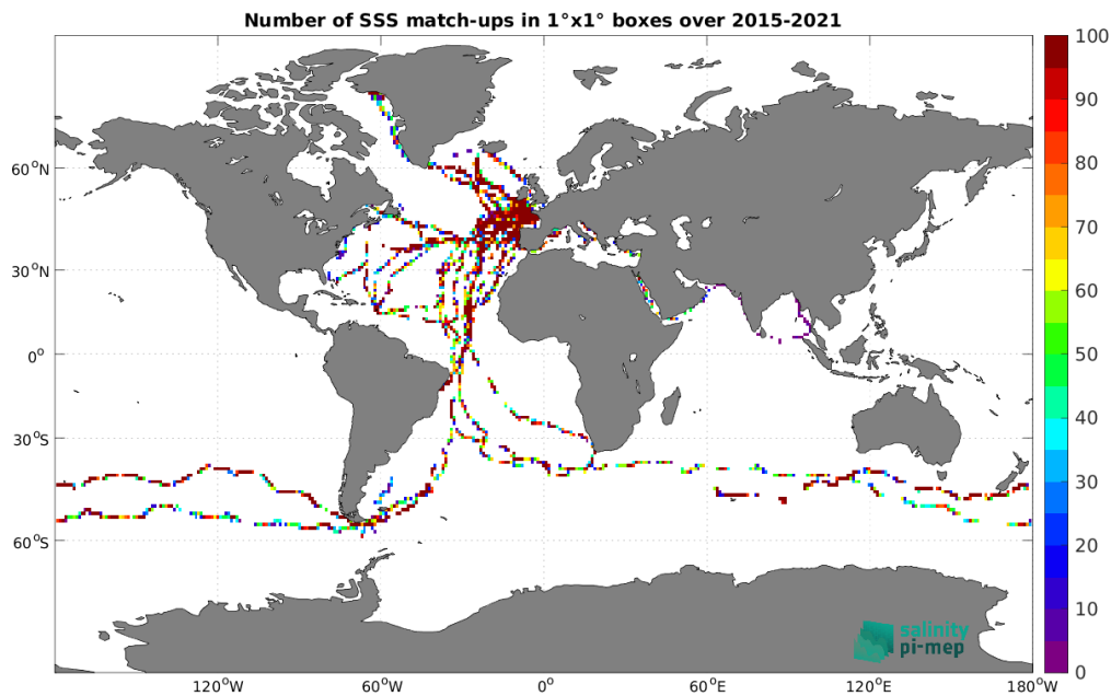
Figure 5: Number of SSS match-ups between TSG (GOSUD-Sailing-ship) SSS and the SMAP SSS L2 v6 (RSS) SSS product for the Global Ocean Pi-MEP region over 1^\circ \times 1^\circ boxes and for the full satellite product period.
