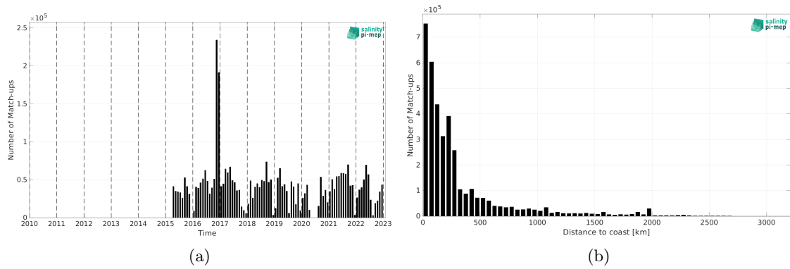
Figure 2: Number of match-ups between TSG (GOSUD-Research-vessel) and SMAP SSS L2 v6 (RSS) SSS as a function of time (a) and as function of the distance to coast (b) over the Global Ocean Pi-MEP region and for the full satellite product period.
