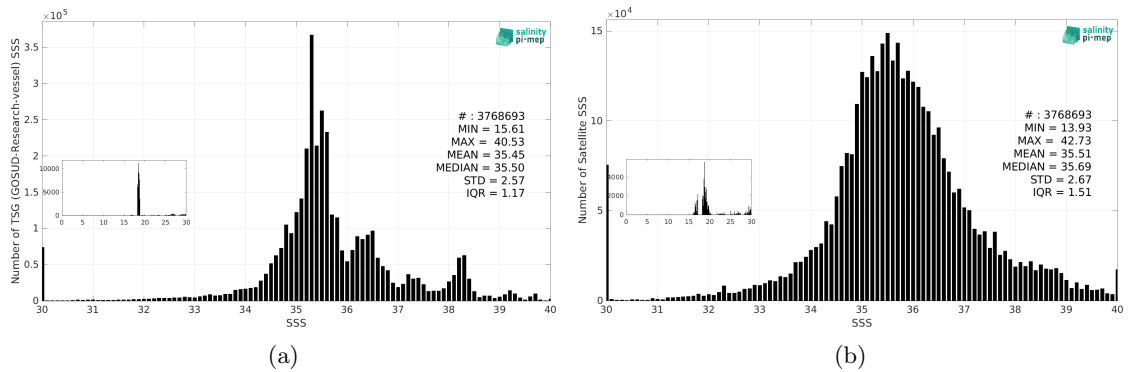
Figure 3: Histograms of SSS from TSG (GOSUD-Research-vessel) (a) and SMAP SSS L2 v6 (RSS) (b) considering all match-up pairs per bins of 0.1 over the Global Ocean Pi-MEP region and for the full satellite product period.
