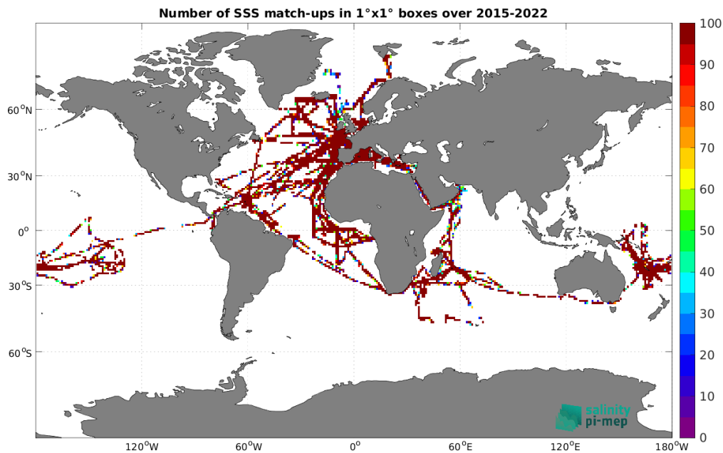
Figure 5: Number of SSS match-ups between TSG (GOSUD-Research-vessel) SSS and the SMAP SSS L2 v6 (RSS) SSS product for the Global Ocean Pi-MEP region over 1^\circ \times 1^\circ boxes and for the full satellite product period.
