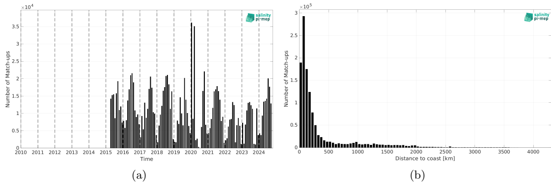
Figure 2: Number of match-ups between TSG (SAMOS) and SMAP SSS L2 v6 - 40 km (RSS) SSS as a function of time (a) and as function of the distance to coast (b) over the Global Ocean Pi-MEP region and for the full satellite product period.
