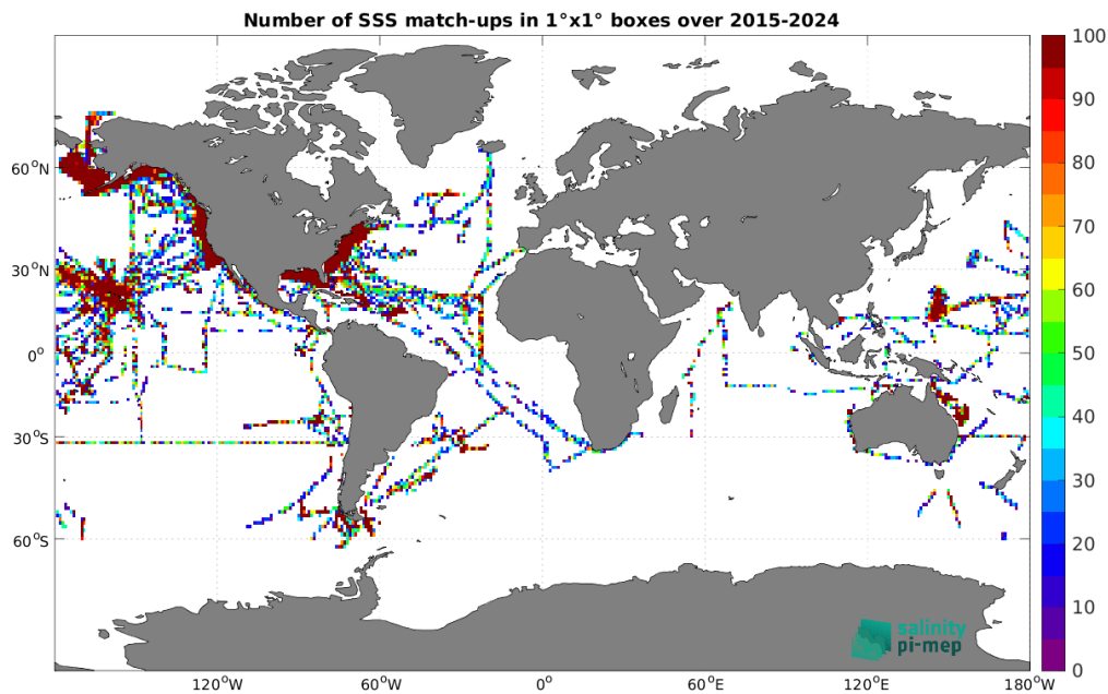
Figure 5: Number of SSS match-ups between TSG (SAMOS) SSS and the SMAP SSS L2 v6 - 40 km (RSS) SSS product for the Global Ocean Pi-MEP region over 1^\circ \times 1^\circ boxes and for the full satellite product period.
