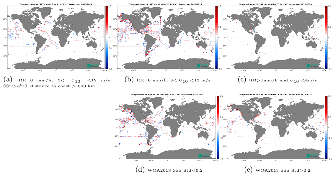
Figure 14: Temporal mean gridded over spatial boxes of size 1^\circ \times 1^\circ of \Delta SSS (SMAP SSS L2 v6 - 40 km (RSS) - TSG (SAMOS)) for 5 different subdatasets corresponding to:RR=0 mm/h, 3 < U_{10} < 12 m/s, SST >5^\circ C, distance to coast > 800 km (a), RR=0 mm/h, 3 < U_{10} < 12 m/s (b), RR >1 mm/h and U_{10} < 4 m/s (c), WOA2013 SSS Std <0.2 (d), WOA2013 SSS Std >0.2 (e).
