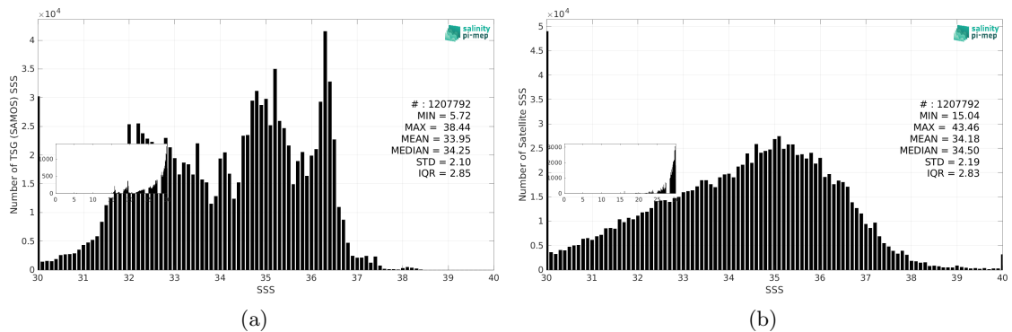
Figure 3: Histograms of SSS from TSG (SAMOS) (a) and SMAP SSS L2 v6 - 40 km (RSS) (b) considering all match-up pairs per bins of 0.1 over the Global Ocean Pi-MEP region and for the full satellite product period.
