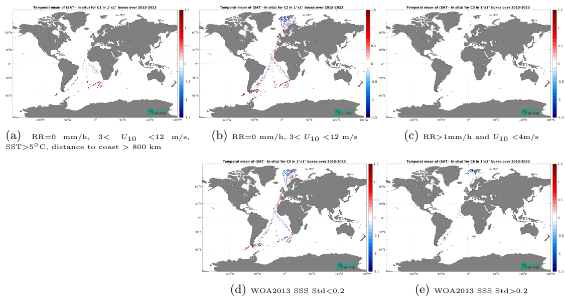
Figure 14: Temporal mean gridded over spatial boxes of size 1^\circ \times 1^\circ of \Delta\text{SSS} (SMAP SSS L2 v6 - 40 km (RSS) - TSG (Polarstern)) for 5 different subdatasets corresponding to:RR=0 mm/h, 3 < U_{10} < 12 m/s, SST > 5^\circ\text{C} , distance to coast > 800 km (a), RR=0 mm/h, 3 < U_{10} < 12 m/s (b), RR > 1 mm/h and U_{10} < 4 m/s (c), WOA2013 SSS Std < 0.2 (d), WOA2013 SSS Std > 0.2 (e).
