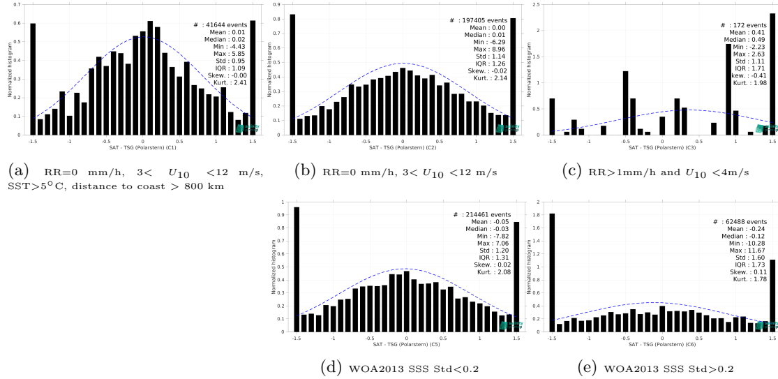
Figure 15: Normalized histogram of \Delta SSS (SMAP SSS L2 v6 - 40 km (RSS) - TSG (Polarstern)) for 5 different subdatasets corresponding to: RR=0 mm/h, 3 < U_{10} < 12 m/s, SST>5°C, distance to coast > 800 km (a), RR=0 mm/h, 3 < U_{10} < 12 m/s (b), RR>1mm/h and U_{10} < 4 m/s (c), WOA2013 SSS Std<0.2 (d), WOA2013 SSS Std>0.2 (e).
