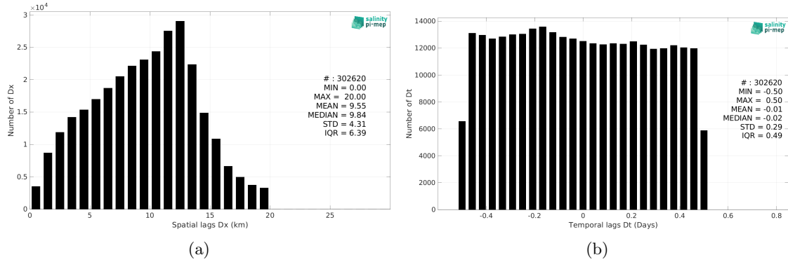
Figure 6: Histograms of the spatial (a) and temporal (b) lags between the location/time of the TSG (Polarstern) measurement and the date of the corresponding SMAP SSS L2 v6 - 40 km (RSS) SSS pixel.
