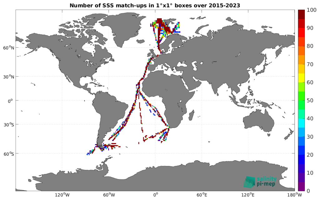
Figure 5: Number of SSS match-ups between TSG (Polarstern) SSS and the SMAP SSS L2 v6 - 40 km (RSS) SSS product for the Global Ocean Pi-MEP region over 1^\circ \times 1^\circ boxes and for the full satellite product period.
