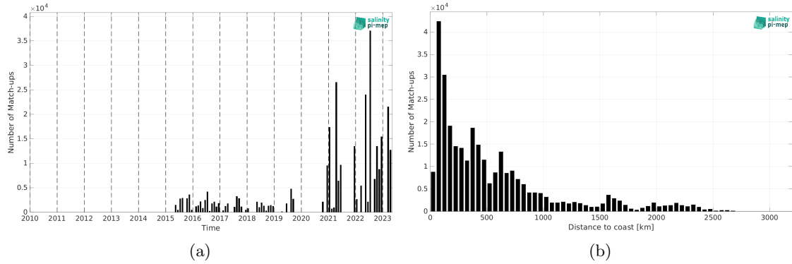
Figure 2: Number of match-ups between TSG (Polarstern) and SMAP SSS L2 v6 - 40 km (RSS) SSS as a function of time (a) and as function of the distance to coast (b) over the Global Ocean Pi-MEP region and for the full satellite product period.
