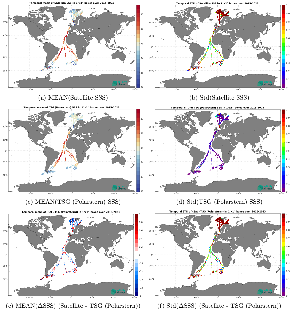
Figure 7: Temporal mean (left) and Std (right) of SSS from SMAP SSS L2 v6 - 40 km (RSS) (top), TSG (Polarstern) (middle), and of \Delta SSS (Satellite - TSG (Polarstern)). Only match-up pairs are used to generate these maps.
