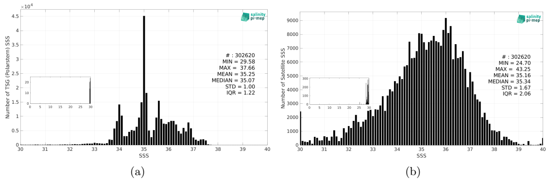
Figure 3: Histograms of SSS from TSG (Polarstern) (a) and SMAP SSS L2 v6 - 40 km (RSS) (b) considering all match-up pairs per bins of 0.1 over the Global Ocean Pi-MEP region and for the full satellite product period.
