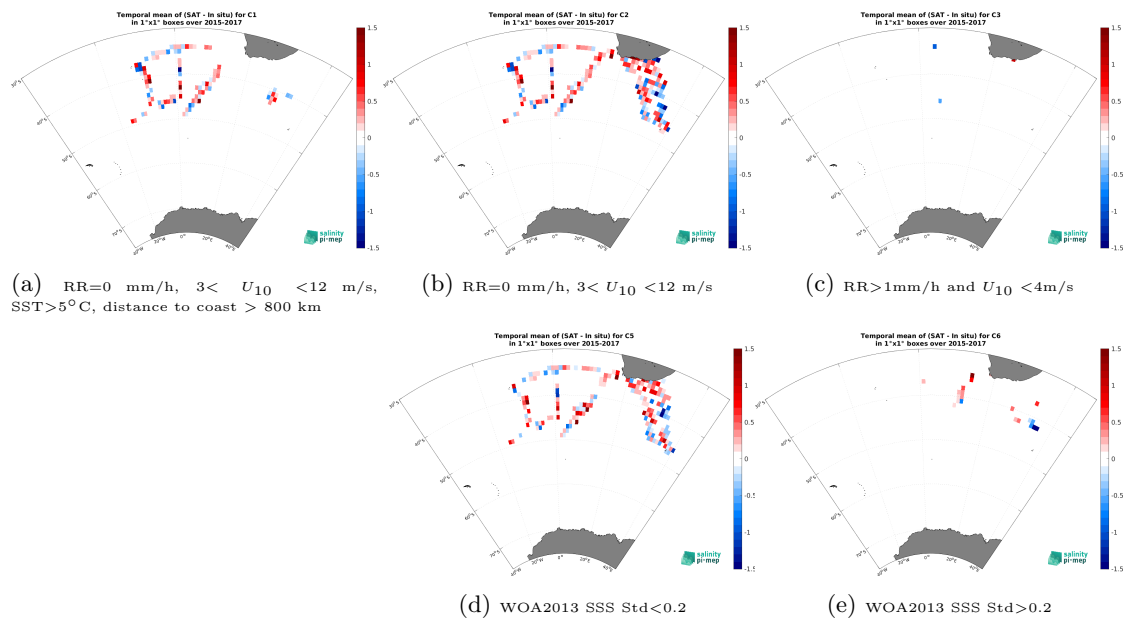
Figure 14: Temporal mean gridded over spatial boxes of size 1^\circ \times 1^\circ of \Delta SSS (SMAP SSS L2 v6 - 40 km (RSS) - TSG (NCEI-0170743)) for 5 different subdatasets corresponding to:RR=0 mm/h, 3 < U_{10} < 12 m/s, SST > 5^\circ\text{C} , distance to coast > 800 km (a), RR=0 mm/h, 3 < U_{10} < 12 m/s (b), RR > 1 mm/h and U_{10} < 4 m/s (c), WOA2013 SSS Std < 0.2 (d), WOA2013 SSS Std > 0.2 (e).
