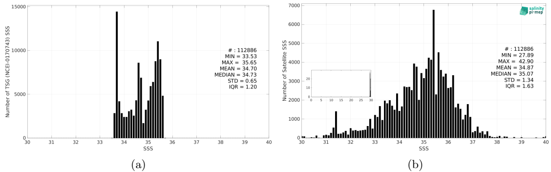
Figure 3: Histograms of SSS from TSG (NCEI-0170743) (a) and SMAP SSS L2 v6 - 40 km (RSS) (b) considering all match-up pairs per bins of 0.1 over the Global Ocean Pi-MEP region and for the full satellite product period.
