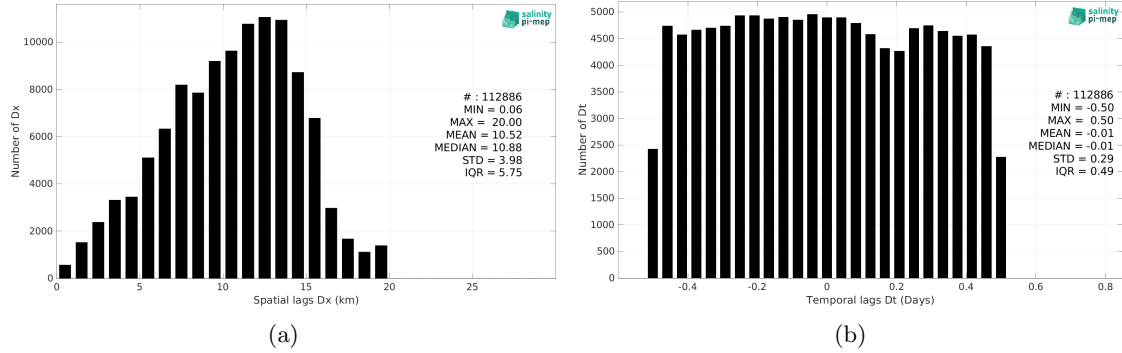
Figure 6: Histograms of the spatial (a) and temporal (b) lags between the location/time of the TSG (NCEI-0170743) measurement and the date of the corresponding SMAP SSS L2 v6 - 40 km (RSS) SSS pixel.
