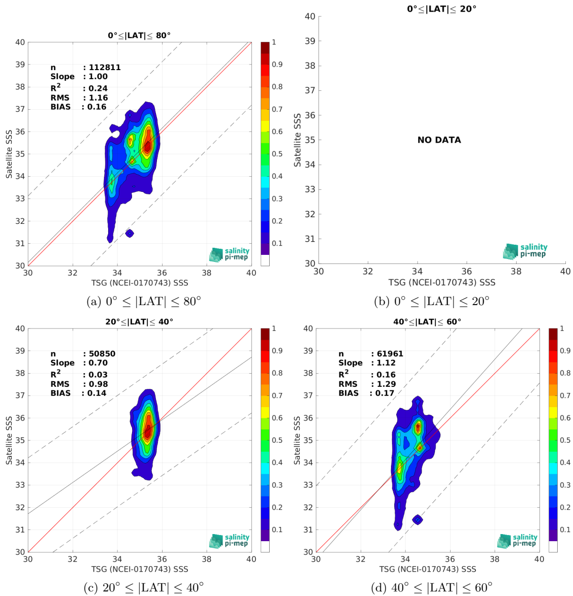
Figure 10: Contour maps of the concentration of SMAP SSS L2 v6 - 40 km (RSS) SSS (y-axis) versus TSG (NCEI-0170743) SSS (x-axis) at match-up pairs for different latitude bands. For each plot, the red line shows x=y . The black thin and dashed lines indicate a linear fit through the data cloud and the \pm 95\% confidence levels, respectively. The number match-up pairs n , the slope and R^2 coefficient of the linear fit, the root mean square (RMS) and the mean bias between satellite and in situ data are indicated for each latitude band in each plots.
