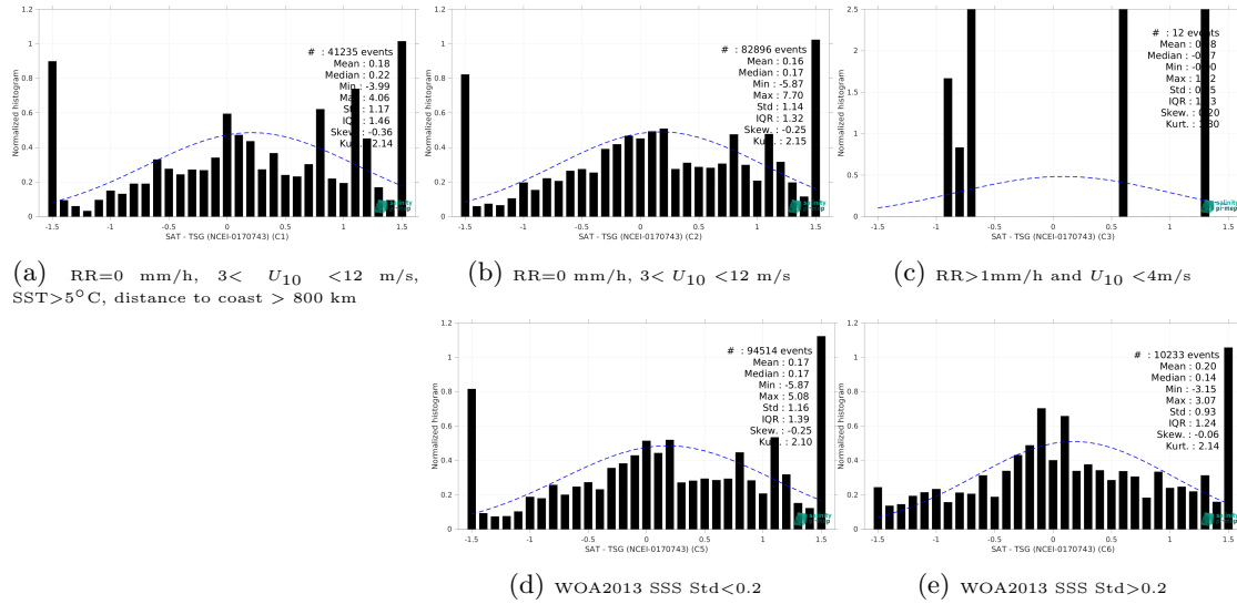
Figure 15: Normalized histogram of \Delta SSS (SMAP SSS L2 v6 - 40 km (RSS) - TSG (NCEI-0170743)) for 5 different subdatasets corresponding to: RR=0 mm/h, 3 < U_{10} < 12 m/s, SST > 5°C, distance to coast > 800 km (a), RR=0 mm/h, 3 < U_{10} < 12 m/s (b), RR > 1mm/h and U_{10} < 4 m/s (c), WOA2013 SSS Std < 0.2 (d), WOA2013 SSS Std > 0.2 (e).
