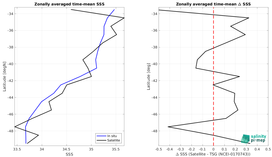
Figure 9: Left panel: Zonal mean SSS from SMAP SSS L2 v6 - 40 km (RSS) satellite product (black) and from TSG (NCEI-0170743) (blue). Right panel: Zonal mean of \Delta SSS (Satellite - TSG (NCEI-0170743)) for all the collected Pi-MEP match-up pairs estimated over the full satellite product period.
