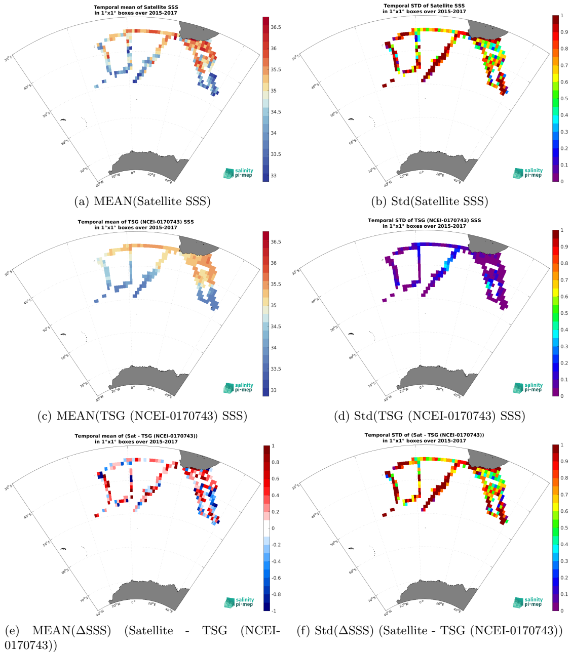
Figure 7: Temporal mean (left) and Std (right) of SSS from SMAP SSS L2 v6 - 40 km (RSS) (top), TSG (NCEI-0170743) (middle), and of \Delta SSS (Satellite - TSG (NCEI-0170743)). Only match-up pairs are used to generate these maps.
