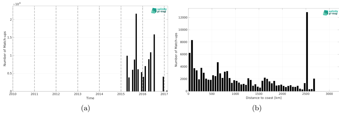
Figure 2: Number of match-ups between TSG (NCEI-0170743) and SMAP SSS L2 v6 - 40 km (RSS) SSS as a function of time (a) and as function of the distance to coast (b) over the Global Ocean Pi-MEP region and for the full satellite product period.
