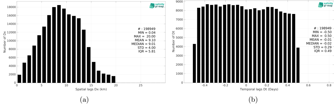
Figure 6: Histograms of the spatial (a) and temporal (b) lags between the location/time of the TSG (LEGOS-Survostral) measurement and the date of the corresponding SMAP SSS L2 v6 - 40 km (RSS) SSS pixel.
