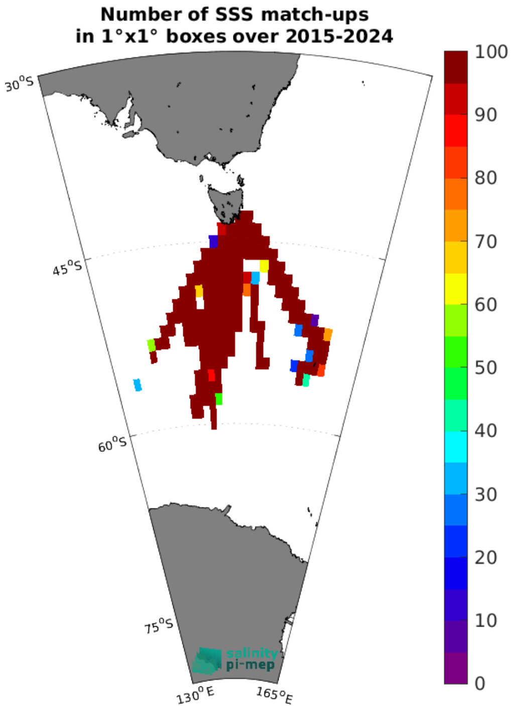
Figure 5: Number of SSS match-ups between TSG (LEGOS-Survostral) SSS and the SMAP SSS L2 v6 - 40 km (RSS) SSS product for the Global Ocean Pi-MEP region over 1°x1° boxes and for the full satellite product period.
