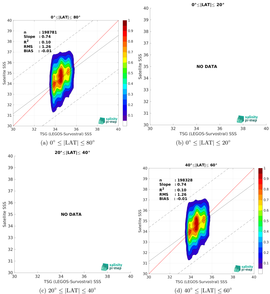
Figure 10: Contour maps of the concentration of SMAP SSS L2 v6 - 40 km (RSS) SSS (y-axis) versus TSG (LEGOS-Survostral) SSS (x-axis) at match-up pairs for different latitude bands. For each plot, the red line shows x=y . The black thin and dashed lines indicate a linear fit through the data cloud and the \pm 95\% confidence levels, respectively. The number match-up pairs n , the slope and R^2 coefficient of the linear fit, the root mean square (RMS) and the mean bias between satellite and in situ data are indicated for each latitude band in each plots.
