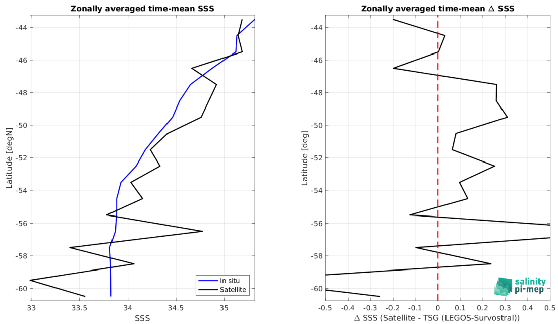
Figure 9: Left panel: Zonal mean SSS from SMAP SSS L2 v6 - 40 km (RSS) satellite product (black) and from TSG (LEGOS-Survostral) (blue). Right panel: Zonal mean of \Delta SSS (Satellite - TSG (LEGOS-Survostral)) for all the collected Pi-MEP match-up pairs estimated over the full satellite product period.
