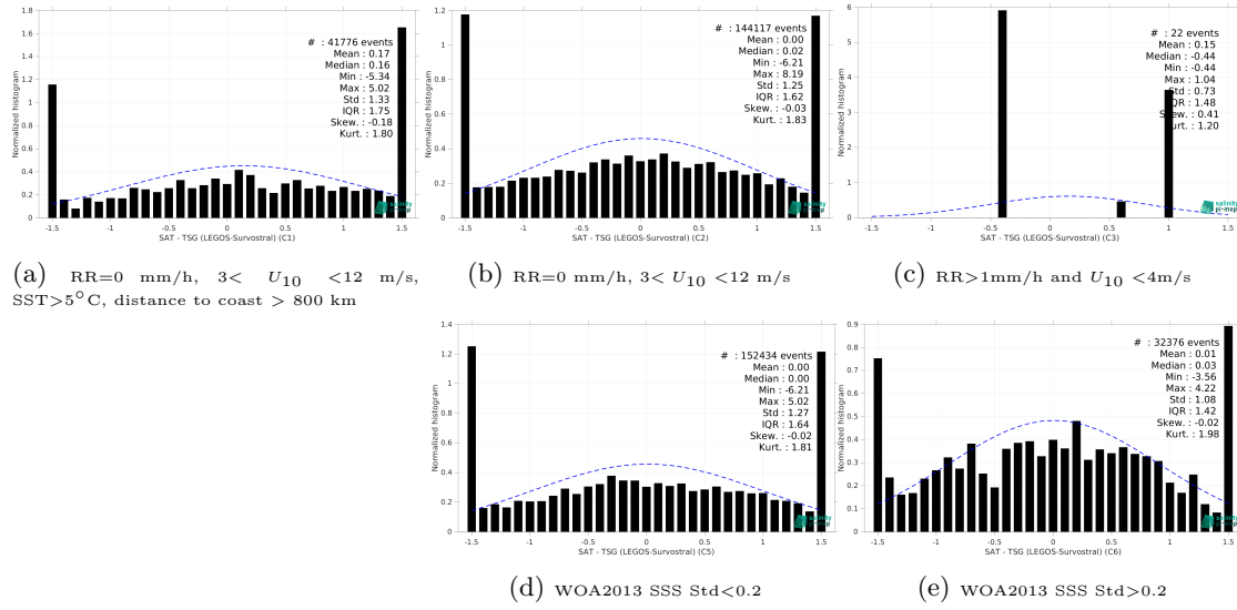
Figure 15: Normalized histogram of \Delta SSS (SMAP SSS L2 v6 - 40 km (RSS) - TSG (LEGOS-Survostral)) for 5 different subdatasets corresponding to: RR=0 mm/h, 3 < U_{10} < 12 m/s, SST > 5°C, distance to coast > 800 km (a), RR=0 mm/h, 3 < U_{10} < 12 m/s (b), RR > 1mm/h and U_{10} < 4 m/s (c), WOA2013 SSS Std < 0.2 (d), WOA2013 SSS Std > 0.2 (e).
