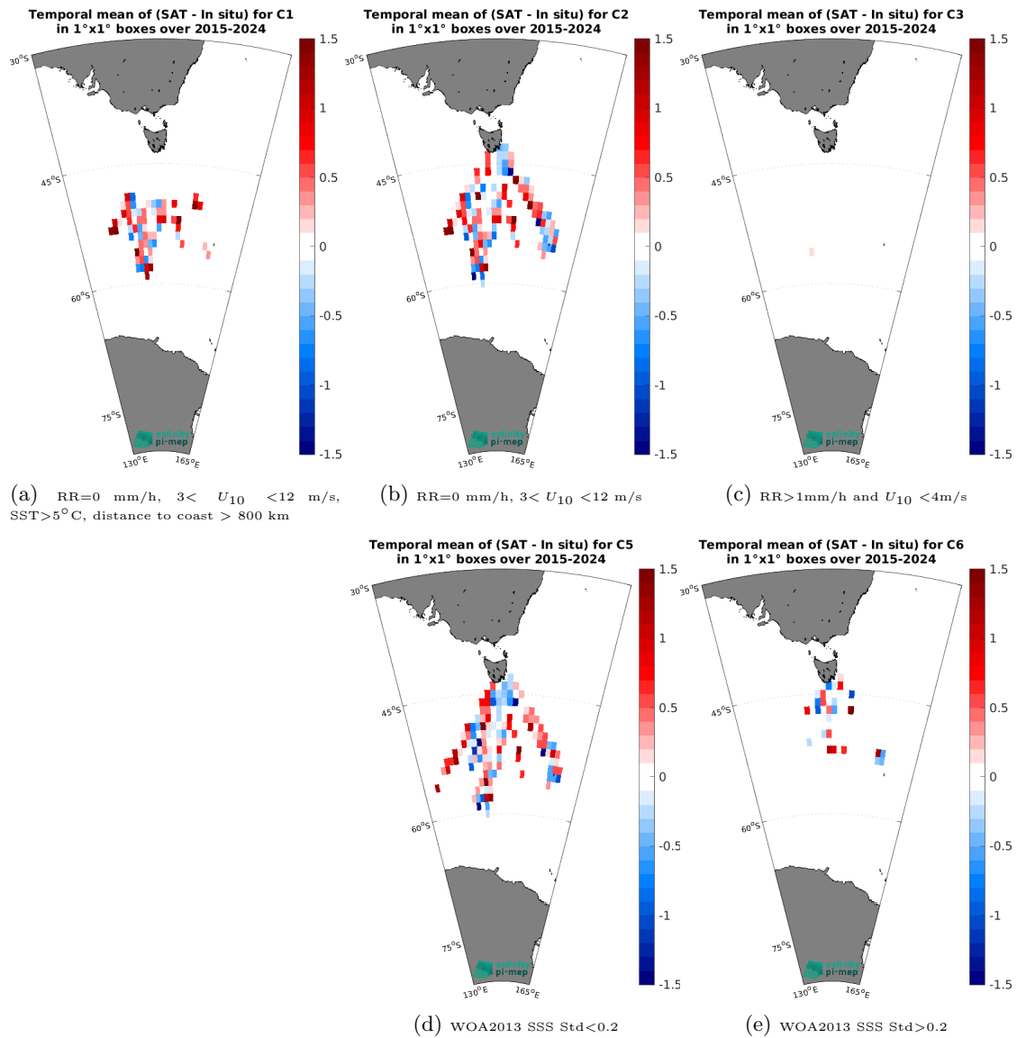
Figure 14: Temporal mean gridded over spatial boxes of size 1°x1° of \Delta SSS (SMAP SSS L2 v6 - 40 km (RSS) - TSG (LEGOS-Survostral)) for 5 different subdatasets corresponding to:RR=0 mm/h, 3 < U_{10} < 12 m/s, SST>5°C, distance to coast > 800 km (a), RR=0 mm/h, 3 < U_{10} < 12 m/s (b), RR>1mm/h and U_{10} < 4 m/s (c), WOA2013 SSS Std<0.2 (d), WOA2013 SSS Std>0.2 (e).
