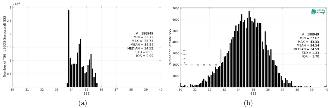
Figure 3: Histograms of SSS from TSG (LEGOS-Survostral) (a) and SMAP SSS L2 v6 - 40 km (RSS) (b) considering all match-up pairs per bins of 0.1 over the Global Ocean Pi-MEP region and for the full satellite product period.
