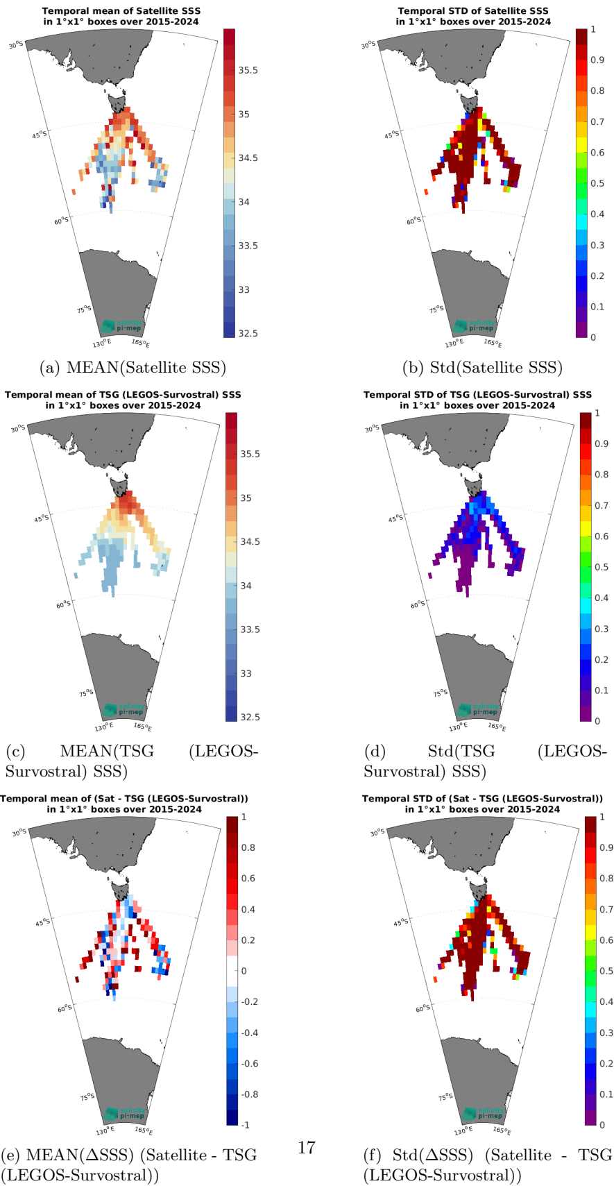
Figure 7: Temporal mean (left) and Std (right) of SSS from SMAP SSS L2 v6 - 40 km (RSS) (top), TSG (LEGOS-Survostral) (middle), and of \Delta SSS (Satellite - TSG (LEGOS-Survostral)). Only match-up pairs are used to generate these maps.
