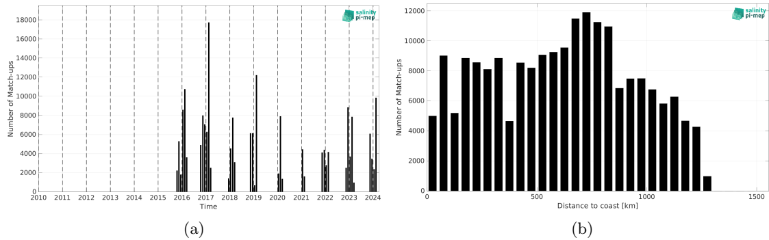
Figure 2: Number of match-ups between TSG (LEGOS-Survostral) and SMAP SSS L2 v6 - 40 km (RSS) SSS as a function of time (a) and as function of the distance to coast (b) over the Global Ocean Pi-MEP region and for the full satellite product period.
