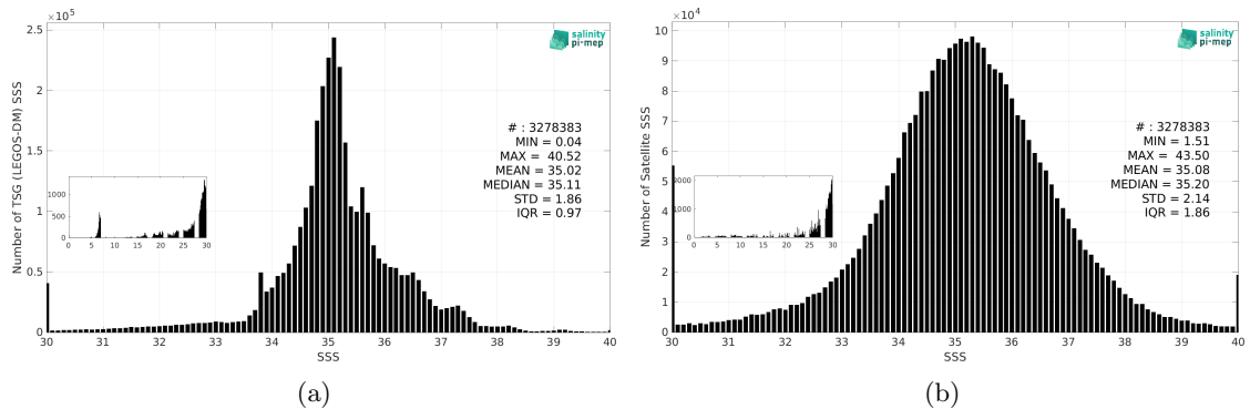
Figure 3: Histograms of SSS from TSG (LEGOS-DM) (a) and SMAP SSS L2 v6 - 40 km (RSS) (b) considering all match-up pairs per bins of 0.1 over the Global Ocean Pi-MEP region and for the full satellite product period.
