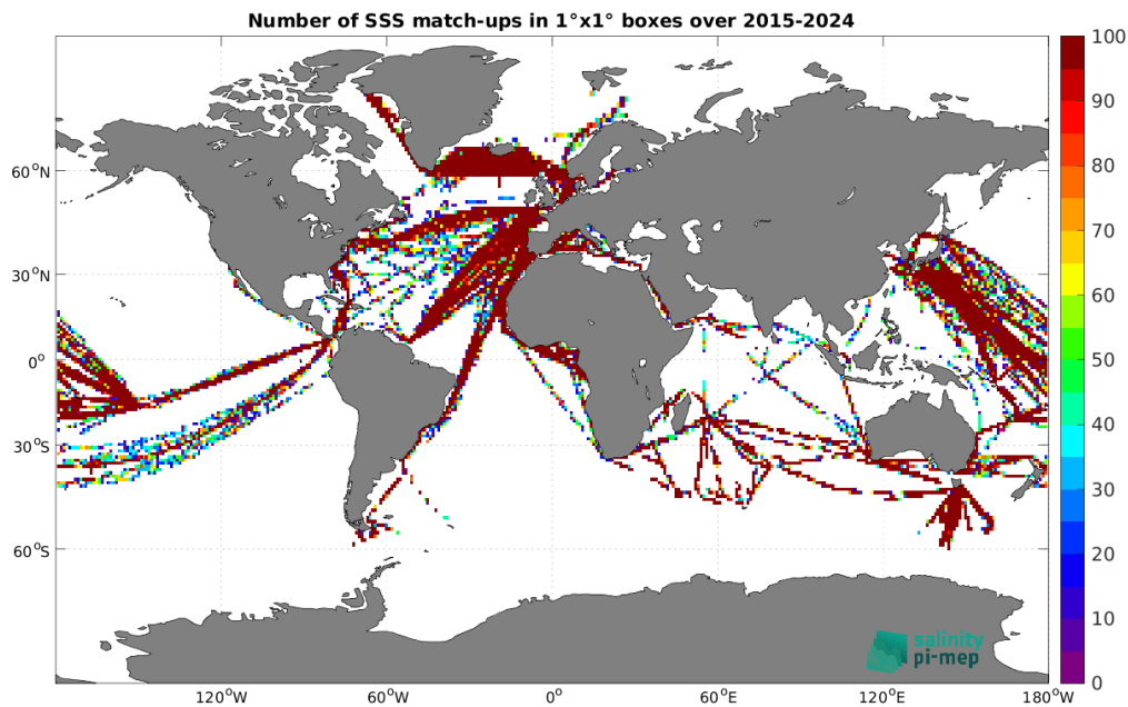
Figure 5: Number of SSS match-ups between TSG (LEGOS-DM) SSS and the SMAP SSS L2 v6 - 40 km (RSS) SSS product for the Global Ocean Pi-MEP region over 1^\circ \times 1^\circ boxes and for the full satellite product period.
