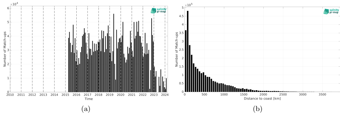
Figure 2: Number of match-ups between TSG (LEGOS-DM) and SMAP SSS L2 v6 - 40 km (RSS) SSS as a function of time (a) and as function of the distance to coast (b) over the Global Ocean Pi-MEP region and for the full satellite product period.
