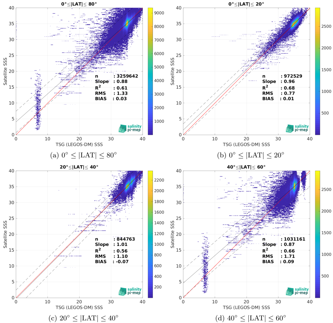
Figure 10: Contour maps of the concentration of SMAP SSS L2 v6 - 40 km (RSS) SSS (y-axis) versus TSG (LEGOS-DM) SSS (x-axis) at match-up pairs for different latitude bands. For each plot, the red line shows x=y . The black thin and dashed lines indicate a linear fit through the data cloud and the \pm 95\% confidence levels, respectively. The number match-up pairs n , the slope and R^2 coefficient of the linear fit, the root mean square (RMS) and the mean bias between satellite and in situ data are indicated for each latitude band in each plots.
