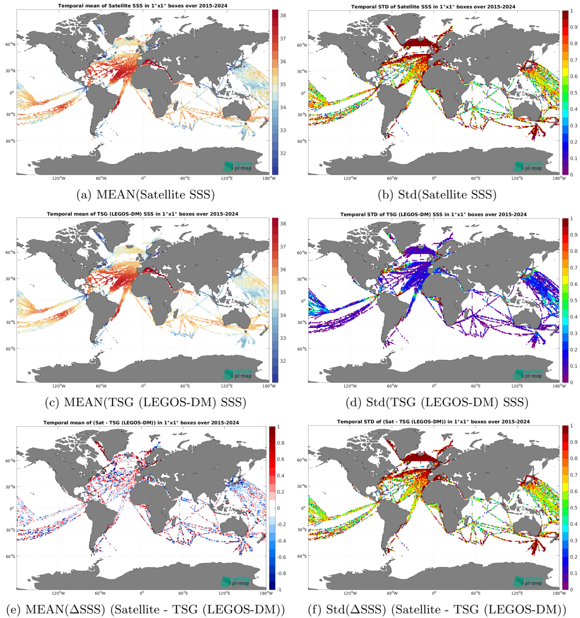
Figure 7: Temporal mean (left) and Std (right) of SSS from SMAP SSS L2 v6 - 40 km (RSS) (top), TSG (LEGOS-DM) (middle), and of \Delta SSS (Satellite - TSG (LEGOS-DM)). Only match-pair are used to generate these maps.
