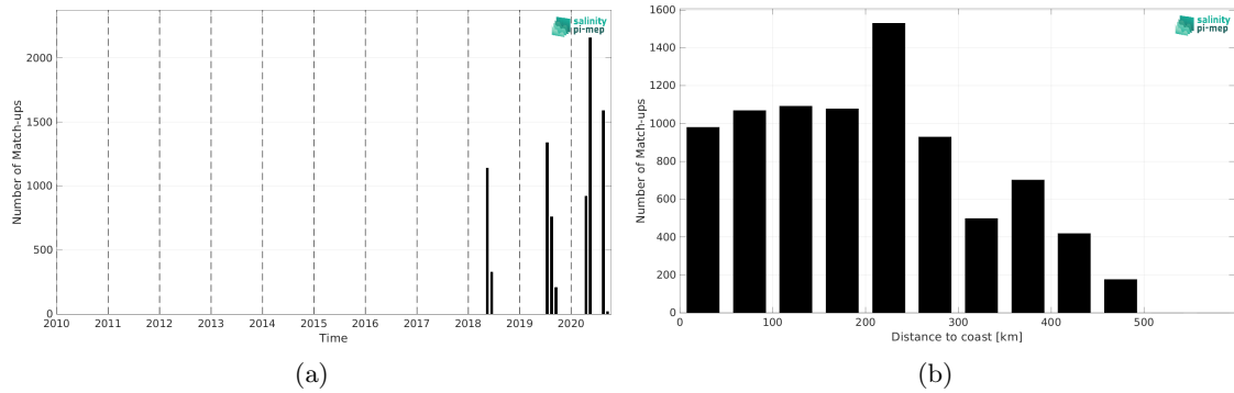
Figure 2: Number of match-ups between TSG (Lauge-Koch) and SMAP SSS L2 v6 - 40 km (RSS) SSS as a function of time (a) and as function of the distance to coast (b) over the Global Ocean Pi-MEP region and for the full satellite product period.
