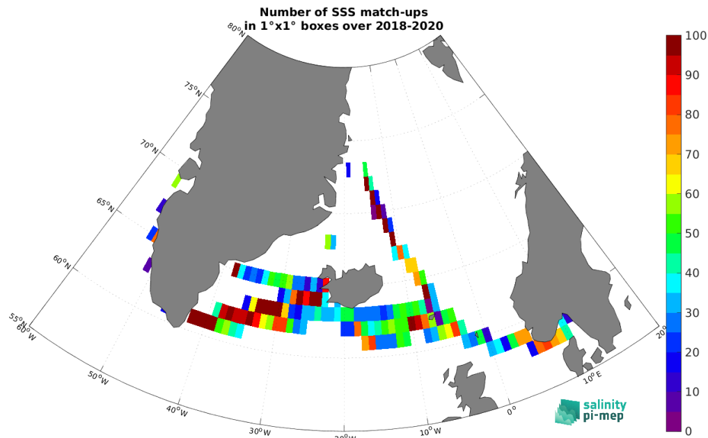
Figure 5: Number of SSS match-ups between TSG (Lauge-Koch) SSS and the SMAP SSS L2 v6 - 40 km (RSS) SSS product for the Global Ocean Pi-MEP region over 1^\circ \times 1^\circ boxes and for the full satellite product period.
