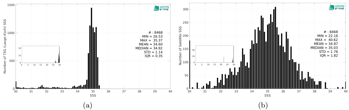
Figure 3: Histograms of SSS from TSG (Lauge-Koch) (a) and SMAP SSS L2 v6 - 40 km (RSS) (b) considering all match-up pairs per bins of 0.1 over the Global Ocean Pi-MEP region and for the full satellite product period.
