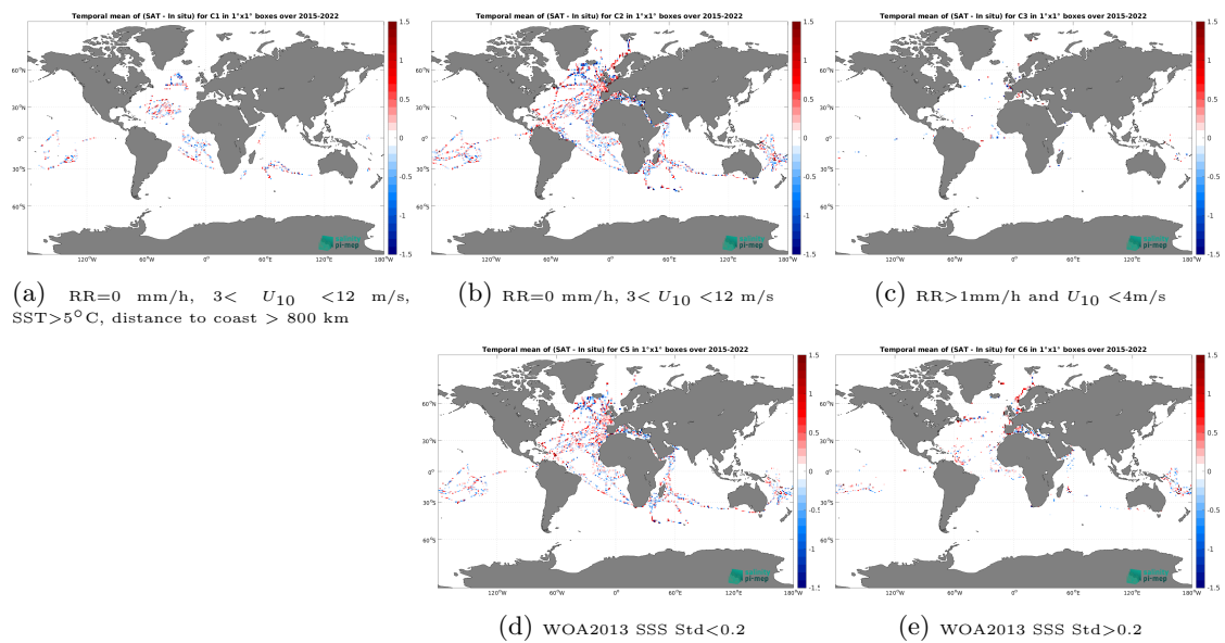
Figure 14: Temporal mean gridded over spatial boxes of size 1^\circ \times 1^\circ of \Delta SSS (SMAP SSS L2 v6 - 40 km (RSS) - TSG (GOSUD-Research-vessel)) for 5 different subdatasets corresponding to: RR=0 mm/h, 3 < U_{10} < 12 m/s, SST > 5^\circ\text{C} , distance to coast > 800 km (a), RR=0 mm/h, 3 < U_{10} < 12 m/s (b), RR > 1 mm/h and U_{10} < 4 m/s (c), WOA2013 SSS Std < 0.2 (d), WOA2013 SSS Std > 0.2 (e).
