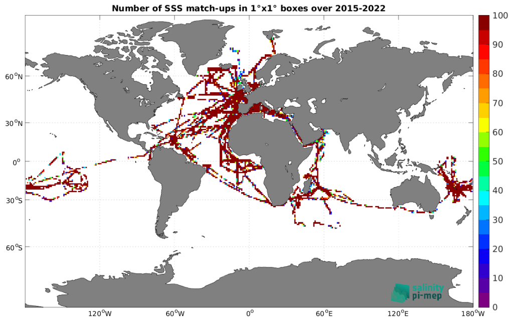
Figure 5: Number of SSS match-ups between TSG (GOSUD-Research-vessel) SSS and the SMAP SSS L2 v6 - 40 km (RSS) SSS product for the Global Ocean Pi-MEP region over 1^\circ \times 1^\circ boxes and for the full satellite product period.
