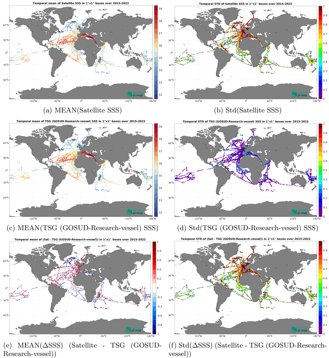
Figure 7: Temporal mean (left) and Std (right) of SSS from SMAP SSS L2 v6 - 40 km (RSS) (top), TSG (GOSUD-Research-vessel) (middle), and of \Delta SSS (Satellite - TSG (GOSUD-Research-vessel)). Only match-up pairs are used to generate these maps.
