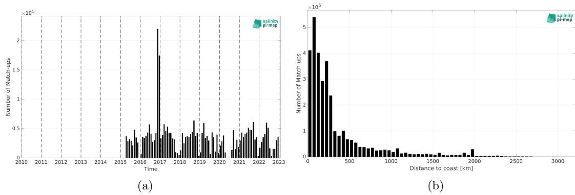
Figure 2: Number of match-ups between TSG (GOSUD-Research-vessel) and SMAP SSS L2 v6 - 40 km (RSS) SSS as a function of time (a) and as function of the distance to coast (b) over the Global Ocean Pi-MEP region and for the full satellite product period.
