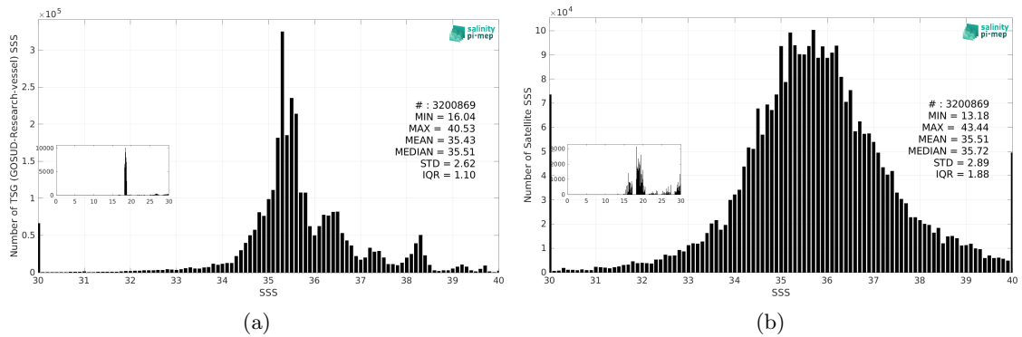
Figure 3: Histograms of SSS from TSG (GOSUD-Research-vessel) (a) and SMAP SSS L2 v6 - 40 km (RSS) (b) considering all match-up pairs per bins of 0.1 over the Global Ocean Pi-MEP region and for the full satellite product period.
