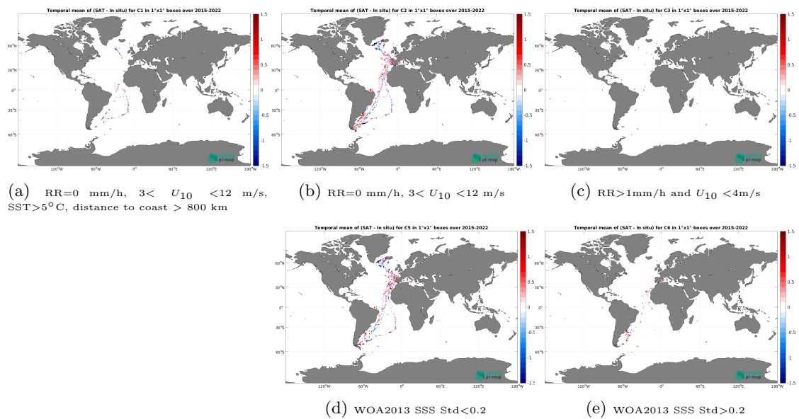
Figure 14: Temporal mean gridded over spatial boxes of size 1^\circ \times 1^\circ of \Delta\text{SSS} (SMAP SSS L2 v6 - 40 km (RSS) - TSG (CSIC-UTM)) for 5 different subdatasets corresponding to:RR=0 mm/h, 3 < U_{10} < 12 m/s, SST > 5^\circ\text{C} , distance to coast > 800 km (a), RR=0 mm/h, 3 < U_{10} < 12 m/s (b), RR > 1 mm/h and U_{10} < 4 m/s (c), WOA2013 SSS Std < 0.2 (d), WOA2013 SSS Std > 0.2 (e).
