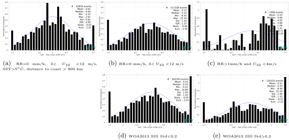
Figure 15: Normalized histogram of \Delta SSS (SMAP SSS L2 v6 - 40 km (RSS) - TSG (CSIC-UTM)) for 5 different subdatasets corresponding to: RR=0 mm/h, 3 < U_{10} < 12 m/s, SST > 5°C, distance to coast > 800 km (a), RR=0 mm/h, 3 < U_{10} < 12 m/s (b), RR > 1mm/h and U_{10} < 4 m/s (c), WOA2013 SSS Std < 0.2 (d), WOA2013 SSS Std > 0.2 (e).
