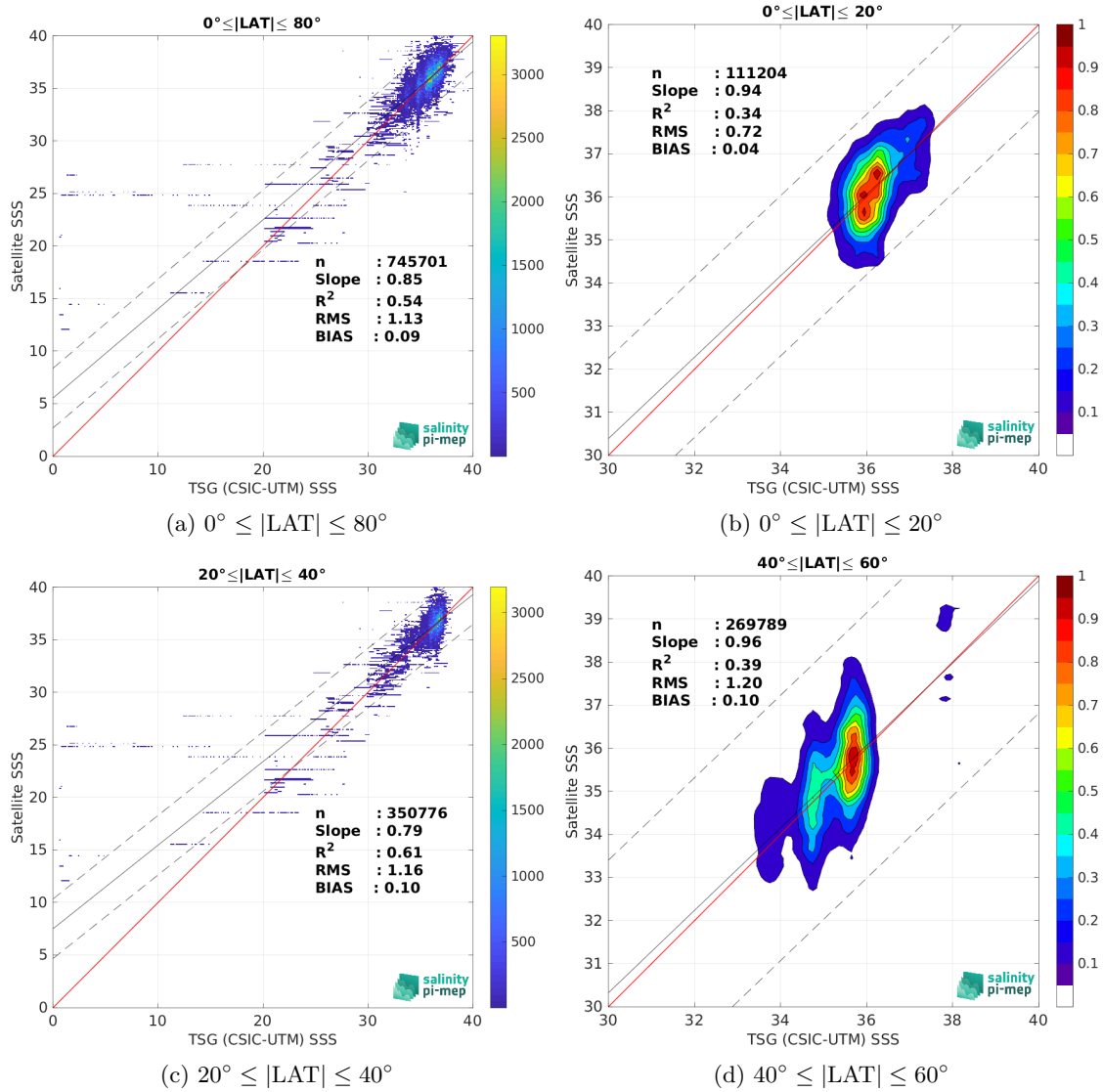
Figure 10: Contour maps of the concentration of SMAP SSS L2 v6 - 40 km (RSS) SSS (y-axis) versus TSG (CSIC-UTM) SSS (x-axis) at match-up pairs for different latitude bands. For each plot, the red line shows x=y . The black thin and dashed lines indicate a linear fit through the data cloud and the \pm 95\% confidence levels, respectively. The number match-up pairs n , the slope and R^2 coefficient of the linear fit, the root mean square (RMS) and the mean bias between satellite and in situ data are indicated for each latitude band in each plots.
