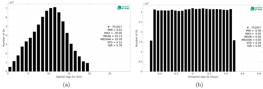
Figure 6: Histograms of the spatial (a) and temporal (b) lags between the location/time of the TSG (CSIC-UTM) measurement and the date of the corresponding SMAP SSS L2 v6 - 40 km (RSS) SSS pixel.
