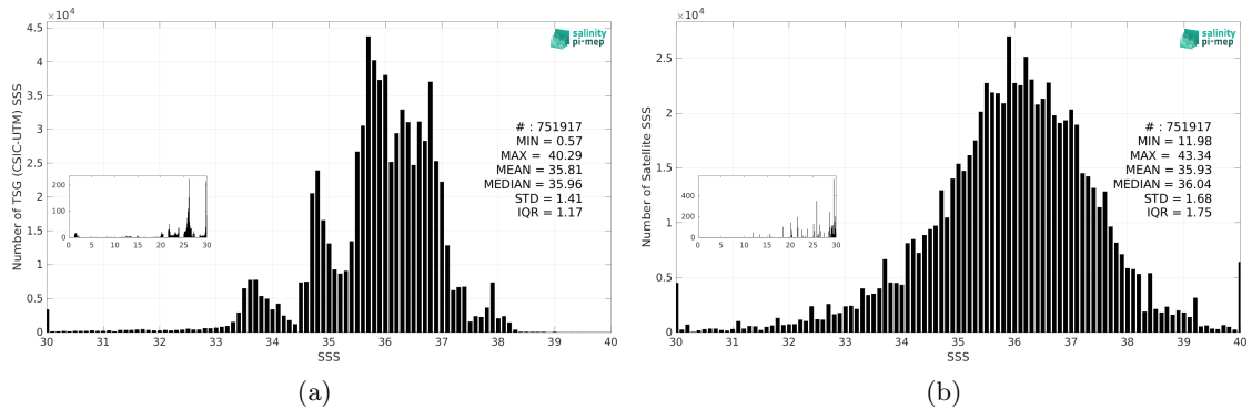
Figure 3: Histograms of SSS from TSG (CSIC-UTM) (a) and SMAP SSS L2 v6 - 40 km (RSS) (b) considering all match-up pairs per bins of 0.1 over the Global Ocean Pi-MEP region and for the full satellite product period.
