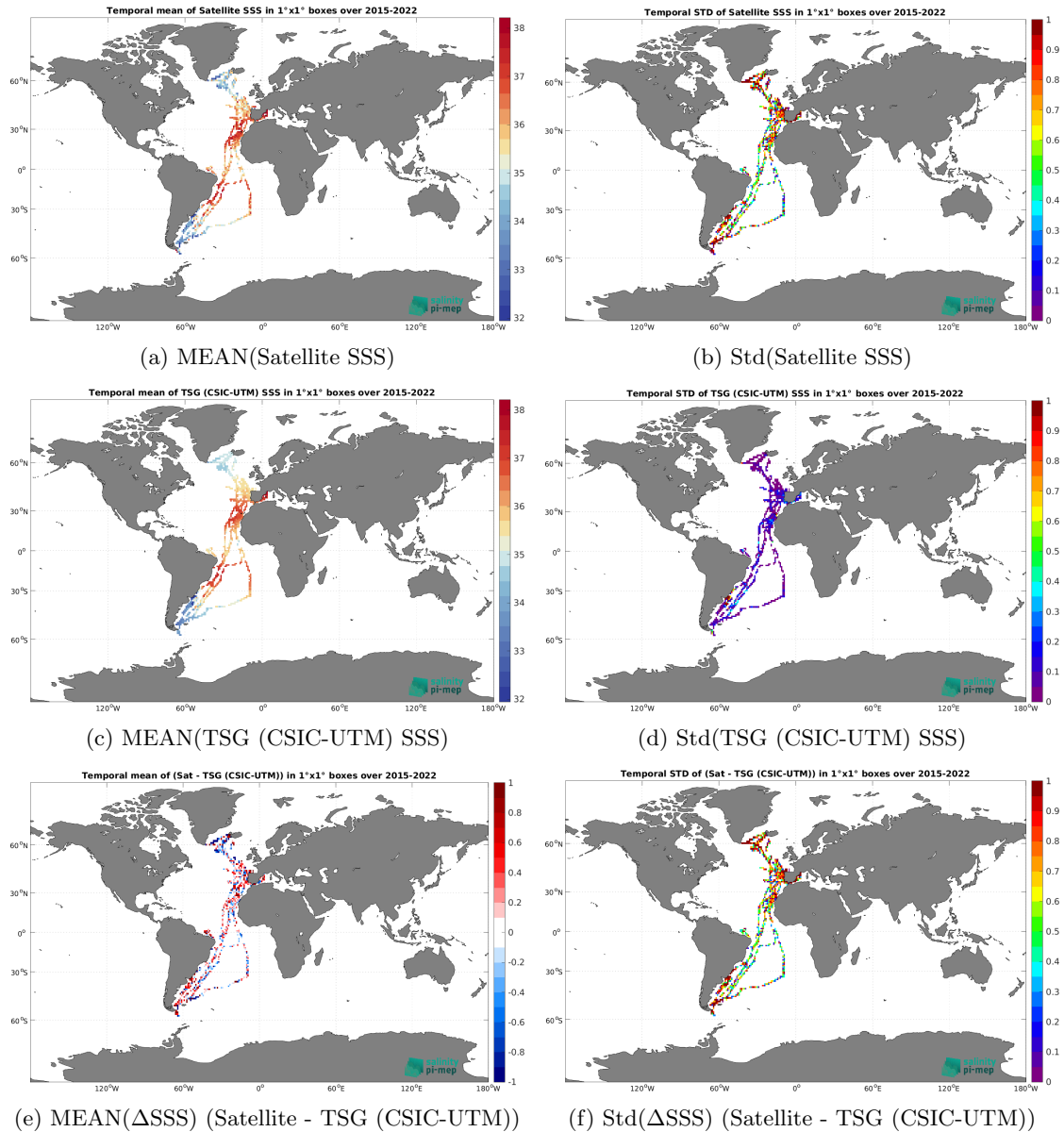
Figure 7: Temporal mean (left) and Std (right) of SSS from SMAP SSS L2 v6 - 40 km (RSS) (top), TSG (CSIC-UTM) (middle), and of \Delta SSS (Satellite - TSG (CSIC-UTM)). Only match-up pairs are used to generate these maps.
