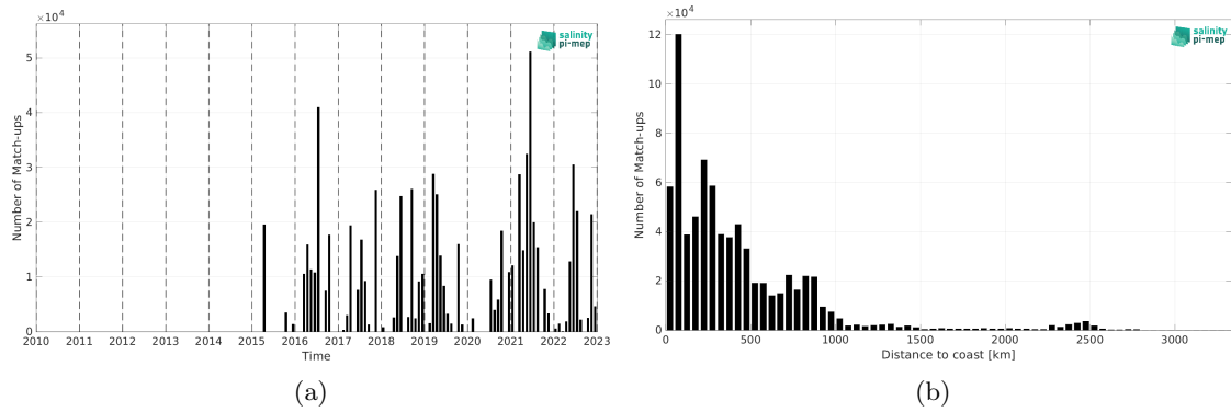
Figure 2: Number of match-ups between TSG (CSIC-UTM) and SMAP SSS L2 v6 - 40 km (RSS) SSS as a function of time (a) and as function of the distance to coast (b) over the Global Ocean Pi-MEP region and for the full satellite product period.
