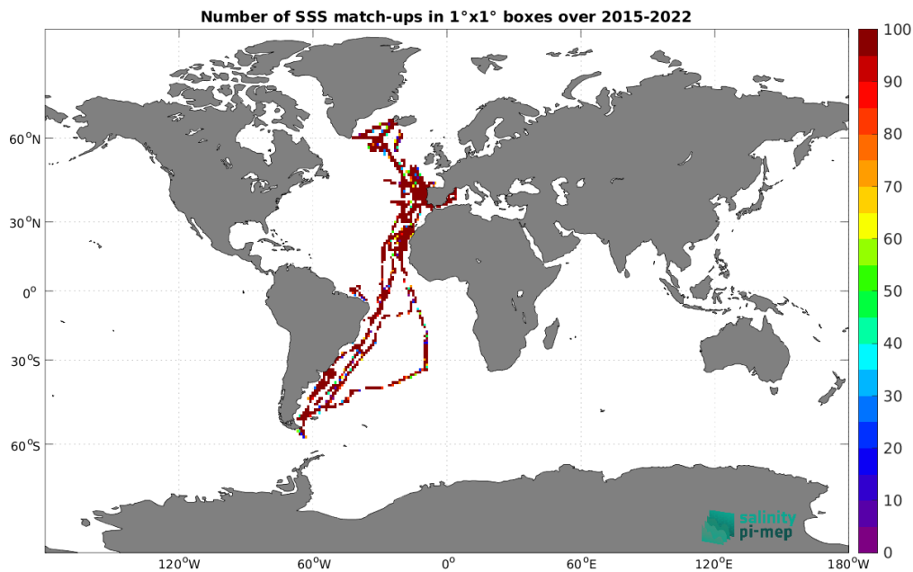
Figure 5: Number of SSS match-ups between TSG (CSIC-UTM) SSS and the SMAP SSS L2 v6 - 40 km (RSS) SSS product for the Global Ocean Pi-MEP region over 1^\circ \times 1^\circ boxes and for the full satellite product period.
