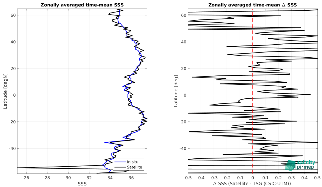
Figure 9: Left panel: Zonal mean SSS from SMAP SSS L2 v6 - 40 km (RSS) satellite product (black) and from TSG (CSIC-UTM) (blue). Right panel: Zonal mean of \Delta SSS (Satellite - TSG (CSIC-UTM)) for all the collected Pi-MEP match-up pairs estimated over the full satellite product period.
