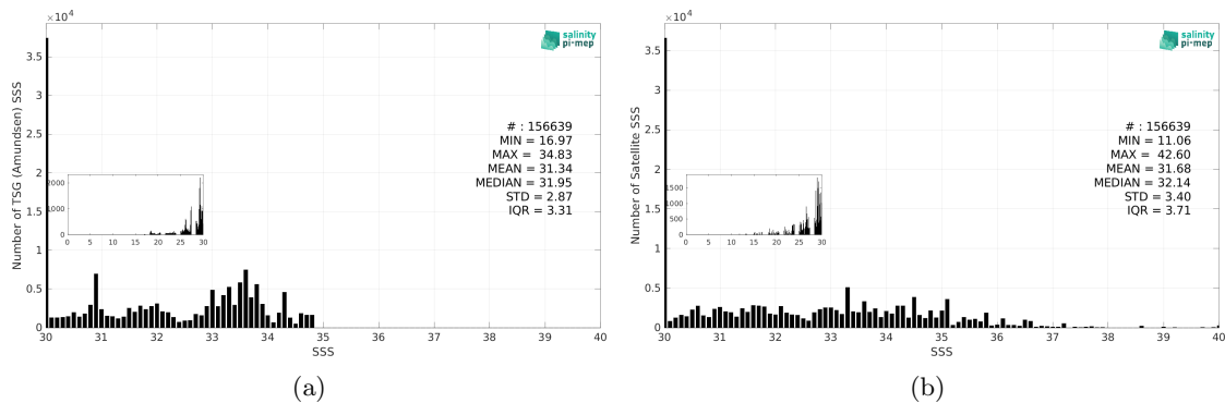
Figure 3: Histograms of SSS from TSG (Amundsen) (a) and SMAP SSS L2 v6 - 40 km (RSS) (b) considering all match-up pairs per bins of 0.1 over the Global Ocean Pi-MEP region and for the full satellite product period.
