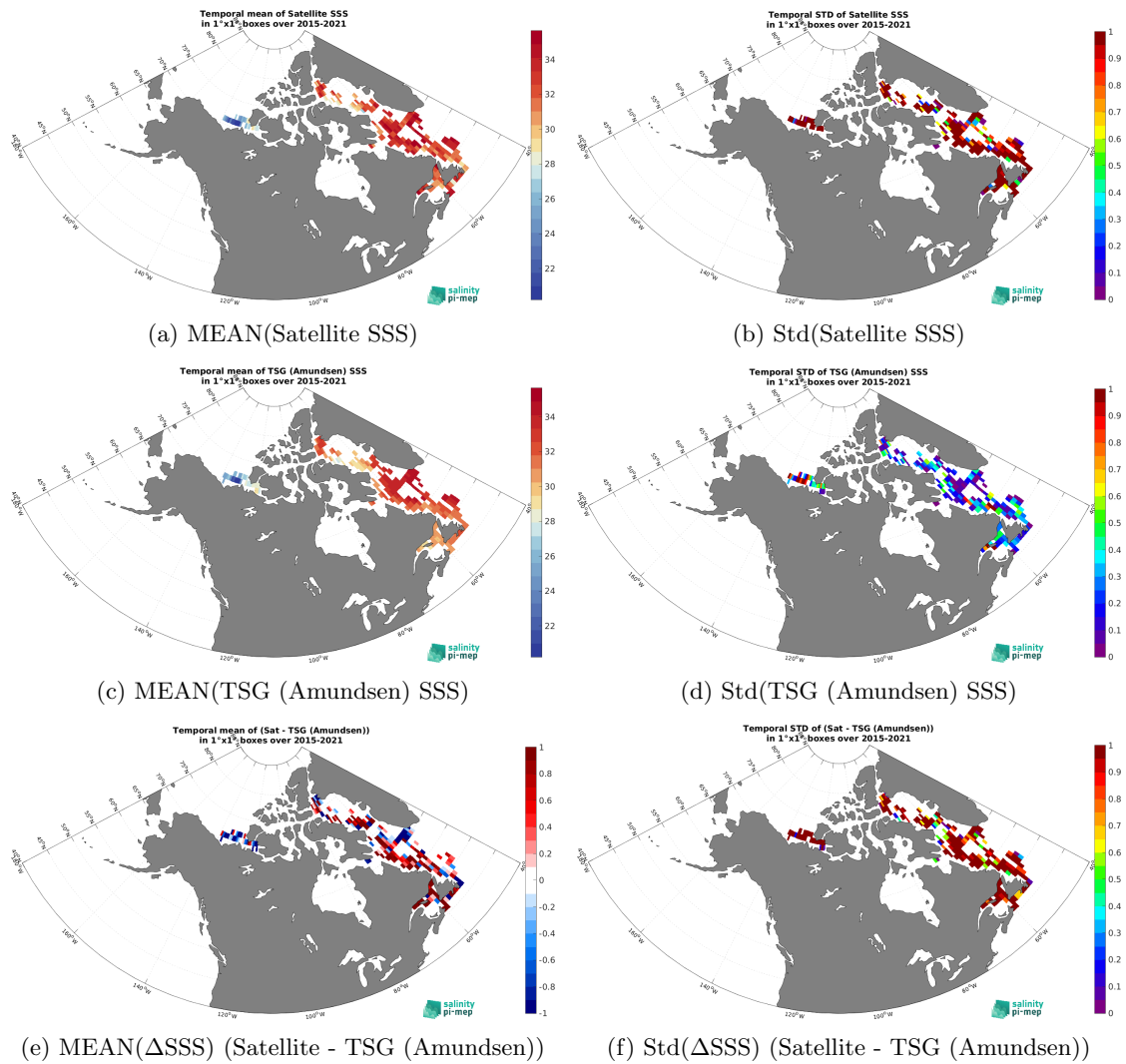
Figure 7: Temporal mean (left) and Std (right) of SSS from SMAP SSS L2 v6 - 40 km (RSS) (top), TSG (Amundsen) (middle), and of \Delta SSS (Satellite - TSG (Amundsen)). Only match-up pairs are used to generate these maps.
