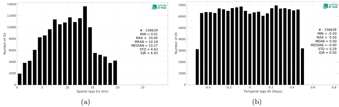
Figure 6: Histograms of the spatial (a) and temporal (b) lags between the location/time of the TSG (Amundsen) measurement and the date of the corresponding SMAP SSS L2 v6 - 40 km (RSS) SSS pixel.
