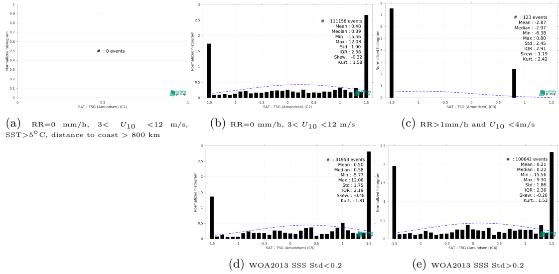
Figure 15: Normalized histogram of \Delta\text{SSS} (SMAP SSS L2 v6 - 40 km (RSS) - TSG (Amundsen)) for 5 different subdatasets corresponding to: RR=0 mm/h, 3 < U_{10} < 12 m/s, SST > 5^\circ\text{C} , distance to coast > 800 km (a), RR=0 mm/h, 3 < U_{10} < 12 m/s (b), RR > 1\text{mm/h} and U_{10} < 4\text{m/s} (c), WOA2013 SSS \text{Std} < 0.2 (d), WOA2013 SSS \text{Std} > 0.2 (e).
