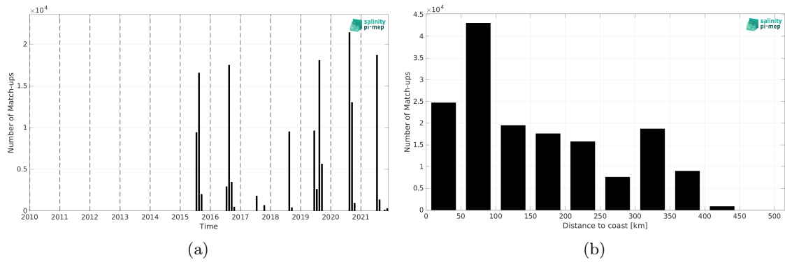
Figure 2: Number of match-ups between TSG (Amundsen) and SMAP SSS L2 v6 - 40 km (RSS) SSS as a function of time (a) and as function of the distance to coast (b) over the Global Ocean Pi-MEP region and for the full satellite product period.
