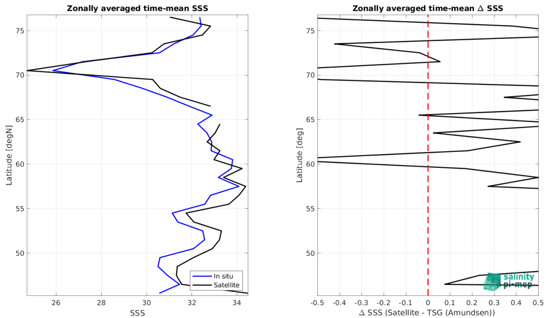
Figure 9: Left panel: Zonal mean SSS from SMAP SSS L2 v6 - 40 km (RSS) satellite product (black) and from TSG (Amundsen) (blue). Right panel: Zonal mean of \Delta SSS (Satellite - TSG (Amundsen)) for all the collected Pi-MEP match-up pairs estimated over the full satellite product period.
