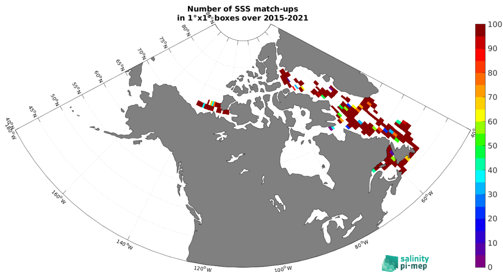
Figure 5: Number of SSS match-ups between TSG (Amundsen) SSS and the SMAP SSS L2 v6 - 40 km (RSS) SSS product for the Global Ocean Pi-MEP region over 1^\circ \times 1^\circ boxes and for the full satellite product period.
