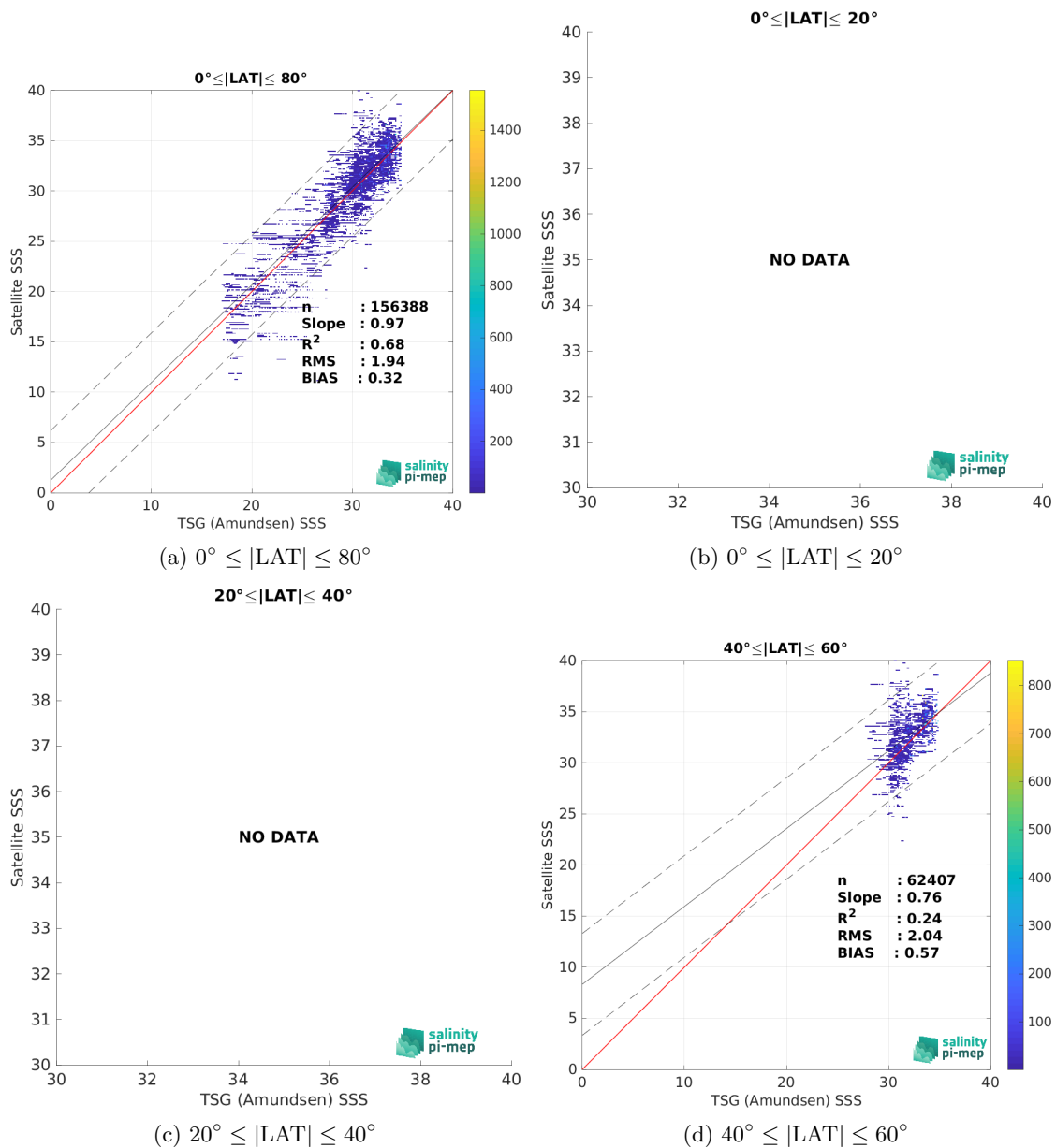
Figure 10: Contour maps of the concentration of SMAP SSS L2 v6 - 40 km (RSS) SSS (y-axis) versus TSG (Amundsen) SSS (x-axis) at match-up pairs for different latitude bands. For each plot, the red line shows x=y . The black thin and dashed lines indicate a linear fit through the data cloud and the \pm 95\% confidence levels, respectively. The number match-up pairs n , the slope and R^2 coefficient of the linear fit, the root mean square (RMS) and the mean bias between satellite and in situ data are indicated for each latitude band in each plots.
