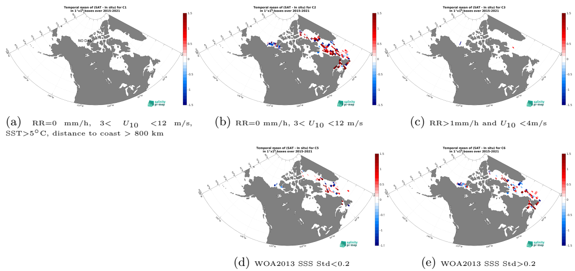
Figure 14: Temporal mean gridded over spatial boxes of size 1^\circ \times 1^\circ of \Delta SSS (SMAP SSS L2 v6 - 40 km (RSS) - TSG (Amundsen)) for 5 different subdatasets corresponding to:RR=0 mm/h, 3 < U_{10} < 12 m/s, SST > 5°C, distance to coast > 800 km (a), RR=0 mm/h, 3 < U_{10} < 12 m/s (b), RR > 1mm/h and U_{10} < 4 m/s (c), WOA2013 SSS Std < 0.2 (d), WOA2013 SSS Std > 0.2 (e).
