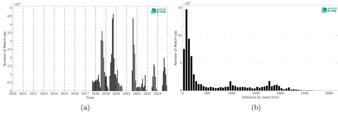
Figure 2: Number of match-ups between Saildrone and SMAP SSS L2 v6 - 40 km (RSS) SSS as a function of time (a) and as function of the distance to coast (b) over the Global Ocean Pi-MEP region and for the full satellite product period.
