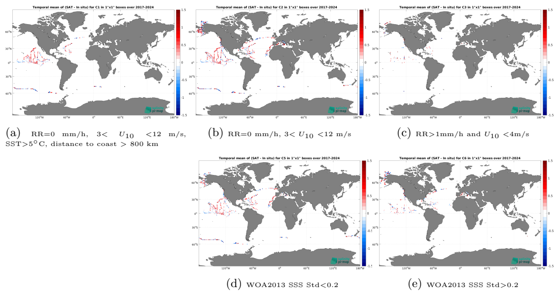
Figure 14: Temporal mean gridded over spatial boxes of size 1^\circ \times 1^\circ of \Delta SSS (SMAP SSS L2 v6 - 40 km (RSS) - Saildrone) for 5 different subdatasets corresponding to:RR=0 mm/h, 3 < U_{10} < 12 m/s, SST > 5^\circ\text{C} , distance to coast > 800 km (a), RR=0 mm/h, 3 < U_{10} < 12 m/s (b), RR > 1 mm/h and U_{10} < 4 m/s (c), WOA2013 SSS Std < 0.2 (d), WOA2013 SSS Std > 0.2 (e).
