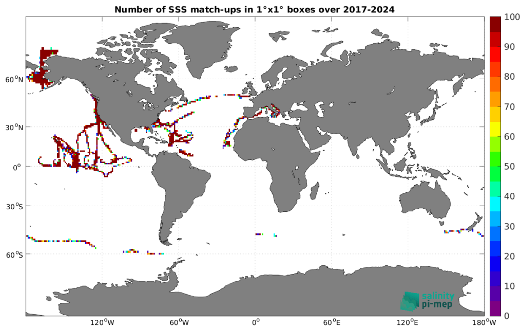
Figure 5: Number of SSS match-ups between Saildrone SSS and the SMAP SSS L2 v6 - 40 km (RSS) SSS product for the Global Ocean Pi-MEP region over 1^\circ \times 1^\circ boxes and for the full satellite product period.
