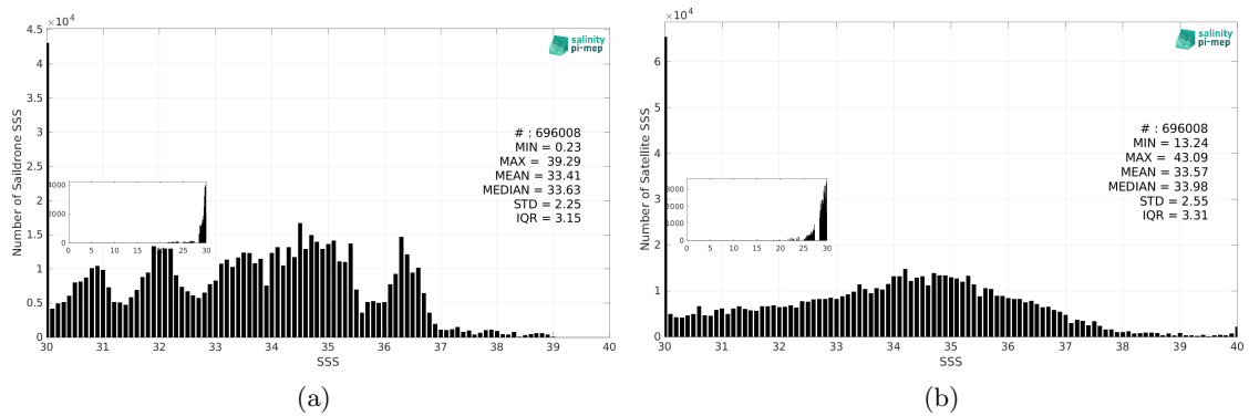
Figure 3: Histograms of SSS from Saildrone (a) and SMAP SSS L2 v6 - 40 km (RSS) (b) considering all match-up pairs per bins of 0.1 over the Global Ocean Pi-MEP region and for the full satellite product period.
