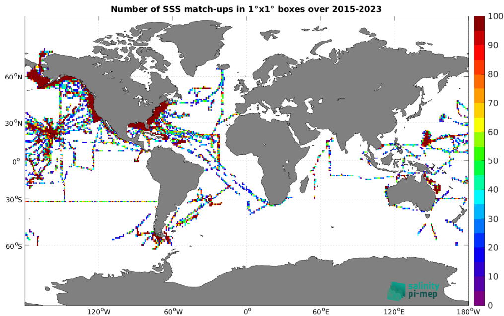
Figure 4: Number of SSS match-ups between TSG (SAMOS) SSS and the SMAP SSS L2 v5 (RSS) SSS product for the Global Ocean Pi-MEP region over 1^\circ \times 1^\circ boxes and for the full satellite product period.
