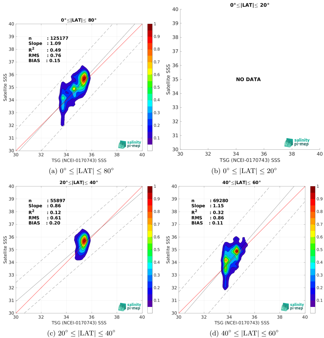
Figure 9: Contour maps of the concentration of SMAP SSS L2 v5 (RSS) SSS (y-axis) versus TSG (NCEI-0170743) SSS (x-axis) at match-up pairs for different latitude bands. For each plot, the red line shows x=y . The black thin and dashed lines indicate a linear fit through the data cloud and the \pm 95\% confidence levels, respectively. The number match-up pairs n , the slope and R^2 coefficient of the linear fit, the root mean square (RMS) and the mean bias between satellite and in situ data are indicated for each latitude band in each plots.
