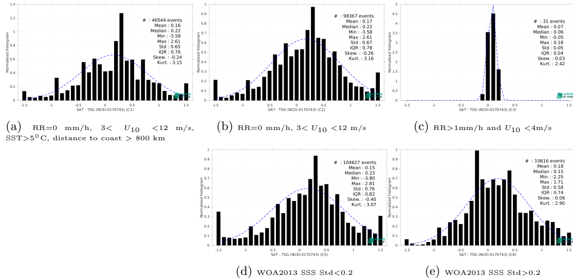
Figure 13: Normalized histogram of \Delta SSS (SMAP SSS L2 v5 (RSS) - TSG (NCEI-0170743)) for 5 different subdatasets corresponding to: RR=0 mm/h, 3 < U_{10} < 12 m/s, SST > 5°C, distance to coast > 800 km (a), RR=0 mm/h, 3 < U_{10} < 12 m/s (b), RR > 1mm/h and U_{10} < 4 m/s (c), WOA2013 SSS Std < 0.2 (d), WOA2013 SSS Std > 0.2 (e).
