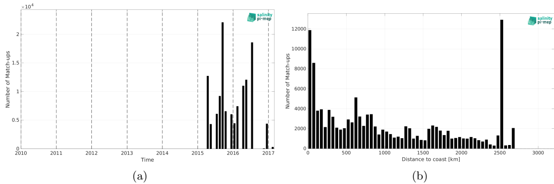
Figure 1: Number of match-ups between TSG (NCEI-0170743) and SMAP SSS L2 v5 (RSS) SSS as a function of time (a) and as function of the distance to coast (b) over the Global Ocean Pi-MEP region and for the full satellite product period.
