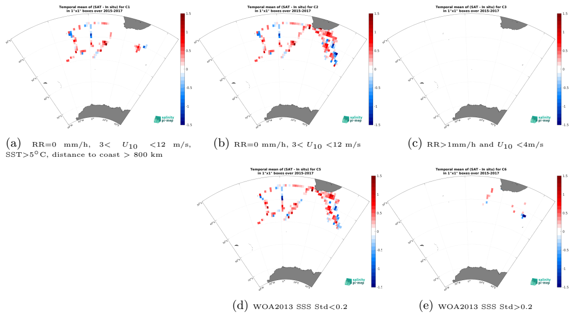
Figure 12: Temporal mean gridded over spatial boxes of size 1^\circ \times 1^\circ of \Delta SSS (SMAP SSS L2 v5 (RSS) - TSG (NCEI-0170743)) for 5 different subdatasets corresponding to:RR=0 mm/h, 3 < U_{10} < 12 m/s, SST >5^\circ C, distance to coast > 800 km (a), RR=0 mm/h, 3 < U_{10} < 12 m/s (b), RR >1 mm/h and U_{10} < 4 m/s (c), WOA2013 SSS Std <0.2 (d), WOA2013 SSS Std >0.2 (e).
