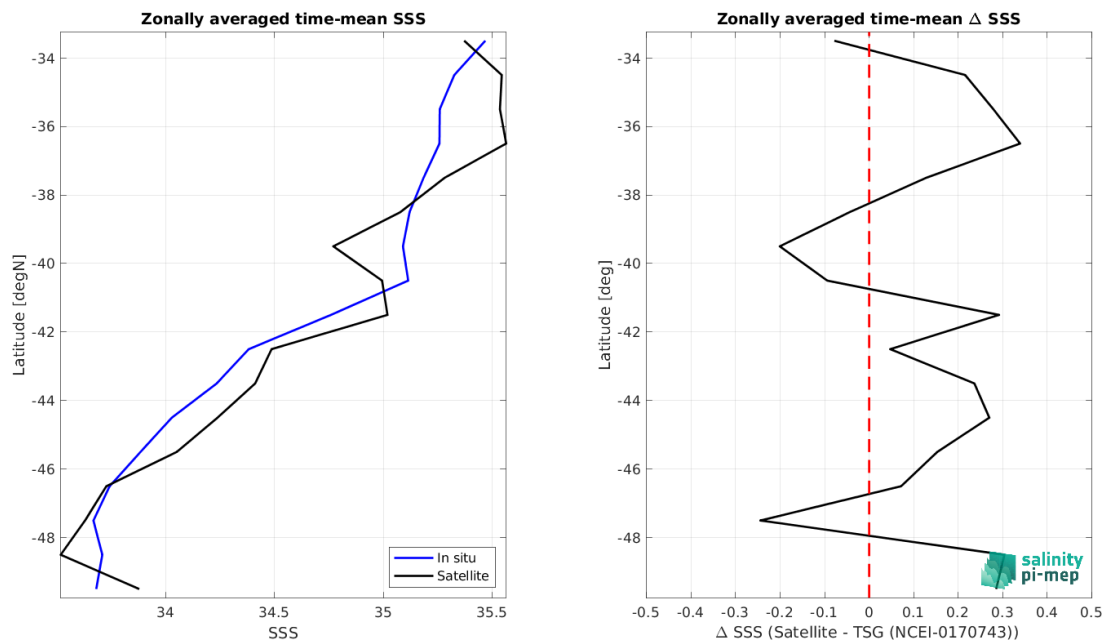
Figure 8: Left panel: Zonal mean SSS from SMAP SSS L2 v5 (RSS) satellite product (black) and from TSG (NCEI-0170743) (blue). Right panel: Zonal mean of \Delta SSS (Satellite - TSG (NCEI-0170743)) for all the collected Pi-MEP match-up pairs estimated over the full satellite product period.
