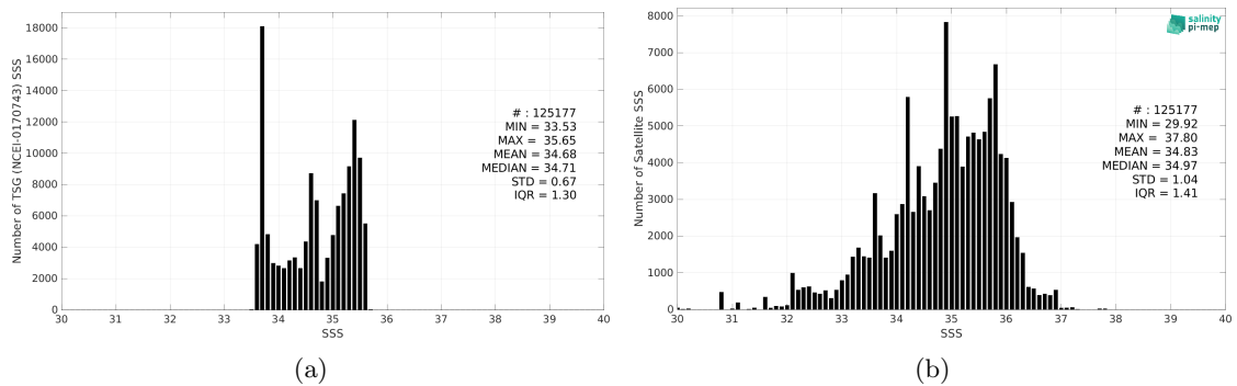
Figure 2: Histograms of SSS from TSG (NCEI-0170743) (a) and SMAP SSS L2 v5 (RSS) (b) considering all match-up pairs per bins of 0.1 over the Global Ocean Pi-MEP region and for the full satellite product period.
