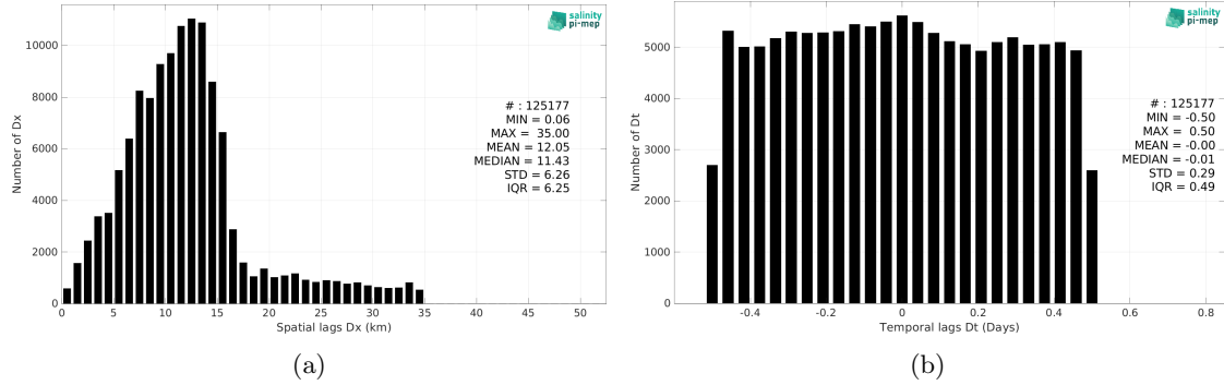
Figure 5: Histograms of the spatial (a) and temporal (b) lags between the location/time of the TSG (NCEI-0170743) measurement and the date of the corresponding SMAP SSS L2 v5 (RSS) SSS pixel.
