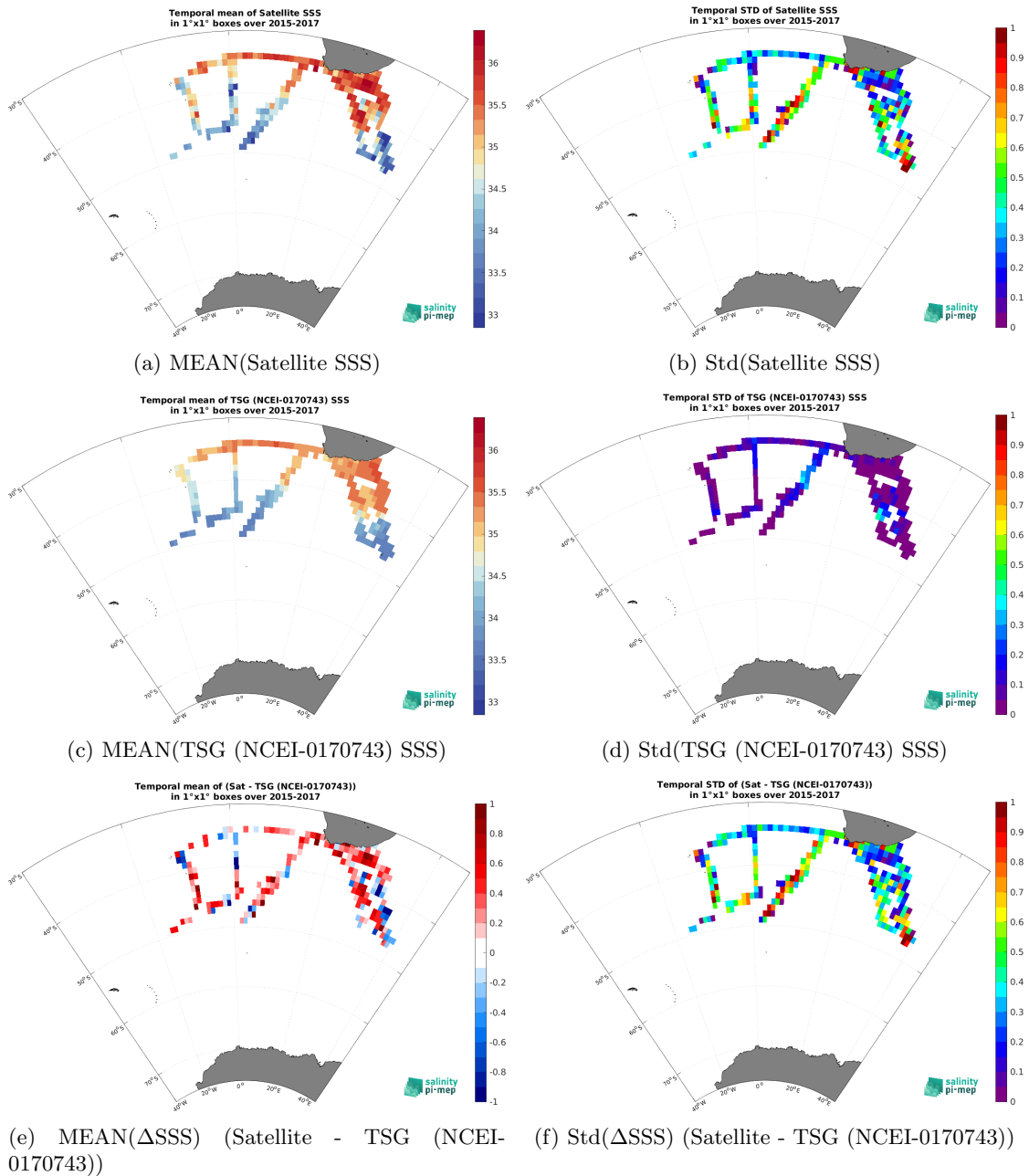
Figure 6: Temporal mean (left) and Std (right) of SSS from SMAP SSS L2 v5 (RSS) (top), TSG (NCEI-0170743) (middle), and of \Delta SSS (Satellite - TSG (NCEI-0170743)). Only match-up pairs are used to generate these maps.
