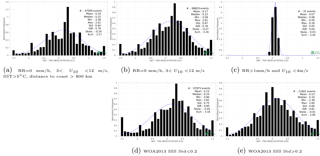
Figure 13: Normalized histogram of \Delta SSS (SMAP SSS L2 v5 (RSS) - TSG (NCEI-0170743)) for 5 different subdatasets corresponding to: RR=0 mm/h, 3 < U_{10} < 12 m/s, SST>5°C, distance to coast > 800 km (a), RR=0 mm/h, 3 < U_{10} < 12 m/s (b), RR>1mm/h and U_{10} < 4 m/s (c), WOA2013 SSS Std<0.2 (d), WOA2013 SSS Std>0.2 (e).
