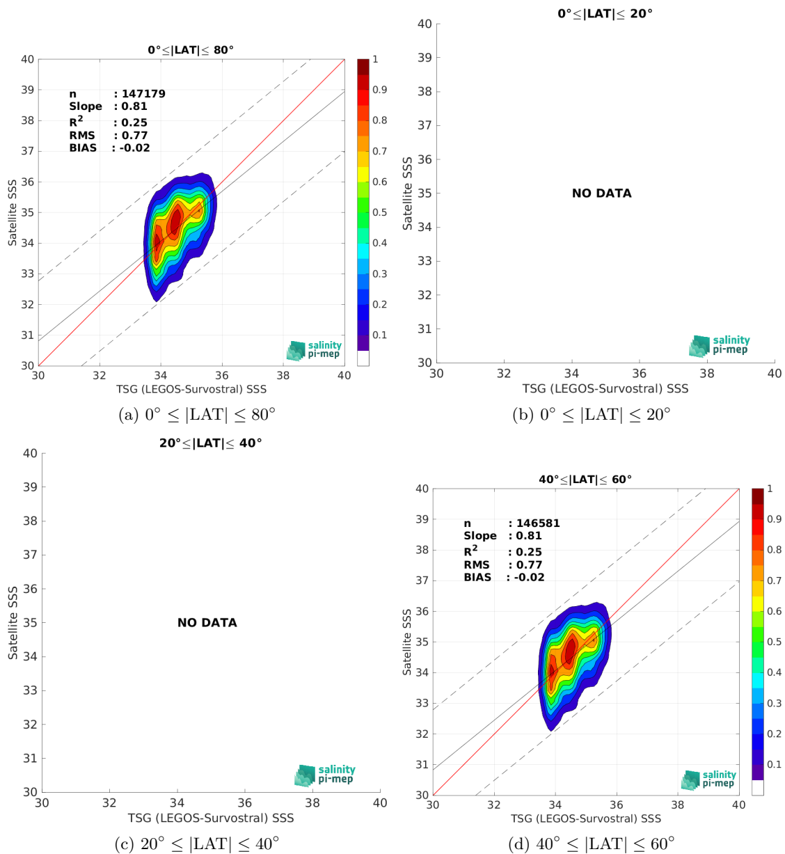
Figure 9: Contour maps of the concentration of SMAP SSS L2 v5 (RSS) SSS (y-axis) versus TSG (LEGOS-Survostral) SSS (x-axis) at match-up pairs for different latitude bands. For each plot, the red line shows x=y . The black thin and dashed lines indicate a linear fit through the data cloud and the \pm 95\% confidence levels, respectively. The number match-up pairs n , the slope and R^2 coefficient of the linear fit, the root mean square (RMS) and the mean bias between satellite and in situ data are indicated for each latitude band in each plot.
