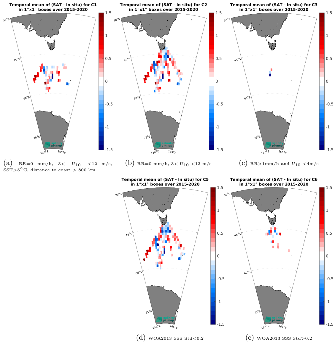
Figure 12: Temporal mean gridded over spatial boxes of size 1°x1° of \Delta SSS (SMAP SSS L2 v5 (RSS) - TSG (LEGOS-Survostral)) for 5 different subdatasets corresponding to:RR=0 mm/h, 3 < U_{10} < 12 m/s, SST>5°C, distance to coast > 800 km (a), RR=0 mm/h, 3 < U_{10} < 12 m/s (b), RR>1mm/h and U_{10} < 4 m/s (c), WOA2013 SSS Std<0.2 (d), WOA2013 SSS Std>0.2 (e).
