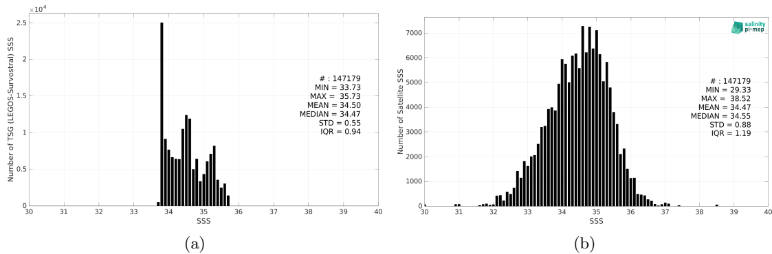
Figure 2: Histograms of SSS from TSG (LEGOS-Survostral) (a) and SMAP SSS L2 v5 (RSS) (b) considering all match-up pairs per bins of 0.1 over the Global Ocean Pi-MEP region and for the full satellite product period.
