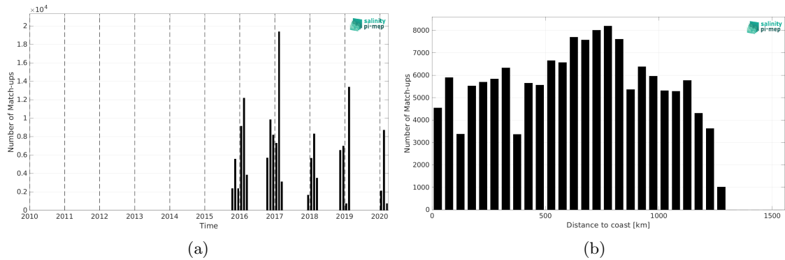
Figure 1: Number of match-ups between TSG (LEGOS-Survostral) and SMAP SSS L2 v5 (RSS) SSS as a function of time (a) and as function of the distance to coast (b) over the Global Ocean Pi-MEP region and for the full satellite product period.
