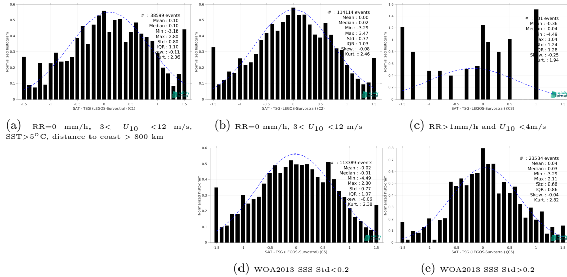
Figure 13: Normalized histogram of \Delta SSS (SMAP SSS L2 v5 (RSS) - TSG (LEGOS-Survostral)) for 5 different subdatasets corresponding to: RR=0 mm/h, 3 < U_{10} < 12 m/s, SST > 5°C, distance to coast > 800 km (a), RR=0 mm/h, 3 < U_{10} < 12 m/s (b), RR > 1mm/h and U_{10} < 4 m/s (c), WOA2013 SSS Std < 0.2 (d), WOA2013 SSS Std > 0.2 (e).
