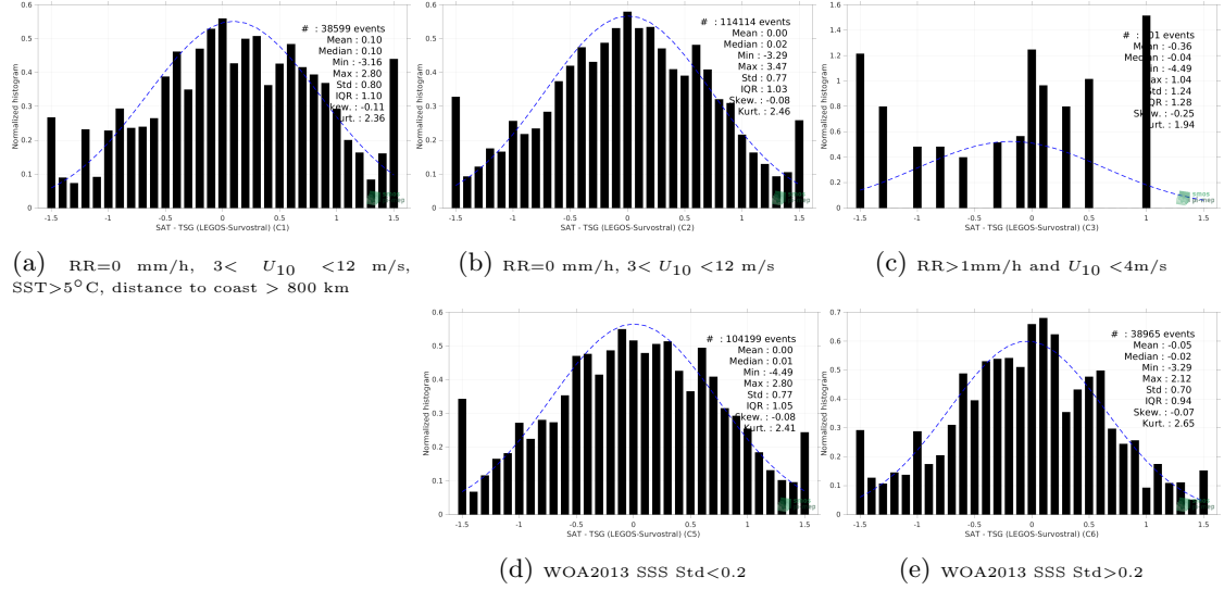
Figure 13: Normalized histogram of \Delta SSS (SMAP SSS L2 v5 (RSS) - TSG (LEGOS-Survostral)) for 5 different subdatasets corresponding to: RR=0 mm/h, 3 < U_{10} < 12 m/s, SST > 5°C, distance to coast > 800 km (a), RR=0 mm/h, 3 < U_{10} < 12 m/s (b), RR > 1mm/h and U_{10} < 4 m/s (c), WOA2013 SSS Std < 0.2 (d), WOA2013 SSS Std > 0.2 (e).
