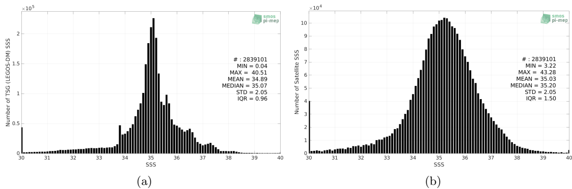
Figure 2: Histograms of SSS from TSG (LEGOS-DM) (a) and SMAP SSS L2 v5 (RSS) (b) considering all match-up pairs per bins of 0.1 over the Global Ocean Pi-MEP region and for the full satellite product period.
