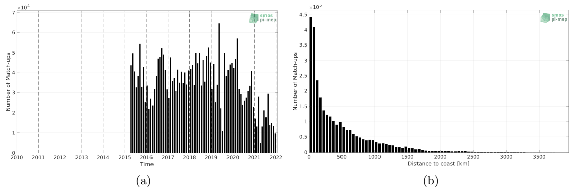
Figure 1: Number of match-ups between TSG (LEGOS-DM) and SMAP SSS L2 v5 (RSS) SSS as a function of time (a) and as function of the distance to coast (b) over the Global Ocean Pi-MEP region and for the full satellite product period.
