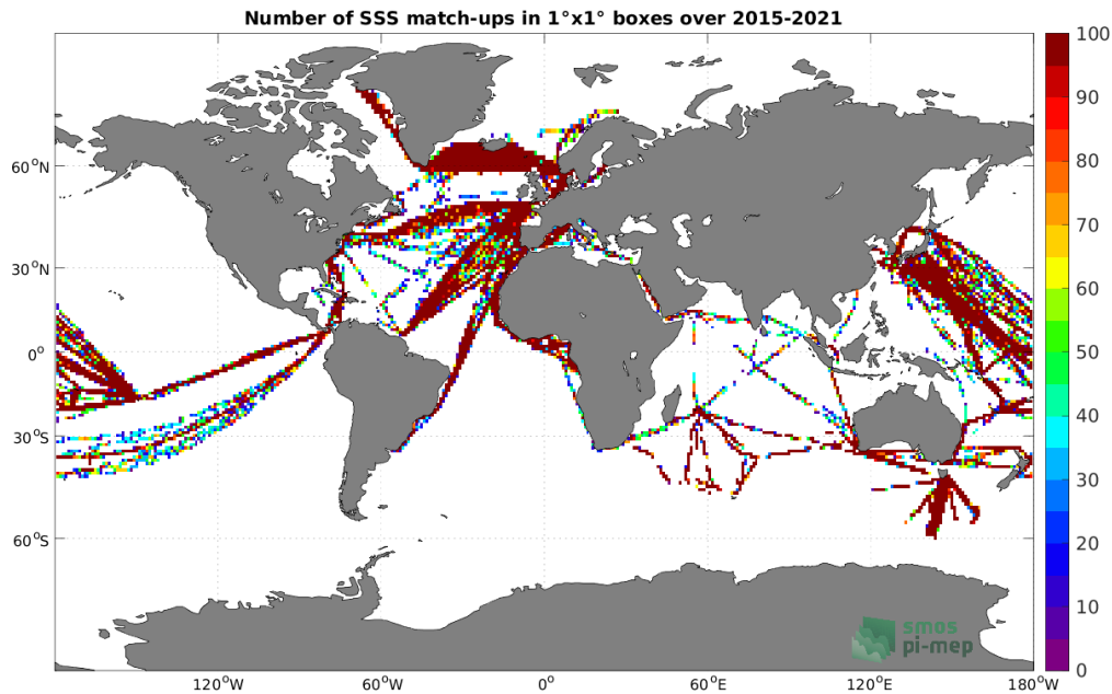
Figure 4: Number of SSS match-ups between TSG (LEGOS-DM) SSS and the SMAP SSS L2 v5 (RSS) SSS product for the Global Ocean Pi-MEP region over 1^\circ \times 1^\circ boxes and for the full satellite product period.
