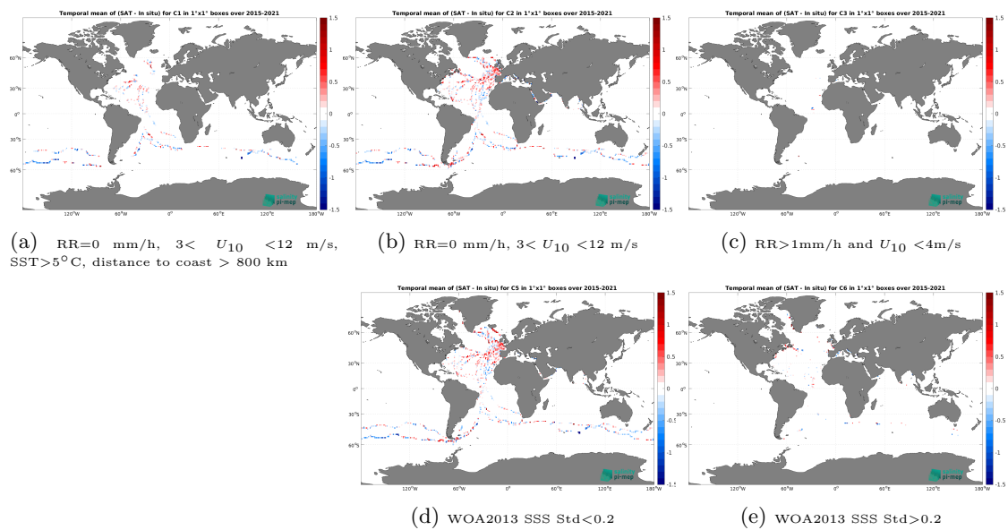
Figure 12: Temporal mean gridded over spatial boxes of size 1^\circ \times 1^\circ of \Delta\text{SSS} (SMAP SSS L2 v5 (RSS) - TSG (GOSUD-Sailing-ship)) for 5 different subdatasets corresponding to:RR=0 mm/h, 3 < U_{10} < 12 m/s, SST > 5^\circ\text{C} , distance to coast > 800 km (a), RR=0 mm/h, 3 < U_{10} < 12 m/s (b), RR > 1 mm/h and U_{10} < 4 m/s (c), WOA2013 SSS Std < 0.2 (d), WOA2013 SSS Std > 0.2 (e).
