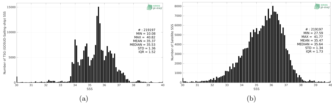
Figure 2: Histograms of SSS from TSG (GOSUD-Sailing-ship) (a) and SMAP SSS L2 v5 (RSS) (b) considering all match-up pairs per bins of 0.1 over the Global Ocean Pi-MEP region and for the full satellite product period.
