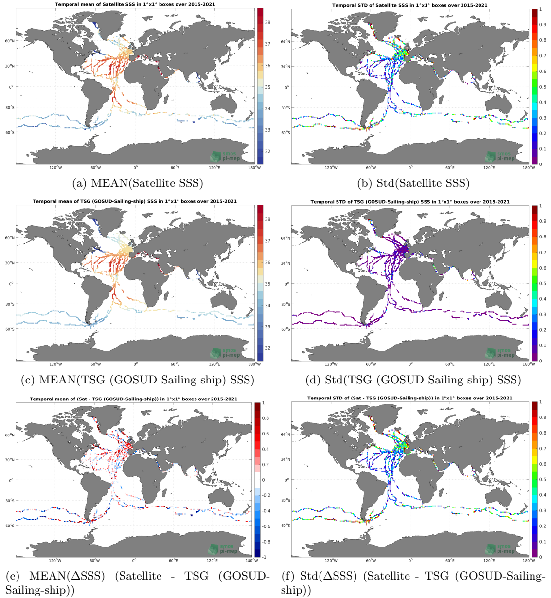
Figure 6: Temporal mean (left) and Std (right) of SSS from SMAP SSS L2 v5 (RSS) (top), TSG (GOSUD-Sailing-ship) (middle), and of \Delta SSS (Satellite - TSG (GOSUD-Sailing-ship)). Only match-up pairs are used to generate these maps.
