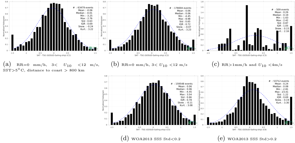
Figure 13: Normalized histogram of \Delta SSS (SMAP SSS L2 v5 (RSS) - TSG (GOSUD-Sailing-ship)) for 5 different subdatasets corresponding to: RR=0 mm/h, 3 < U_{10} < 12 m/s, SST>5°C, distance to coast > 800 km (a), RR=0 mm/h, 3 < U_{10} < 12 m/s (b), RR>1mm/h and U_{10} < 4 m/s (c), WOA2013 SSS Std<0.2 (d), WOA2013 SSS Std>0.2 (e).
