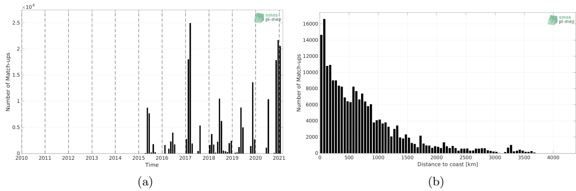
Figure 1: Number of match-ups between TSG (GOSUD-Sailing-ship) and SMAP SSS L2 v5 (RSS) SSS as a function of time (a) and as function of the distance to coast (b) over the Global Ocean Pi-MEP region and for the full satellite product period.
