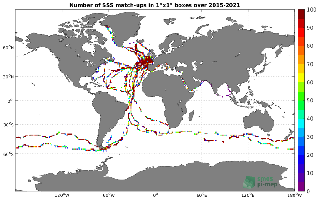
Figure 4: Number of SSS match-ups between TSG (GOSUD-Sailing-ship) SSS and the SMAP SSS L2 v5 (RSS) SSS product for the Global Ocean Pi-MEP region over 1^\circ \times 1^\circ boxes and for the full satellite product period.
