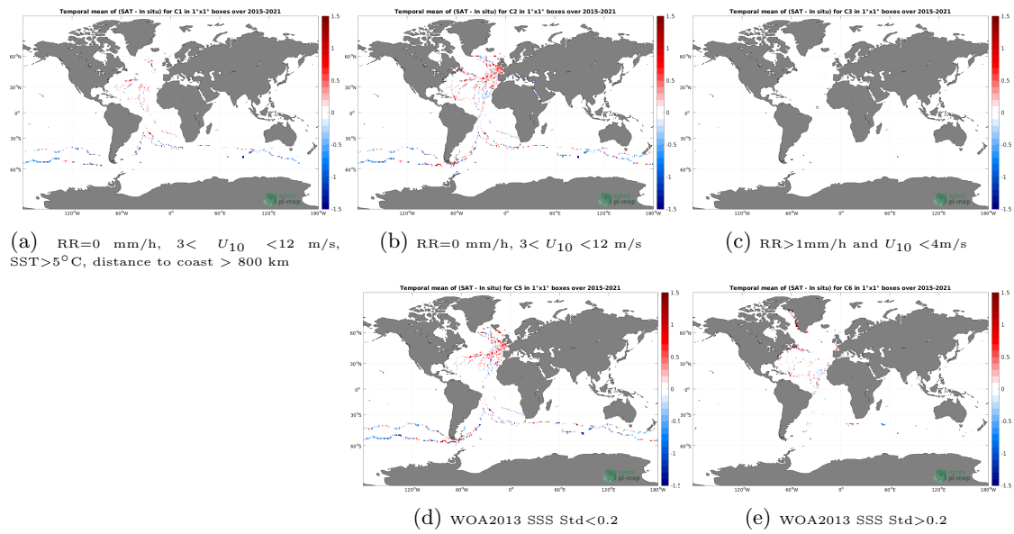
Figure 12: Temporal mean gridded over spatial boxes of size 1^\circ \times 1^\circ of \Delta SSS (SMAP SSS L2 v5 (RSS) - TSG (GOSUD-Sailing-ship)) for 5 different subdatasets corresponding to: RR=0 mm/h, 3 < U_{10} < 12 m/s, SST > 5°C, distance to coast > 800 km (a), RR=0 mm/h, 3 < U_{10} < 12 m/s (b), RR > 1mm/h and U_{10} < 4 m/s (c), WOA2013 SSS Std < 0.2 (d), WOA2013 SSS Std > 0.2 (e).
