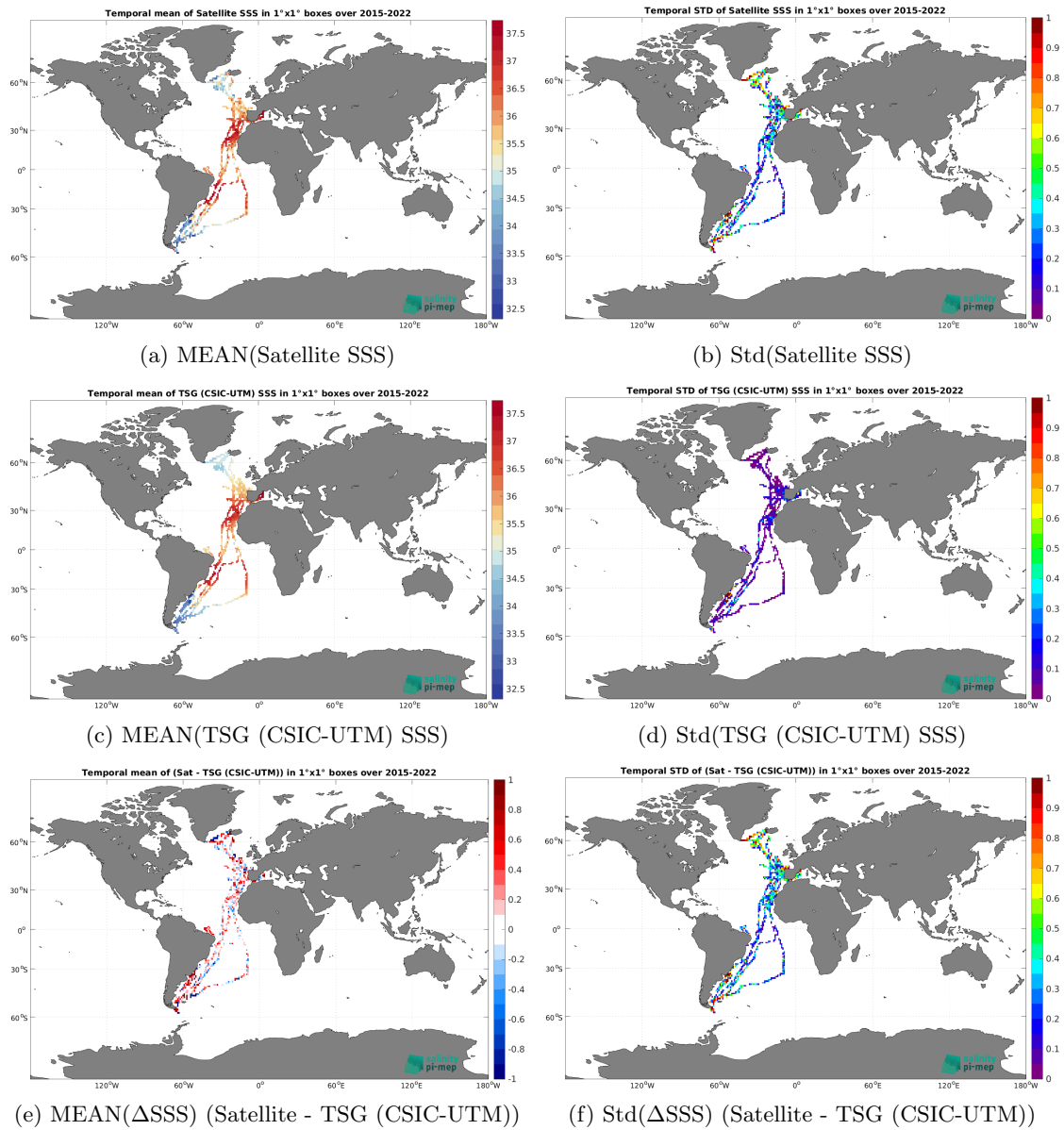
Figure 6: Temporal mean (left) and Std (right) of SSS from SMAP SSS L2 v5 (RSS) (top), TSG (CSIC-UTM) (middle), and of \Delta SSS (Satellite - TSG (CSIC-UTM)). Only match-up pairs are used to generate these maps.
