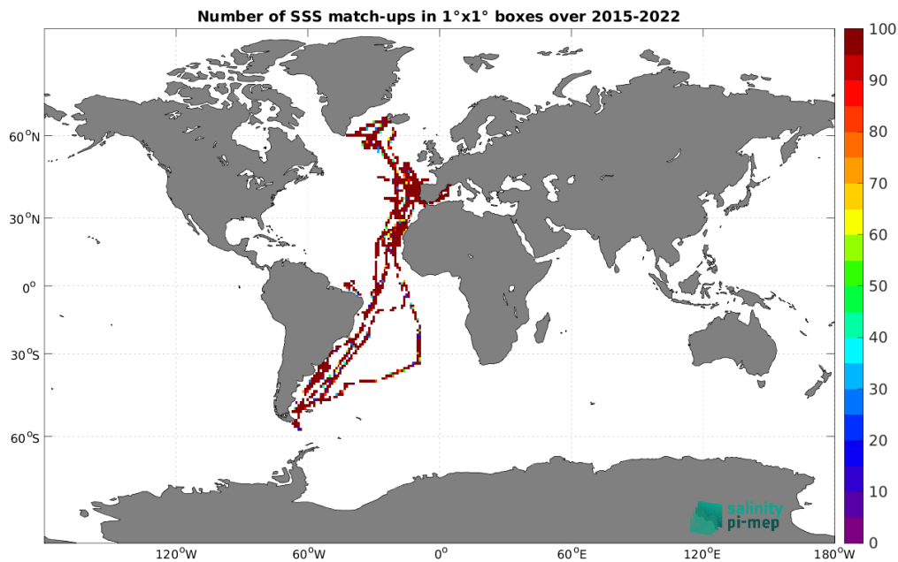
Figure 4: Number of SSS match-ups between TSG (CSIC-UTM) SSS and the SMAP SSS L2 v5 (RSS) SSS product for the Global Ocean Pi-MEP region over 1^\circ \times 1^\circ boxes and for the full satellite product period.
