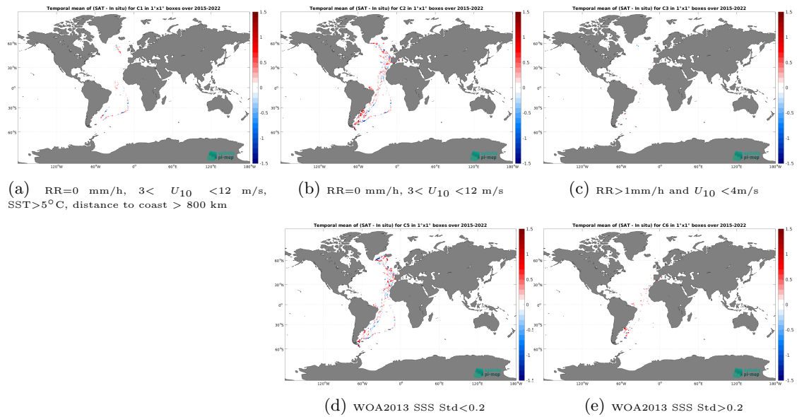
Figure 12: Temporal mean gridded over spatial boxes of size 1^\circ \times 1^\circ of \Delta SSS (SMAP SSS L2 v5 (RSS) - TSG (CSIC-UTM)) for 5 different subdatasets corresponding to:RR=0 mm/h, 3 < U_{10} < 12 m/s, SST >5^\circ C, distance to coast > 800 km (a), RR=0 mm/h, 3 < U_{10} < 12 m/s (b), RR >1 mm/h and U_{10} < 4 m/s (c), WOA2013 SSS Std <0.2 (d), WOA2013 SSS Std >0.2 (e).
