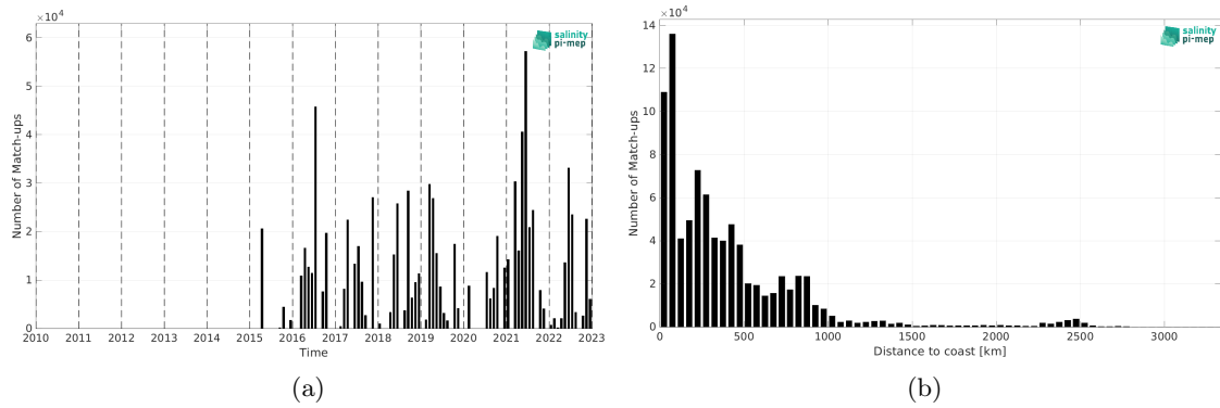
Figure 1: Number of match-ups between TSG (CSIC-UTM) and SMAP SSS L2 v5 (RSS) SSS as a function of time (a) and as function of the distance to coast (b) over the Global Ocean Pi-MEP region and for the full satellite product period.
