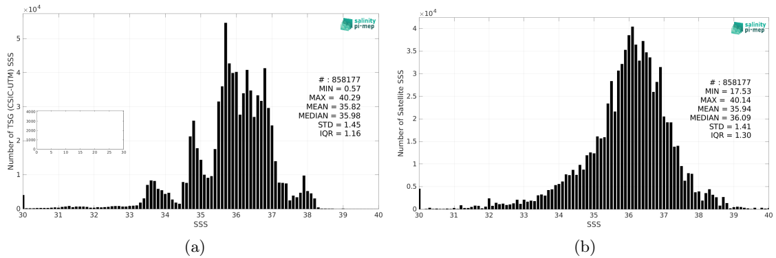
Figure 2: Histograms of SSS from TSG (CSIC-UTM) (a) and SMAP SSS L2 v5 (RSS) (b) considering all match-up pairs per bins of 0.1 over the Global Ocean Pi-MEP region and for the full satellite product period.
