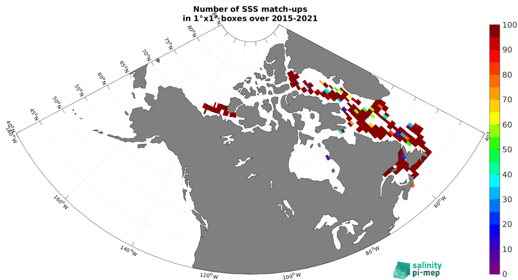
Figure 4: Number of SSS match-ups between TSG (Amundsen) SSS and the SMAP SSS L2 v5 (RSS) SSS product for the Global Ocean Pi-MEP region over 1^\circ \times 1^\circ boxes and for the full satellite product period.
