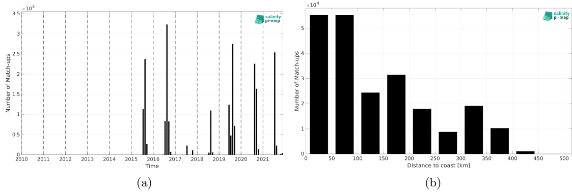
Figure 1: Number of match-ups between TSG (Amundsen) and SMAP SSS L2 v5 (RSS) SSS as a function of time (a) and as function of the distance to coast (b) over the Global Ocean Pi-MEP region and for the full satellite product period.
