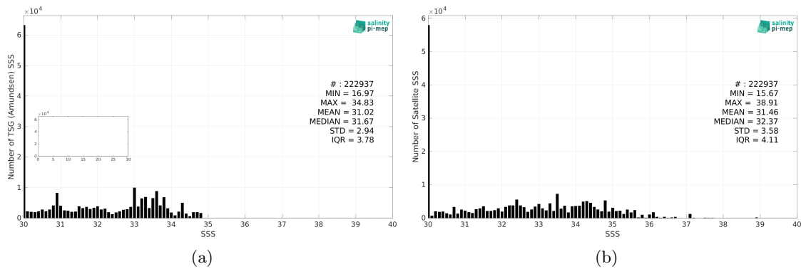
Figure 2: Histograms of SSS from TSG (Amundsen) (a) and SMAP SSS L2 v5 (RSS) (b) considering all match-up pairs per bins of 0.1 over the Global Ocean Pi-MEP region and for the full satellite product period.
