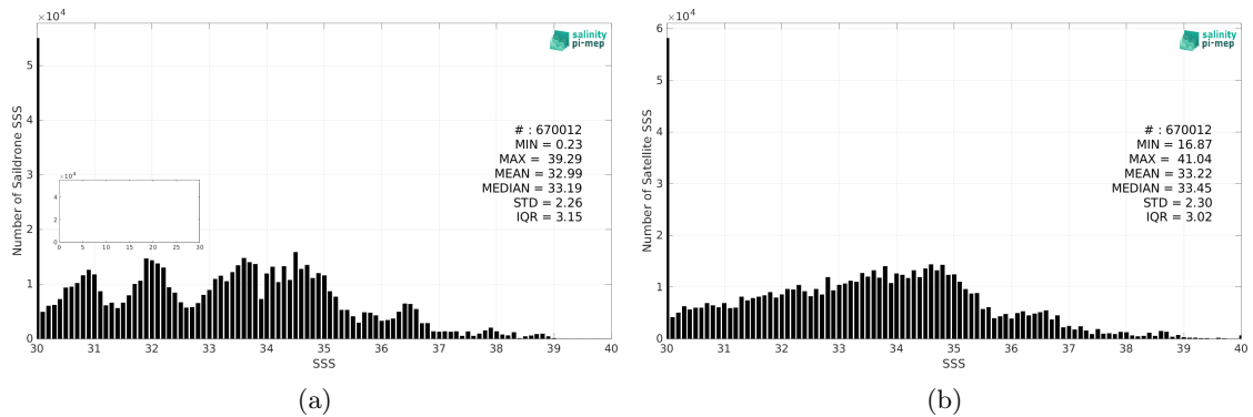
Figure 2: Histograms of SSS from Saildrone (a) and SMAP SSS L2 v5 (RSS) (b) considering all match-up pairs per bins of 0.1 over the Global Ocean Pi-MEP region and for the full satellite product period.
