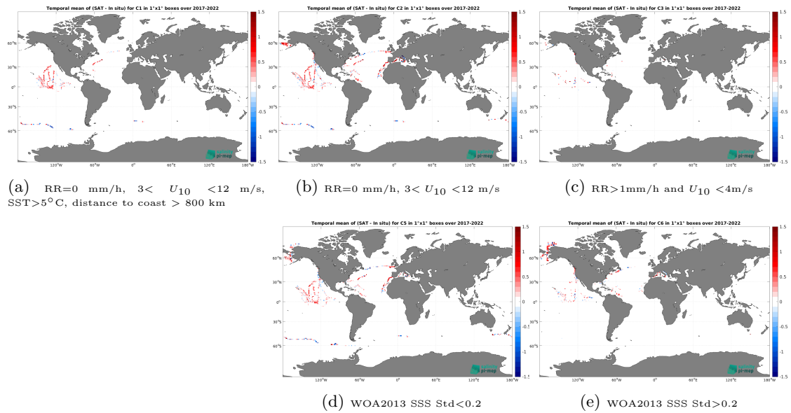
Figure 12: Temporal mean gridded over spatial boxes of size 1^\circ \times 1^\circ of \Delta SSS (SMAP SSS L2 v5 (RSS) - Saifdrone) for 5 different subdatasets corresponding to:RR=0 mm/h, 3 < U_{10} < 12 m/s, SST >5^\circ\text{C} , distance to coast > 800 km (a), RR=0 mm/h, 3 < U_{10} < 12 m/s (b), RR >1 mm/h and U_{10} < 4 m/s (c), WOA2013 SSS Std <0.2 (d), WOA2013 SSS Std >0.2 (e).
