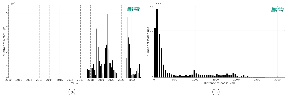
Figure 1: Number of match-ups between Saildrone and SMAP SSS L2 v5 (RSS) SSS as a function of time (a) and as function of the distance to coast (b) over the Global Ocean Pi-MEP region and for the full satellite product period.
