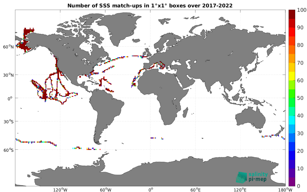
Figure 4: Number of SSS match-ups between Saildrone SSS and the SMAP SSS L2 v5 (RSS) SSS product for the Global Ocean Pi-MEP region over 1^\circ \times 1^\circ boxes and for the full satellite product period.
