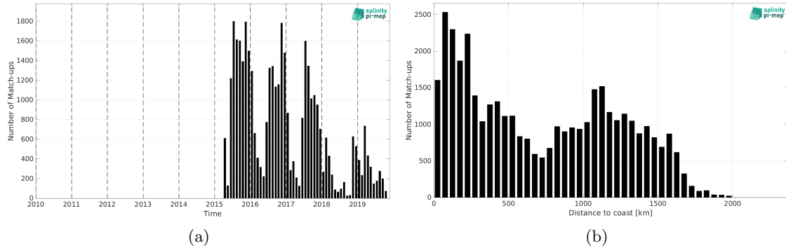
Figure 1: Number of match-ups between Marine mammals and SMAP SSS L2 v5 (RSS) SSS as a function of time (a) and as function of the distance to coast (b) over the Global Ocean Pi-MEP region and for the full satellite product period.
