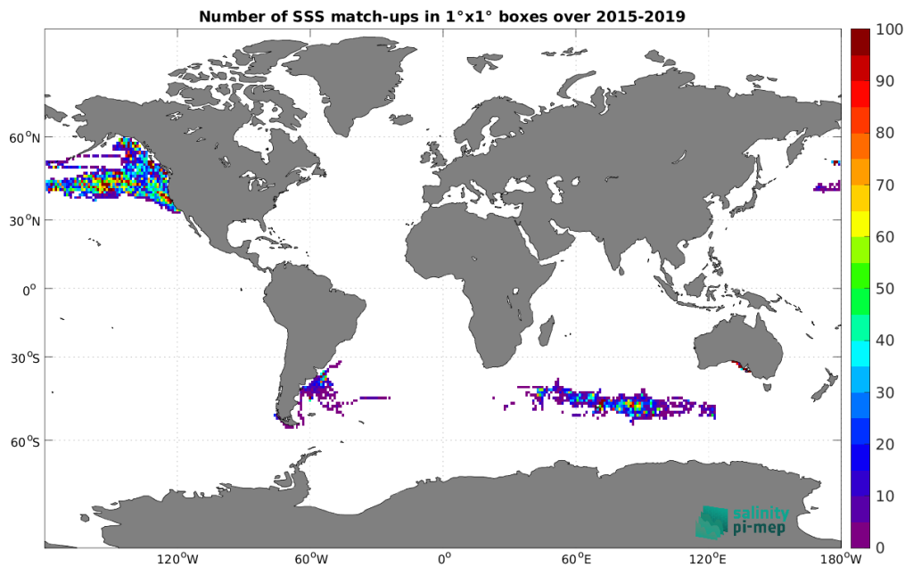
Figure 4: Number of SSS match-ups between Marine mammals SSS and the SMAP SSS L2 v5 (RSS) SSS product for the Global Ocean Pi-MEP region over 1^\circ \times 1^\circ boxes and for the full satellite product period.
