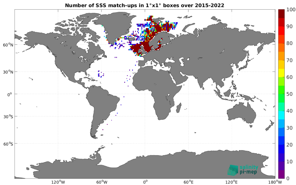
Figure 4: Number of SSS match-ups between ICES SSS and the SMAP SSS L2 v5 (RSS) SSS product for the Global Ocean Pi-MEP region over 1^\circ \times 1^\circ boxes and for the full satellite product period.
