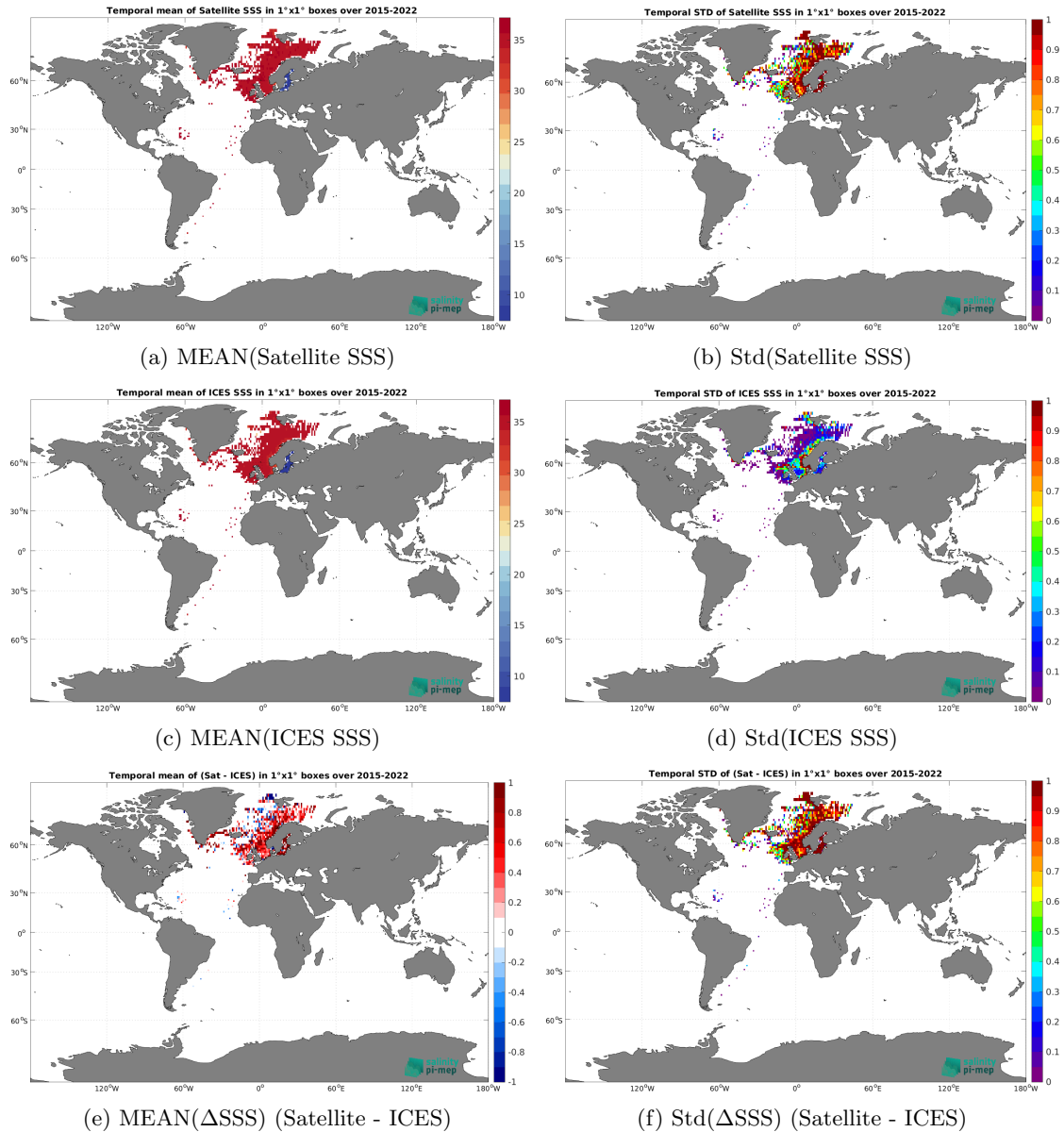
Figure 6: Temporal mean (left) and Std (right) of SSS from SMAP SSS L2 v5 (RSS) (top), ICES (middle), and of \Delta SSS (Satellite - ICES). Only match-up pairs are used to generate these maps.
