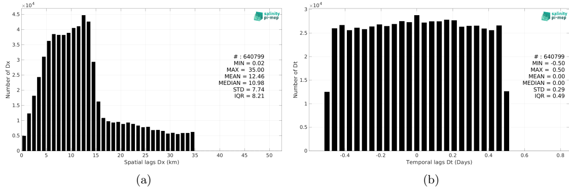
Figure 5: Histograms of the spatial (a) and temporal (b) lags between the location/time of the ICES measurement and the date of the corresponding SMAP SSS L2 v5 (RSS) SSS pixel.
