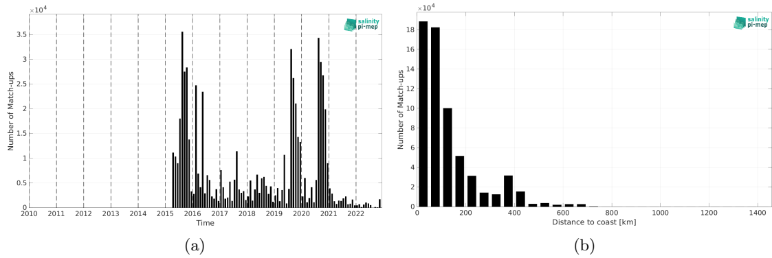
Figure 1: Number of match-ups between ICES and SMAP SSS L2 v5 (RSS) SSS as a function of time (a) and as function of the distance to coast (b) over the Global Ocean Pi-MEP region and for the full satellite product period.
