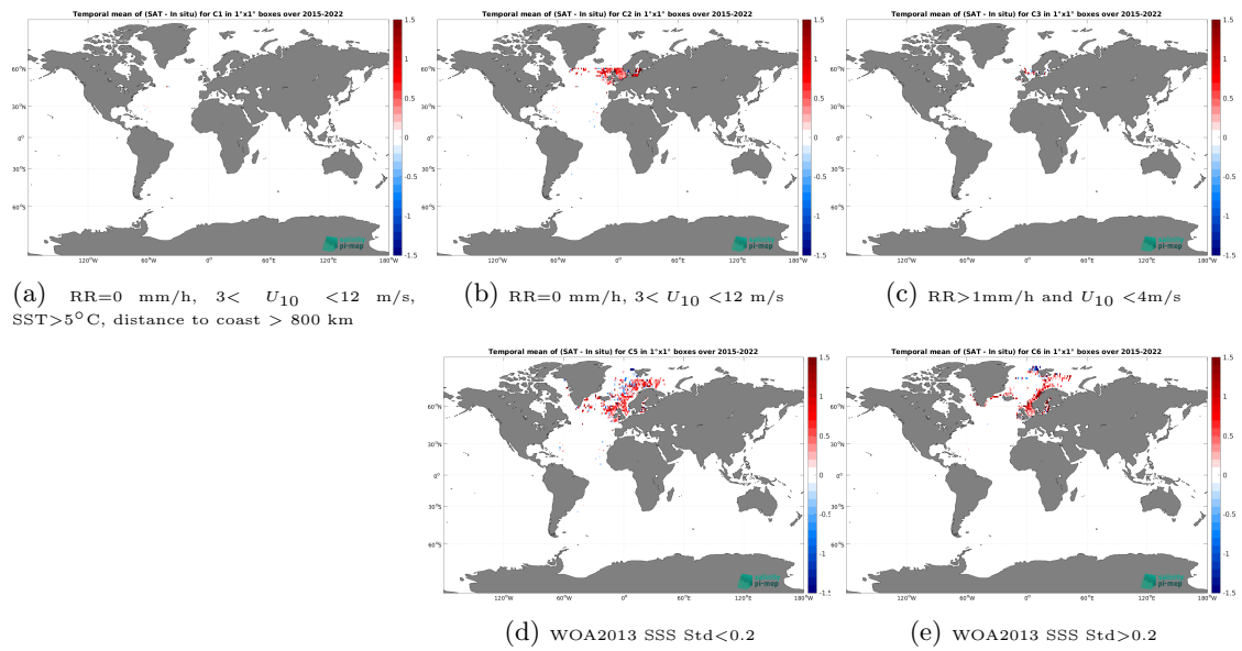
Figure 12: Temporal mean gridded over spatial boxes of size 1^\circ \times 1^\circ of \Delta SSS (SMAP SSS L2 v5 (RSS) - ICES) for 5 different subdatasets corresponding to:RR=0 mm/h, 3 < U_{10} < 12 m/s, SST >5^\circ C, distance to coast > 800 km (a), RR=0 mm/h, 3 < U_{10} < 12 m/s (b), RR >1 mm/h and U_{10} < 4 m/s (c), WOA2013 SSS Std <0.2 (d), WOA2013 SSS Std >0.2 (e).
