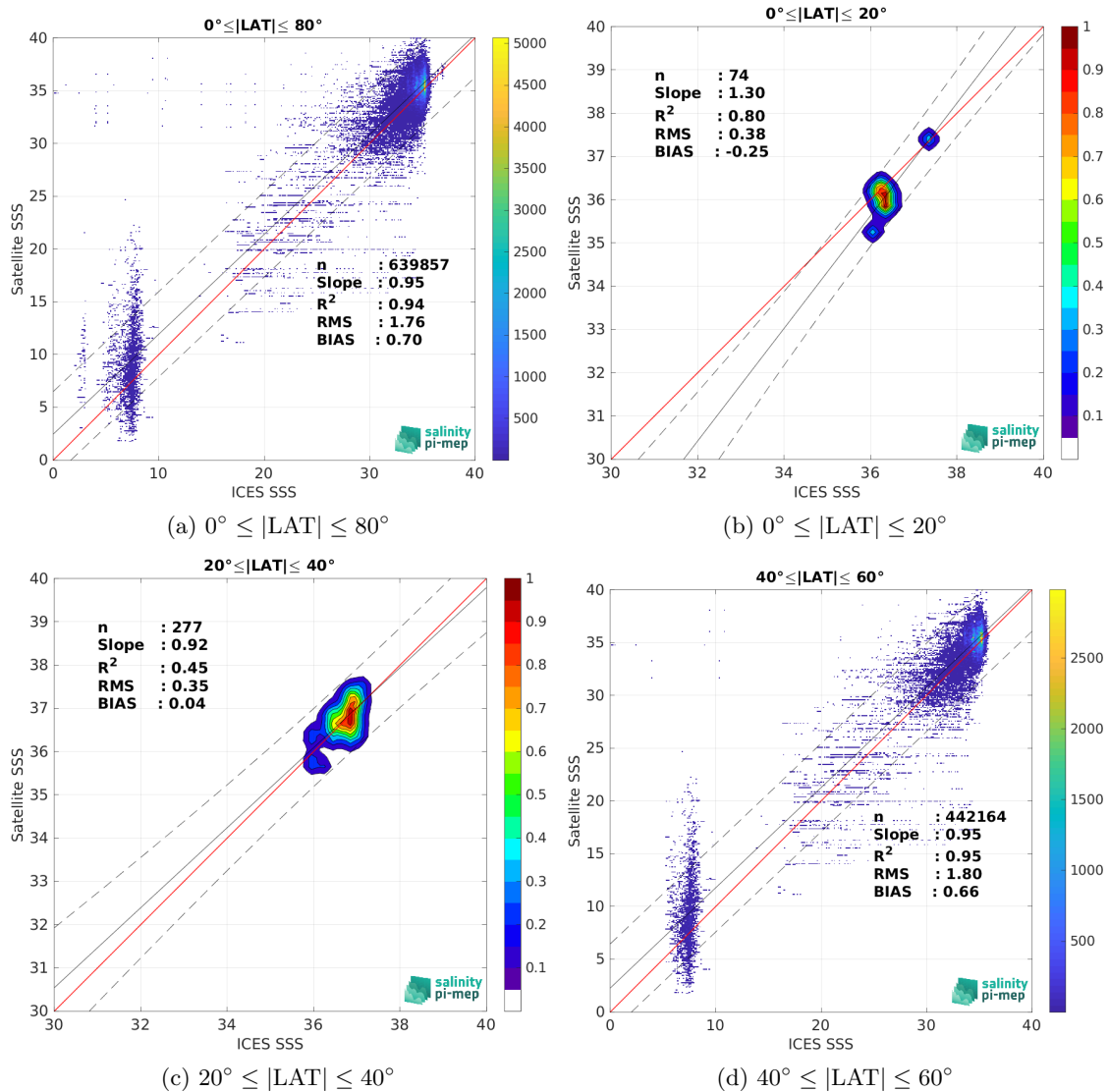
Figure 9: Contour maps of the concentration of SMAP SSS L2 v5 (RSS) SSS (y-axis) versus ICES SSS (x-axis) at match-up pairs for different latitude bands. For each plot, the red line shows x=y . The black thin and dashed lines indicate a linear fit through the data cloud and the \pm 95\% confidence levels, respectively. The number match-up pairs n , the slope and R^2 coefficient of the linear fit, the root mean square (RMS) and the mean bias between satellite and in situ data are indicated for each latitude band in each plots.
