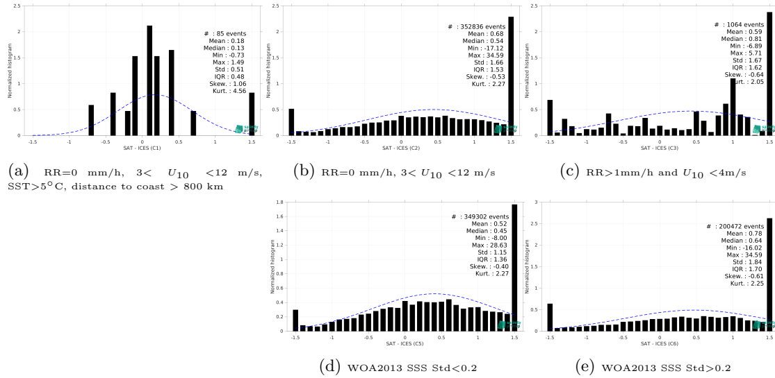
Figure 13: Normalized histogram of \Delta SSS (SMAP SSS L2 v5 (RSS) - ICES) for 5 different subdatasets corresponding to: RR=0 mm/h, 3 < U_{10} < 12 m/s, SST>5°C, distance to coast > 800 km (a), RR=0 mm/h, 3 < U_{10} < 12 m/s (b), RR>1mm/h and U_{10} < 4 m/s (c), WOA2013 SSS Std<0.2 (d), WOA2013 SSS Std>0.2 (e).
