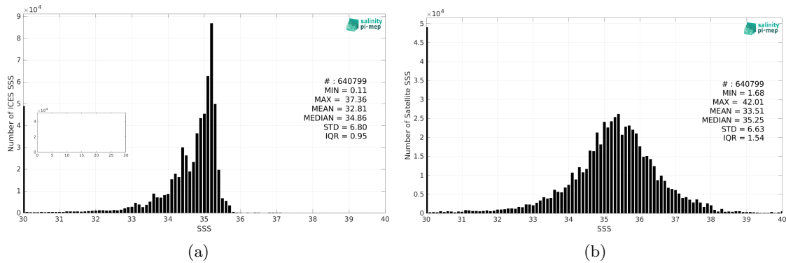
Figure 2: Histograms of SSS from ICES (a) and SMAP SSS L2 v5 (RSS) (b) considering all match-up pairs per bins of 0.1 over the Global Ocean Pi-MEP region and for the full satellite product period.
