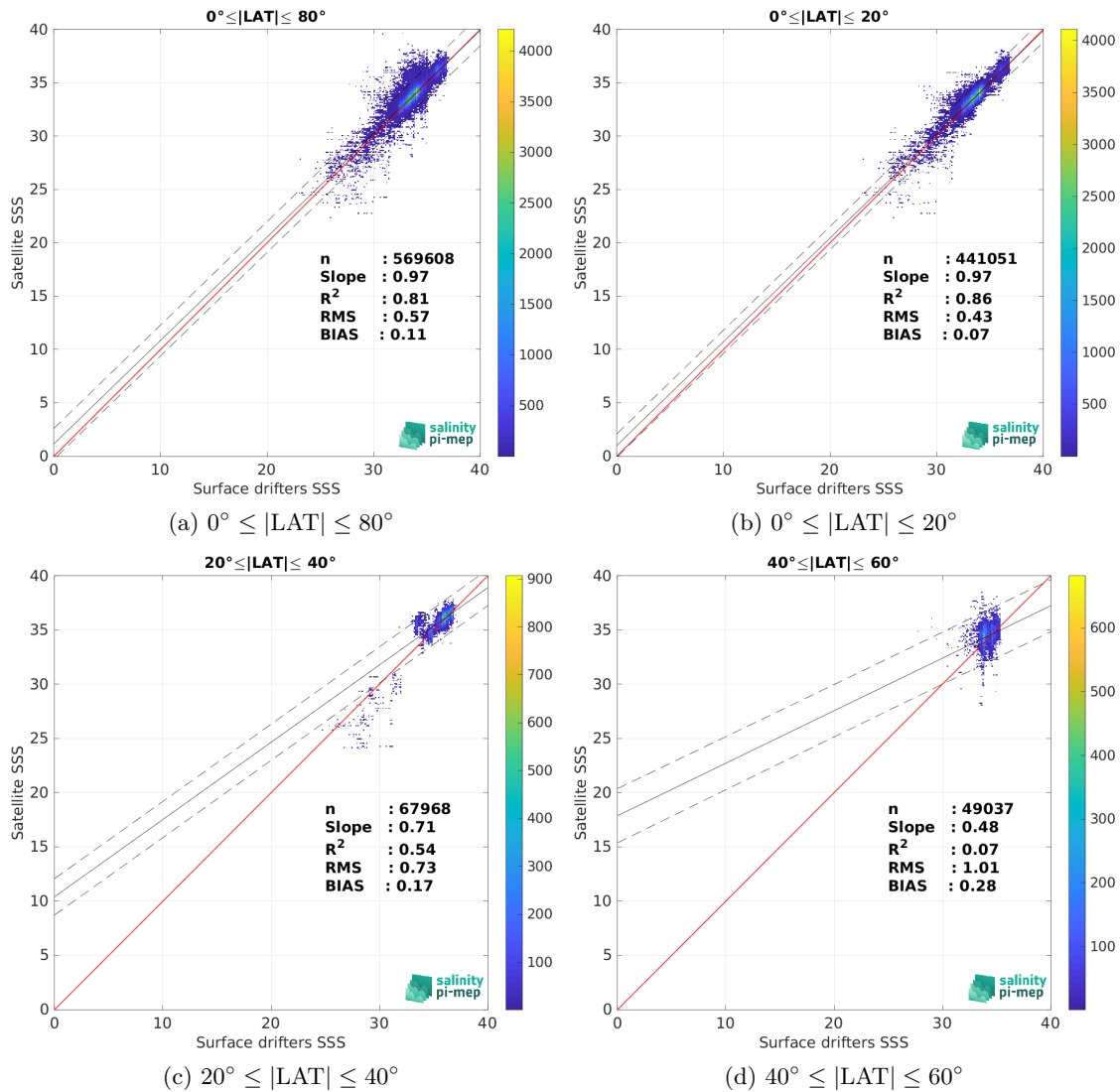
Figure 8: Contour maps of the concentration of SMAP SSS L2 v5 (RSS) SSS (y-axis) versus Surface drifters SSS (x-axis) at match-up pairs for different latitude bands. For each plot, the red line shows x=y . The black thin and dashed lines indicate a linear fit through the data cloud and the \pm 95\% confidence levels, respectively. The number match-up pairs n , the slope and R^2 coefficient of the linear fit, the root mean square (RMS) and the mean bias between satellite and in situ data are indicated for each latitude band in each plots.
