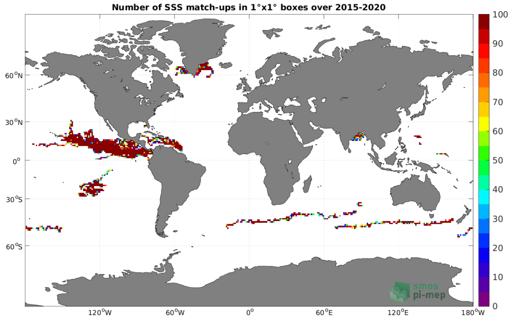
Figure 3: Number of SSS match-ups between Surface drifters SSS and the SMAP SSS L2 v5 (RSS) SSS product for the Global Ocean Pi-MEP region over 1^\circ \times 1^\circ boxes and for the full satellite product period.
