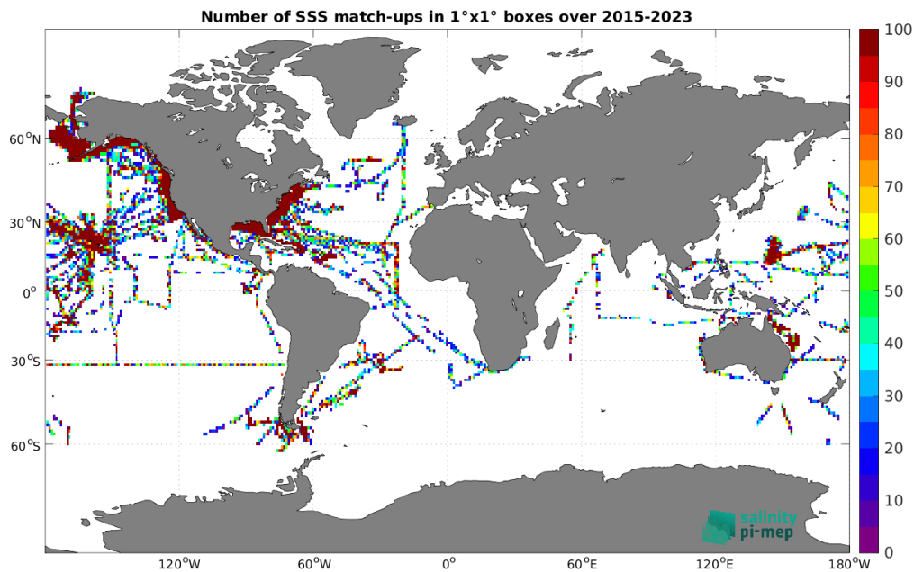
Figure 5: Number of SSS match-ups between TSG (SAMOS) SSS and the SMAP SSS L2 v5.3 (RSS) SSS product for the Global Ocean Pi-MEP region over 1^\circ \times 1^\circ boxes and for the full satellite product period.
