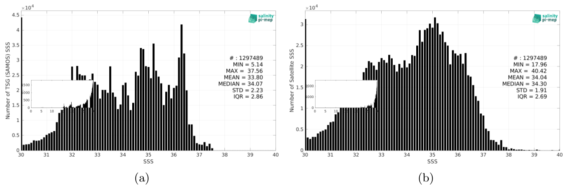
Figure 3: Histograms of SSS from TSG (SAMOS) (a) and SMAP SSS L2 v5.3 (RSS) (b) considering all match-up pairs per bins of 0.1 over the Global Ocean Pi-MEP region and for the full satellite product period.
