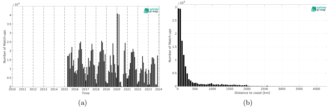
Figure 2: Number of match-ups between TSG (SAMOS) and SMAP SSS L2 v5.3 (RSS) SSS as a function of time (a) and as function of the distance to coast (b) over the Global Ocean Pi-MEP region and for the full satellite product period.
