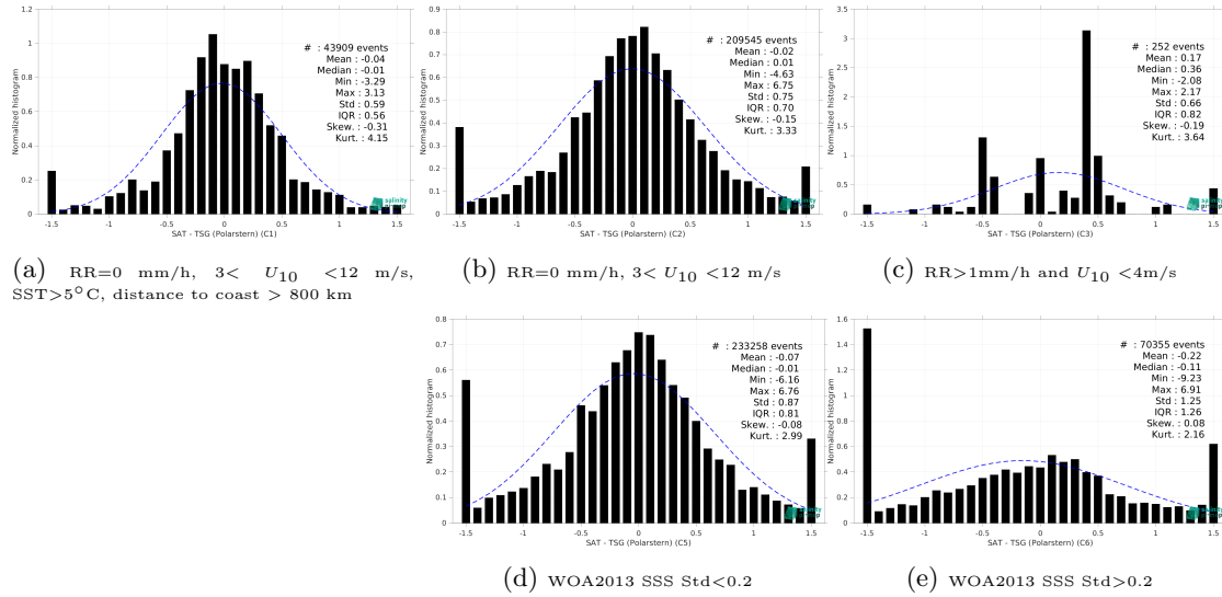
Figure 15: Normalized histogram of \Delta SSS (SMAP SSS L2 v5.3 (RSS) - TSG (Polarstern)) for 5 different subdatasets corresponding to: RR=0 mm/h, 3 < U_{10} < 12 m/s, SST>5°C, distance to coast > 800 km (a), RR=0 mm/h, 3 < U_{10} < 12 m/s (b), RR>1mm/h and U_{10} < 4 m/s (c), WOA2013 SSS Std<0.2 (d), WOA2013 SSS Std>0.2 (e).
