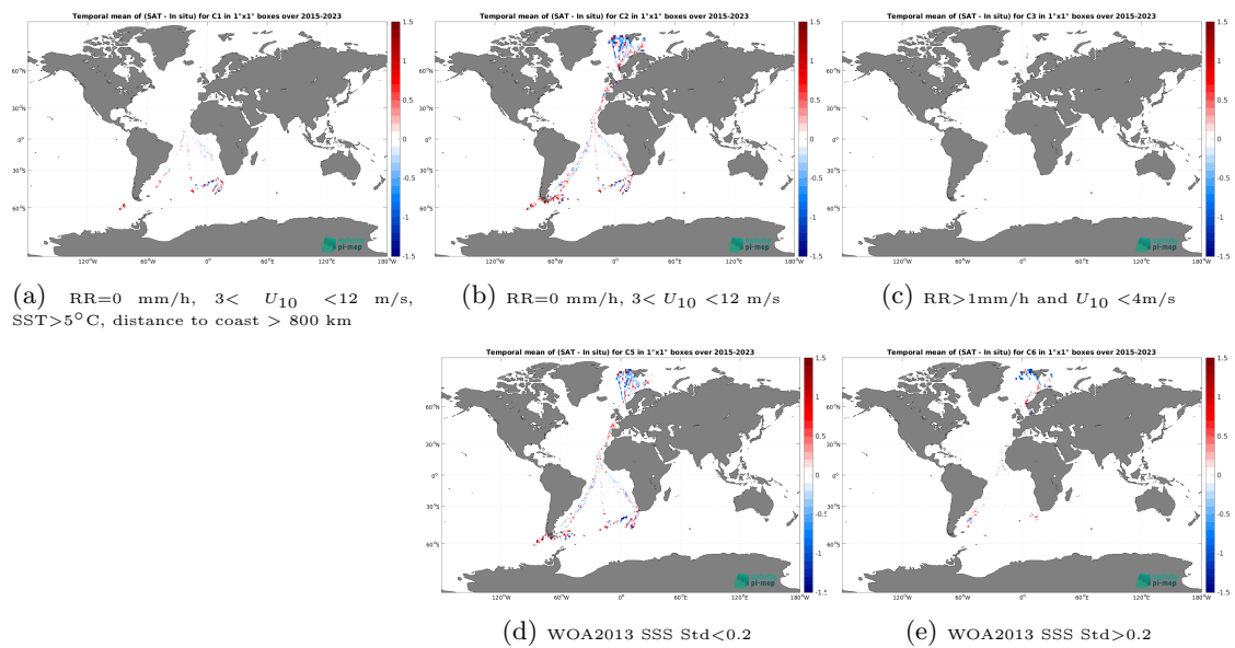
Figure 14: Temporal mean gridded over spatial boxes of size 1^\circ \times 1^\circ of \Delta SSS (SMAP SSS L2 v5.3 (RSS) - TSG (Polarstern)) for 5 different subdatasets corresponding to:RR=0 mm/h, 3 < U_{10} < 12 m/s, SST > 5^\circ\text{C} , distance to coast > 800 km (a), RR=0 mm/h, 3 < U_{10} < 12 m/s (b), RR > 1 mm/h and U_{10} < 4 m/s (c), WOA2013 SSS Std < 0.2 (d), WOA2013 SSS Std > 0.2 (e).
