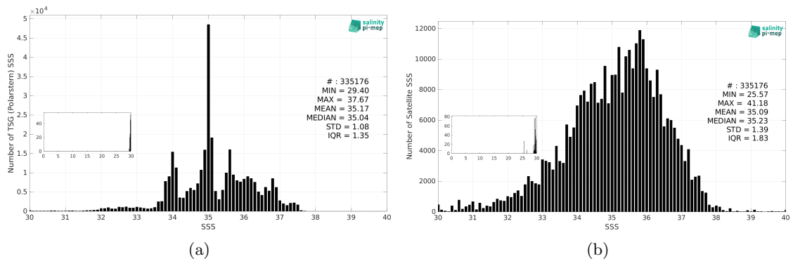
Figure 3: Histograms of SSS from TSG (Polarstern) (a) and SMAP SSS L2 v5.3 (RSS) (b) considering all match-up pairs per bins of 0.1 over the Global Ocean Pi-MEP region and for the full satellite product period.
