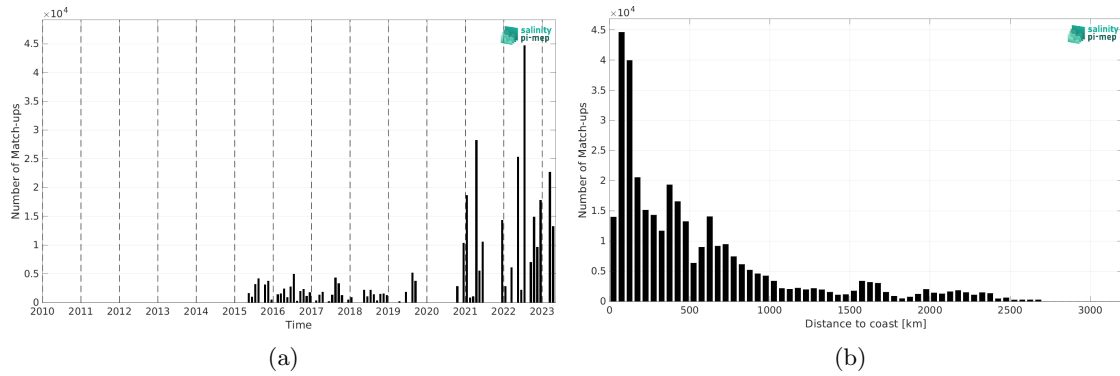
Figure 2: Number of match-ups between TSG (Polarstern) and SMAP SSS L2 v5.3 (RSS) SSS as a function of time (a) and as function of the distance to coast (b) over the Global Ocean Pi-MEP region and for the full satellite product period.
