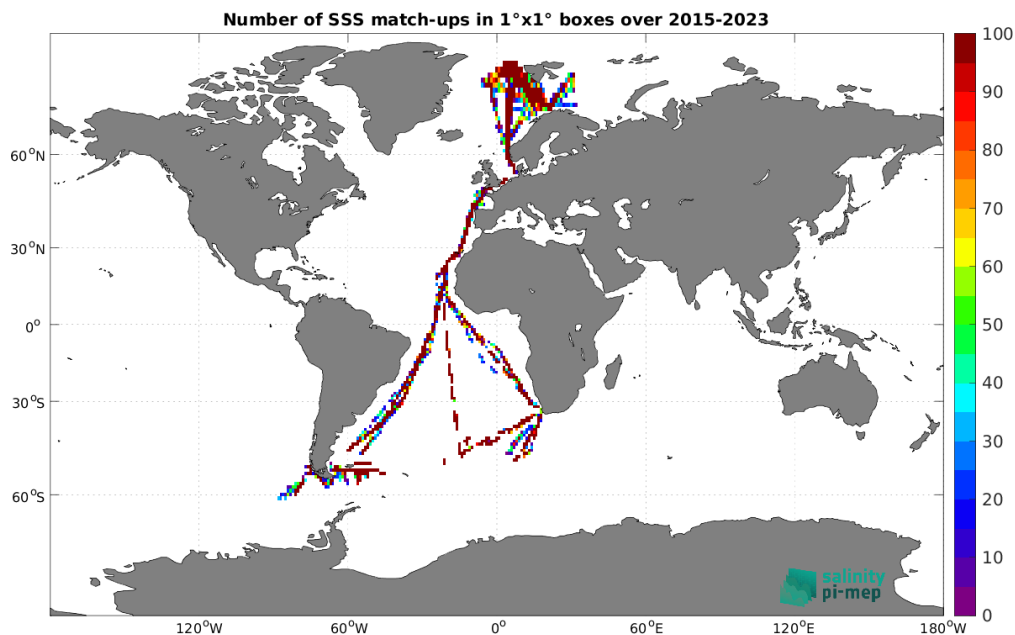
Figure 5: Number of SSS match-ups between TSG (Polarstern) SSS and the SMAP SSS L2 v5.3 (RSS) SSS product for the Global Ocean Pi-MEP region over 1^\circ \times 1^\circ boxes and for the full satellite product period.
