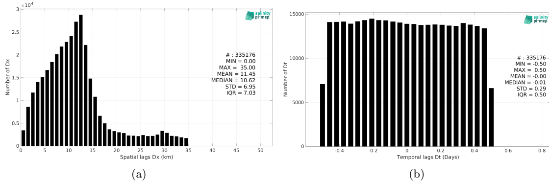
Figure 6: Histograms of the spatial (a) and temporal (b) lags between the location/time of the TSG (Polarstern) measurement and the date of the corresponding SMAP SSS L2 v5.3 (RSS) SSS pixel.
