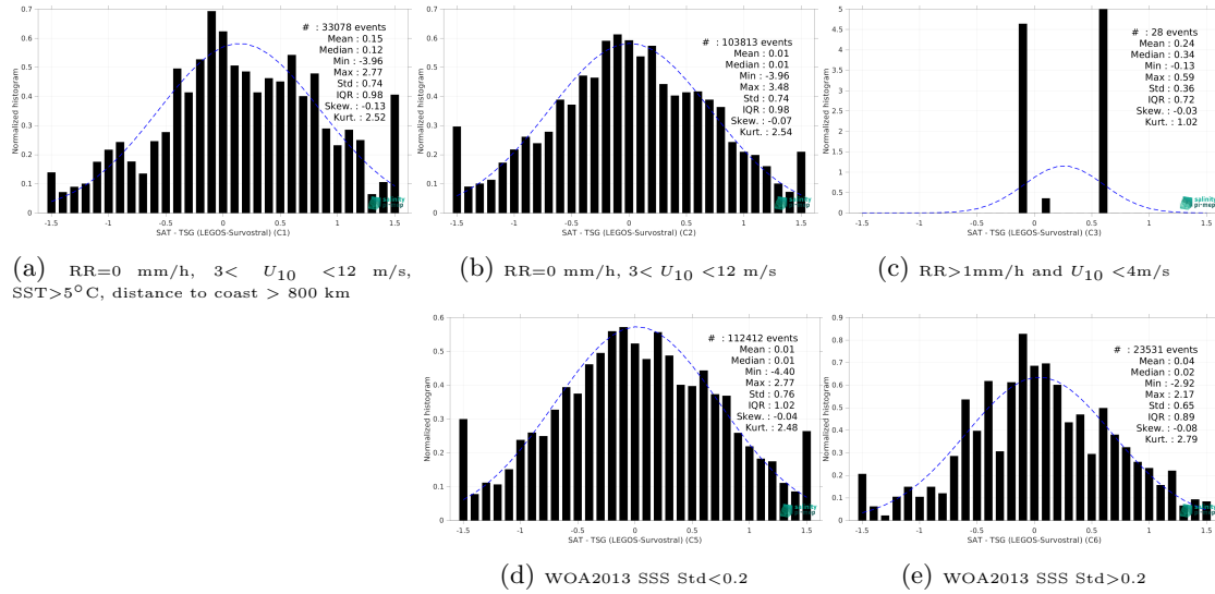
Figure 15: Normalized histogram of \Delta SSS (SMAP SSS L2 v5.3 (RSS) - TSG (LEGOS-Survostral)) for 5 different subdatasets corresponding to: RR=0 mm/h, 3 < U_{10} < 12 m/s, SST > 5°C, distance to coast > 800 km (a), RR=0 mm/h, 3 < U_{10} < 12 m/s (b), RR > 1mm/h and U_{10} < 4 m/s (c), WOA2013 SSS Std < 0.2 (d), WOA2013 SSS Std > 0.2 (e).
