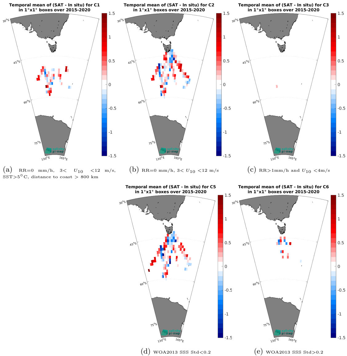
Figure 14: Temporal mean gridded over spatial boxes of size 1^\circ \times 1^\circ of \Delta SSS (SMAP SSS L2 v5.3 (RSS) - TSG (LEGOS-Survostral)) for 5 different subdatasets corresponding to:RR=0 mm/h, 3 < U_{10} < 12 m/s, SST>5°C, distance to coast > 800 km (a), RR=0 mm/h, 3 < U_{10} < 12 m/s (b), RR>1mm/h and U_{10} < 4 m/s (c), WOA2013 SSS Std<0.2 (d), WOA2013 SSS Std>0.2 (e).
