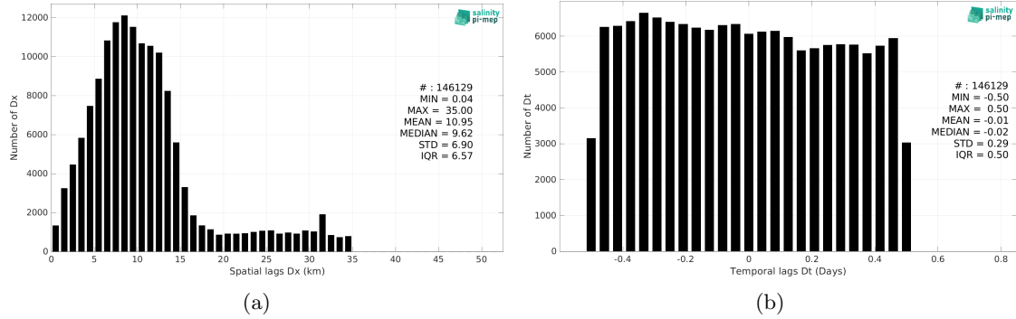
Figure 6: Histograms of the spatial (a) and temporal (b) lags between the location/time of the TSG (LEGOS-Survostral) measurement and the date of the corresponding SMAP SSS L2 v5.3 (RSS) SSS pixel.
