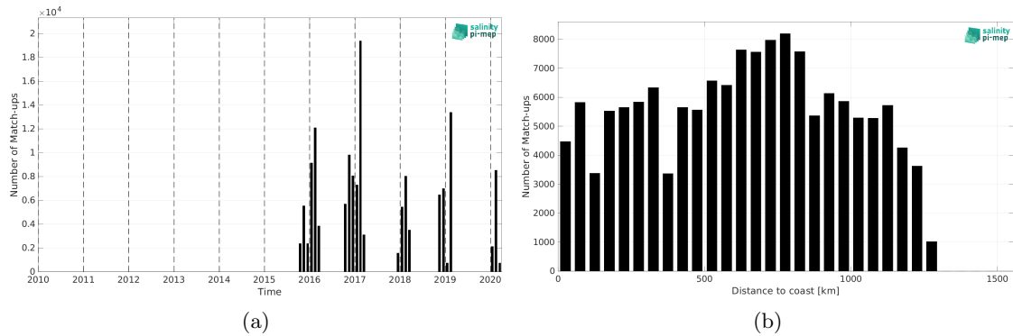
Figure 2: Number of match-ups between TSG (LEGOS-Survostral) and SMAP SSS L2 v5.3 (RSS) SSS as a function of time (a) and as function of the distance to coast (b) over the Global Ocean Pi-MEP region and for the full satellite product period.
