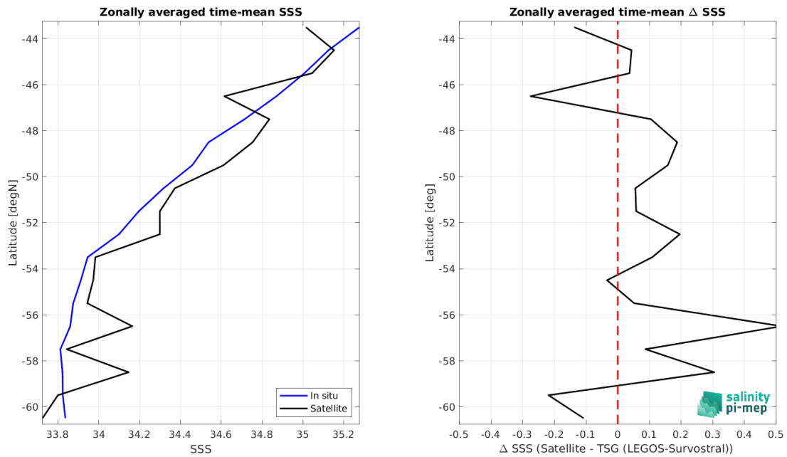
Figure 9: Left panel: Zonal mean SSS from SMAP SSS L2 v5.3 (RSS) satellite product (black) and from TSG (LEGOS-Survostral) (blue). Right panel: Zonal mean of \Delta SSS (Satellite - TSG (LEGOS-Survostral)) for all the collected Pi-MEP match-up pairs estimated over the full satellite product period.
