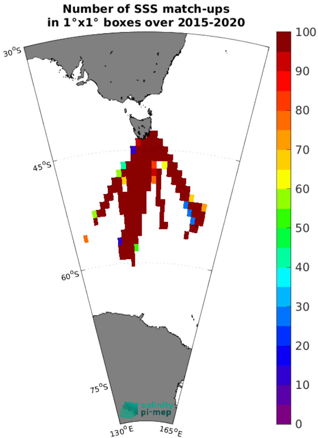
Figure 5: Number of SSS match-ups between TSG (LEGOS-Survostral) SSS and the SMAP SSS L2 v5.3 (RSS) SSS product for the Global Ocean Pi-MEP region over 1°x1° boxes and for the full satellite product period.
