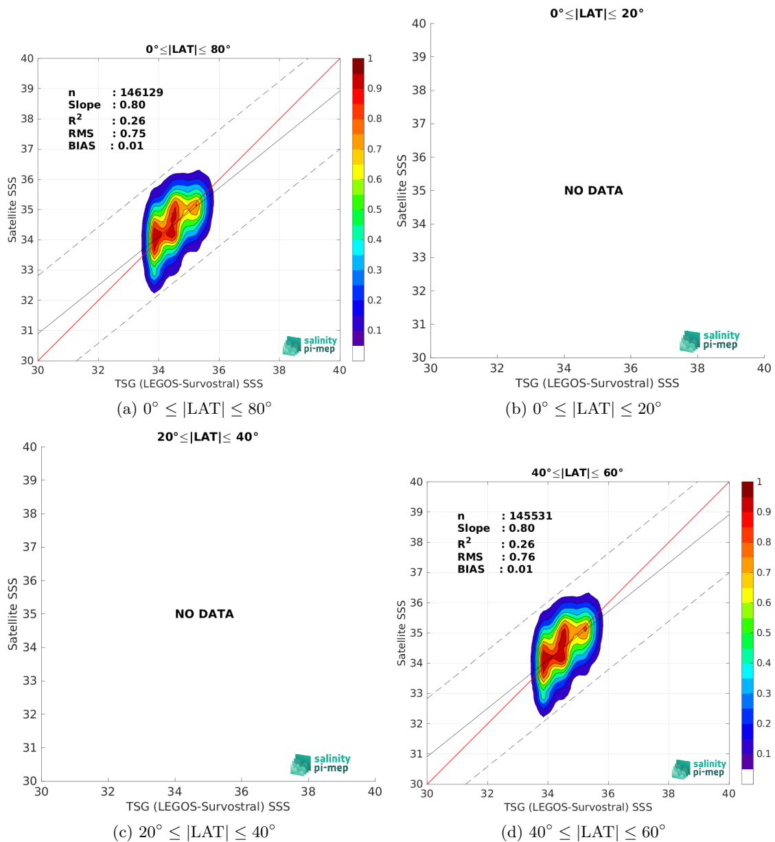
Figure 10: Contour maps of the concentration of SMAP SSS L2 v5.3 (RSS) SSS (y-axis) versus TSG (LEGOS-Survostral) SSS (x-axis) at match-up pairs for different latitude bands. For each plot, the red line shows x=y . The black thin and dashed lines indicate a linear fit through the data cloud and the \pm 95\% confidence levels, respectively. The number match-up pairs n , the slope and R^2 coefficient of the linear fit, the root mean square (RMS) and the mean bias between satellite and in situ data are indicated for each latitude band in each plots.
