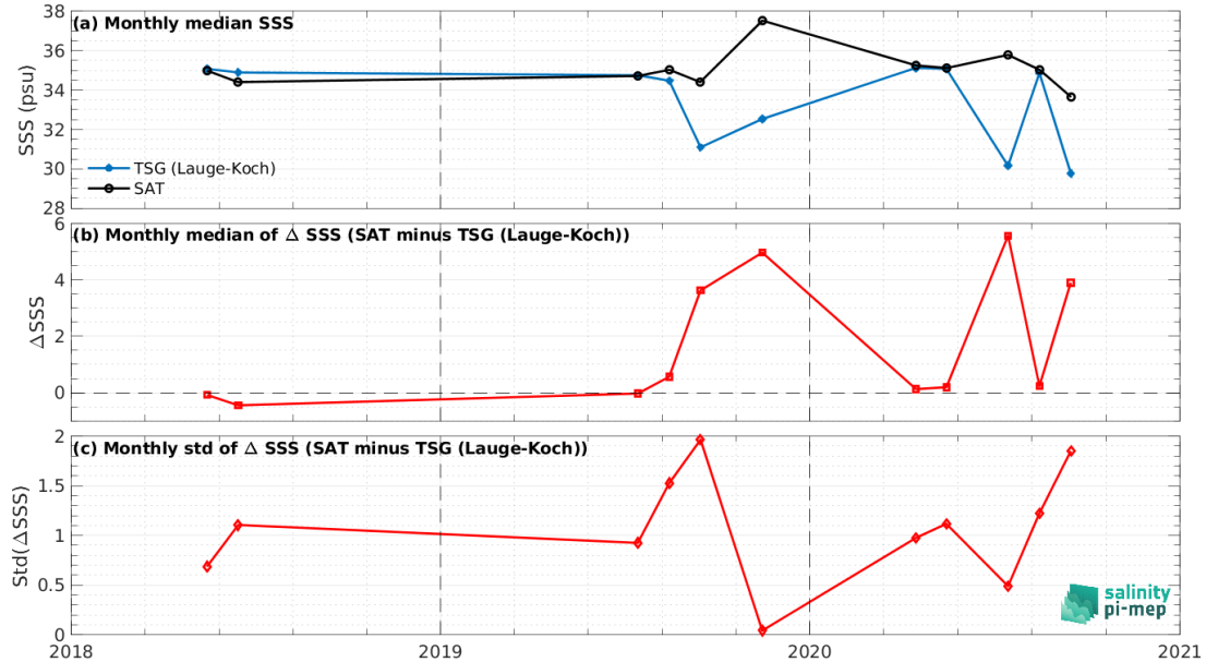
Figure 8: Time series of the monthly median SSS (top), median of \Delta\text{SSS} (Satellite - TSG (Lauge-Koch)) and Std of \Delta\text{SSS} (Satellite - TSG (Lauge-Koch)) over the Global Ocean Pi-MEP region considering all match-ups collected by the Pi-MEP.
