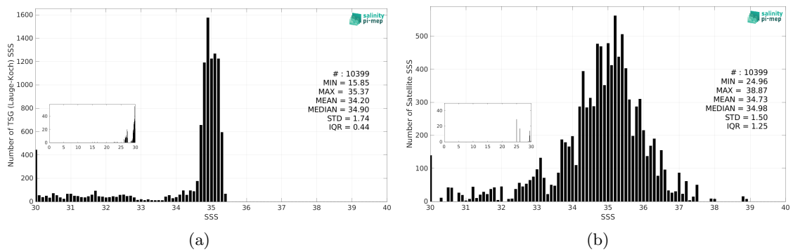
Figure 3: Histograms of SSS from TSG (Lauge-Koch) (a) and SMAP SSS L2 v5.3 (RSS) (b) considering all match-up pairs per bins of 0.1 over the Global Ocean Pi-MEP region and for the full satellite product period.
