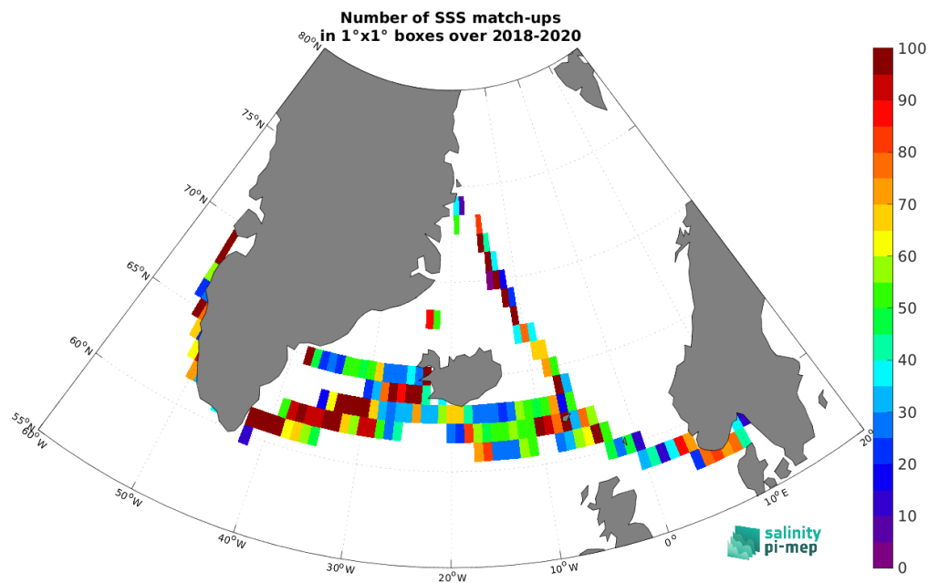
Figure 5: Number of SSS match-ups between TSG (Lauge-Koch) SSS and the SMAP SSS L2 v5.3 (RSS) SSS product for the Global Ocean Pi-MEP region over 1^\circ \times 1^\circ boxes and for the full satellite product period.
