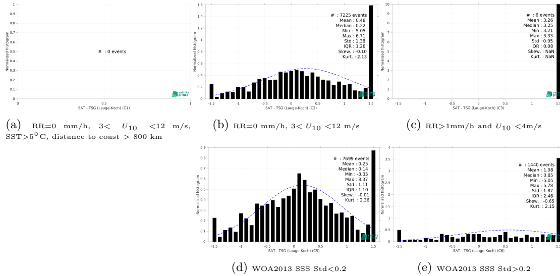
Figure 15: Normalized histogram of \Delta SSS (SMAP SSS L2 v5.3 (RSS) - TSG (Lauge-Koch)) for 5 different subdatasets corresponding to: RR=0 mm/h, 3 < U_{10} < 12 m/s, SST>5°C, distance to coast > 800 km (a), RR=0 mm/h, 3 < U_{10} < 12 m/s (b), RR>1mm/h and U_{10} < 4 m/s (c), WOA2013 SSS Std<0.2 (d), WOA2013 SSS Std>0.2 (e).
