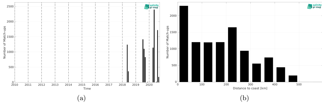
Figure 2: Number of match-ups between TSG (Lauge-Koch) and SMAP SSS L2 v5.3 (RSS) SSS as a function of time (a) and as function of the distance to coast (b) over the Global Ocean Pi-MEP region and for the full satellite product period.
