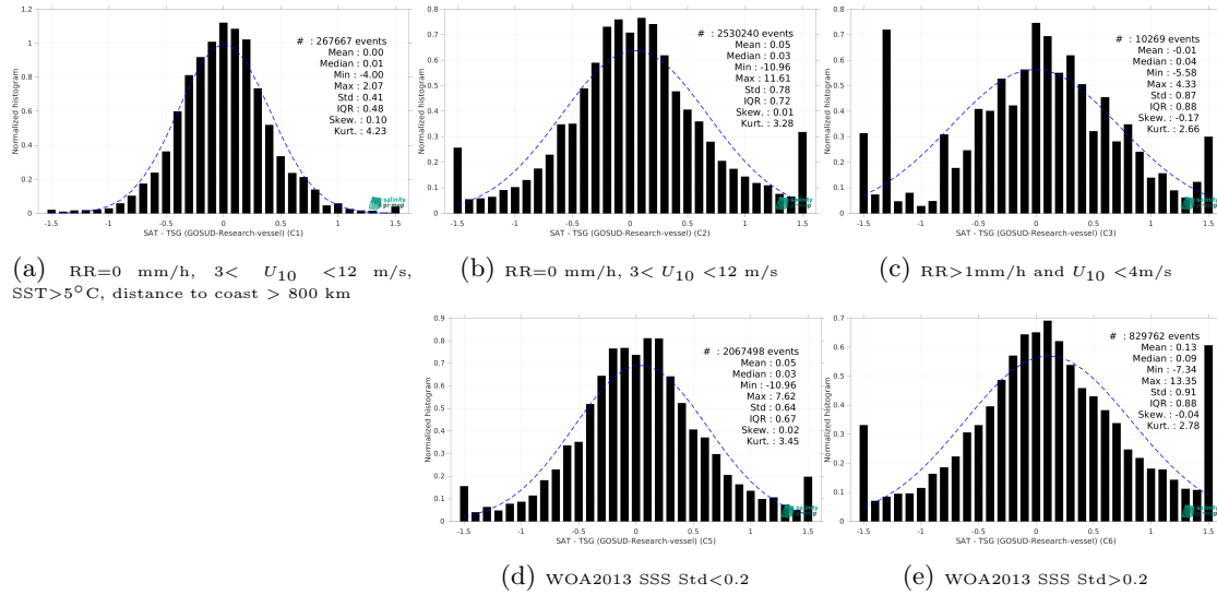
Figure 15: Normalized histogram of \Delta SSS (SMAP SSS L2 v5.3 (RSS) - TSG (GOSUD-Research-vessel)) for 5 different subdatasets corresponding to: RR=0 mm/h, 3 < U_{10} < 12 m/s, SST>5°C, distance to coast > 800 km (a), RR=0 mm/h, 3 < U_{10} < 12 m/s (b), RR>1mm/h and U_{10} < 4 m/s (c), WOA2013 SSS Std<0.2 (d), WOA2013 SSS Std>0.2 (e).
