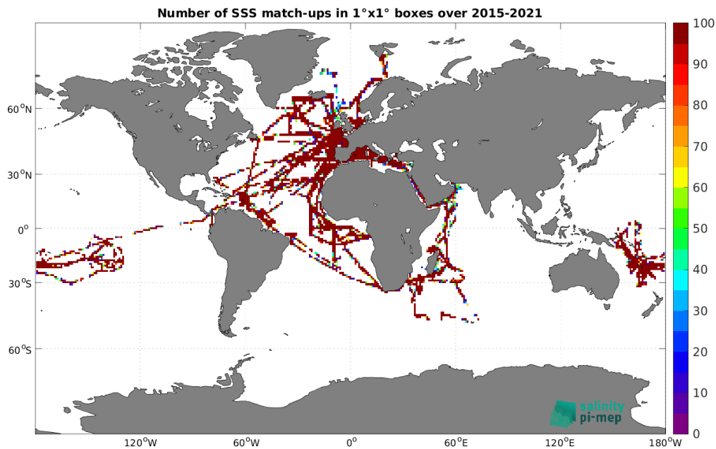
Figure 5: Number of SSS match-ups between TSG (GOSUD-Research-vessel) SSS and the SMAP SSS L2 v5.3 (RSS) SSS product for the Global Ocean Pi-MEP region over 1^\circ \times 1^\circ boxes and for the full satellite product period.
