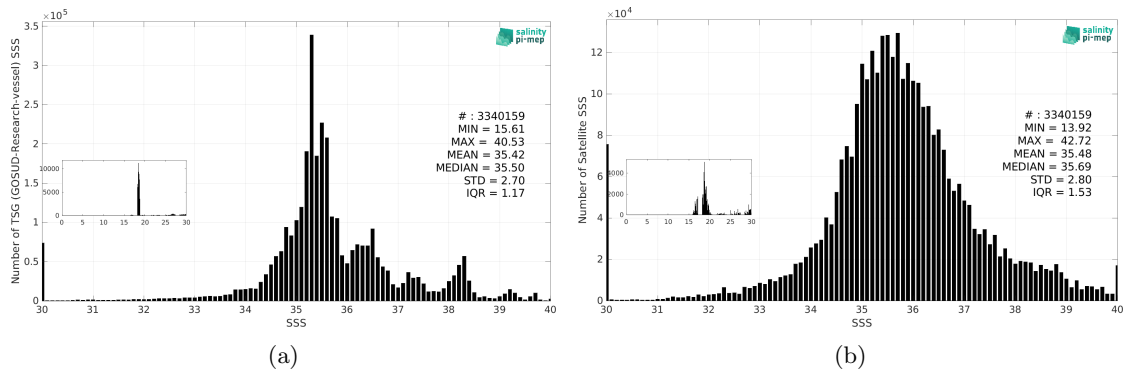
Figure 3: Histograms of SSS from TSG (GOSUD-Research-vessel) (a) and SMAP SSS L2 v5.3 (RSS) (b) considering all match-up pairs per bins of 0.1 over the Global Ocean Pi-MEP region and for the full satellite product period.
