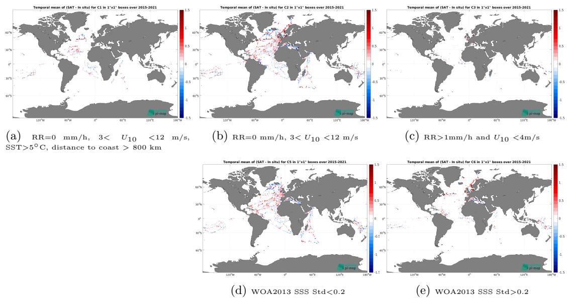
Figure 14: Temporal mean gridded over spatial boxes of size 1^\circ \times 1^\circ of \Delta SSS (SMAP SSS L2 v5.3 (RSS) - TSG (GOSUD-Research-vessel)) for 5 different subdatasets corresponding to:RR=0 mm/h, 3 < U_{10} < 12 m/s, SST > 5^\circ\text{C} , distance to coast > 800 km (a), RR=0 mm/h, 3 < U_{10} < 12 m/s (b), RR > 1 mm/h and U_{10} < 4 m/s (c), WOA2013 SSS Std < 0.2 (d), WOA2013 SSS Std > 0.2 (e).
