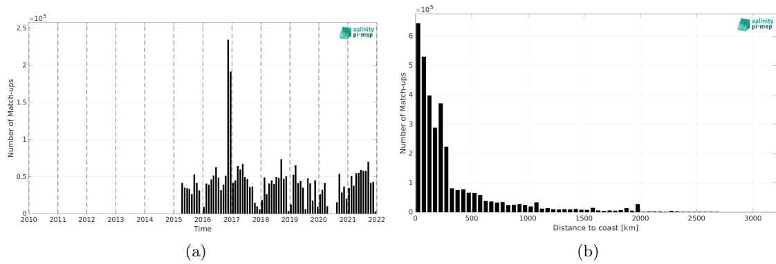
Figure 2: Number of match-ups between TSG (GOSUD-Research-vessel) and SMAP SSS L2 v5.3 (RSS) SSS as a function of time (a) and as function of the distance to coast (b) over the Global Ocean Pi-MEP region and for the full satellite product period.
