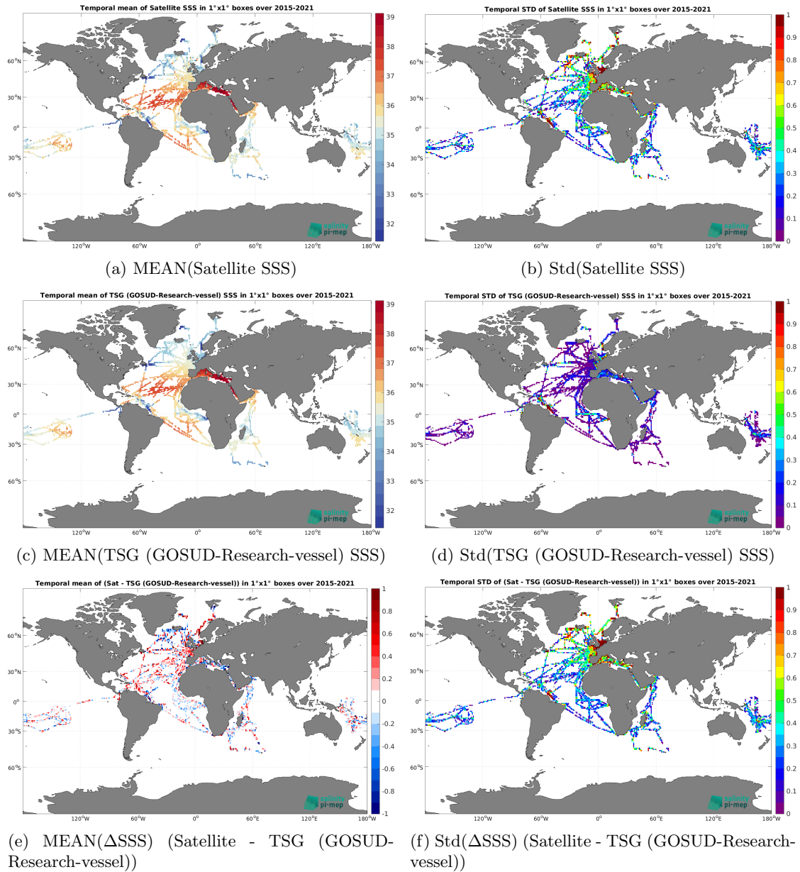
Figure 7: Temporal mean (left) and Std (right) of SSS from SMAP SSS L2 v5.3 (RSS) (top), TSG (GOSUD-Research-vessel) (middle), and of \Delta SSS (Satellite - TSG (GOSUD-Research-vessel)). Only match-up pairs are used to generate these maps.
