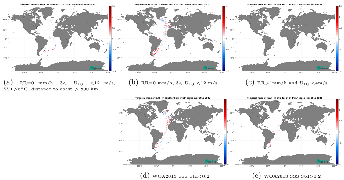
Figure 14: Temporal mean gridded over spatial boxes of size 1^\circ \times 1^\circ of \Delta SSS (SMAP SSS L2 v5.3 (RSS) - TSG (CSIC-UTM)) for 5 different subdatasets corresponding to:RR=0 mm/h, 3 < U_{10} < 12 m/s, SST > 5^\circ\text{C} , distance to coast > 800 km (a), RR=0 mm/h, 3 < U_{10} < 12 m/s (b), RR > 1 mm/h and U_{10} < 4 m/s (c), WOA2013 SSS Std < 0.2 (d), WOA2013 SSS Std > 0.2 (e).
