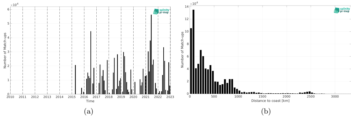
Figure 2: Number of match-ups between TSG (CSIC-UTM) and SMAP SSS L2 v5.3 (RSS) SSS as a function of time (a) and as function of the distance to coast (b) over the Global Ocean Pi-MEP region and for the full satellite product period.
