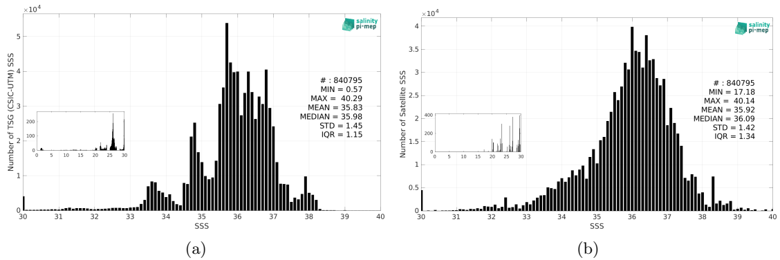
Figure 3: Histograms of SSS from TSG (CSIC-UTM) (a) and SMAP SSS L2 v5.3 (RSS) (b) considering all match-up pairs per bins of 0.1 over the Global Ocean Pi-MEP region and for the full satellite product period.
