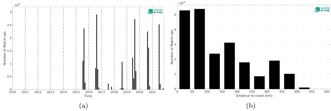
Figure 2: Number of match-ups between TSG (Amundsen) and SMAP SSS L2 v5.3 (RSS) SSS as a function of time (a) and as function of the distance to coast (b) over the Global Ocean Pi-MEP region and for the full satellite product period.
