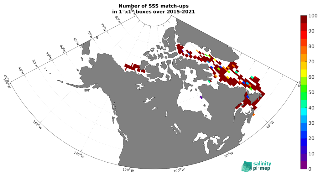
Figure 5: Number of SSS match-ups between TSG (Amundsen) SSS and the SMAP SSS L2 v5.3 (RSS) SSS product for the Global Ocean Pi-MEP region over 1^\circ \times 1^\circ boxes and for the full satellite product period.
