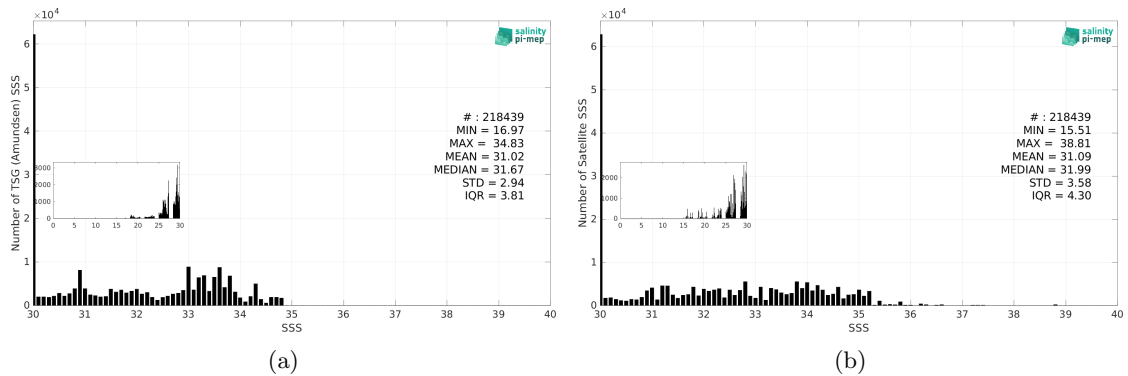
Figure 3: Histograms of SSS from TSG (Amundsen) (a) and SMAP SSS L2 v5.3 (RSS) (b) considering all match-up pairs per bins of 0.1 over the Global Ocean Pi-MEP region and for the full satellite product period.
