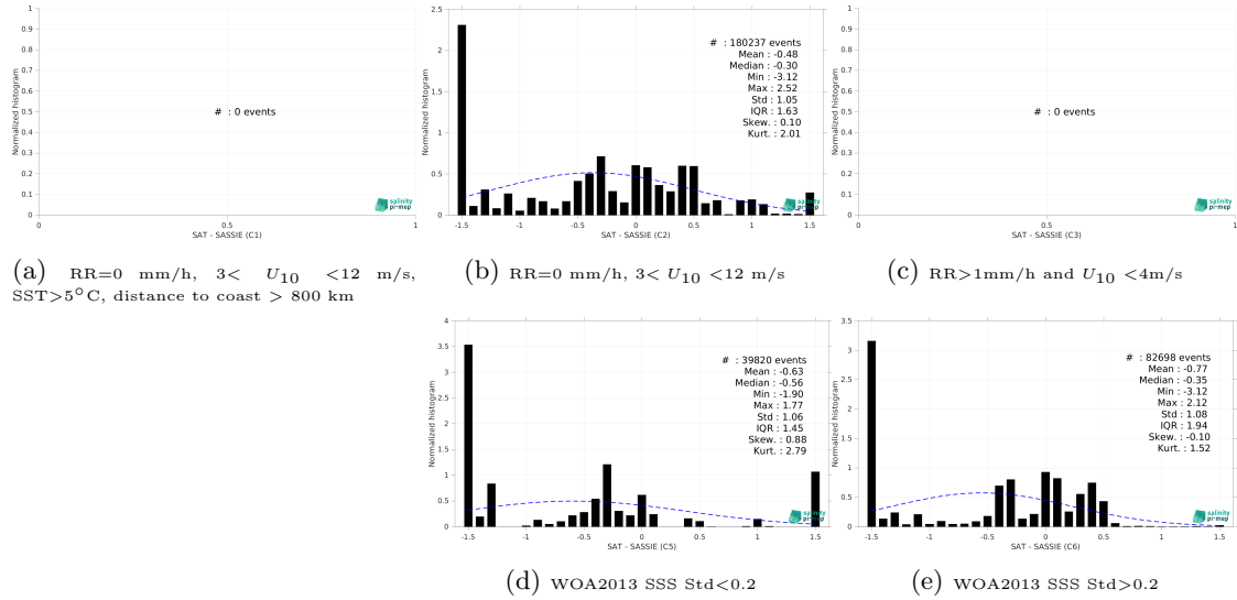
Figure 15: Normalized histogram of \Delta SSS (SMAP SSS L2 v5.3 (RSS) - SASSIE) for 5 different subdatasets corresponding to: RR=0 mm/h, 3 < U_{10} < 12 m/s, SST > 5°C, distance to coast > 800 km (a), RR=0 mm/h, 3 < U_{10} < 12 m/s (b), RR > 1mm/h and U_{10} < 4 m/s (c), WOA2013 SSS Std < 0.2 (d), WOA2013 SSS Std > 0.2 (e).
