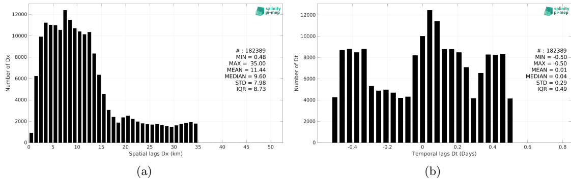
Figure 6: Histograms of the spatial (a) and temporal (b) lags between the location/time of the SASSIE measurement and the date of the corresponding SMAP SSS L2 v5.3 (RSS) SSS pixel.
