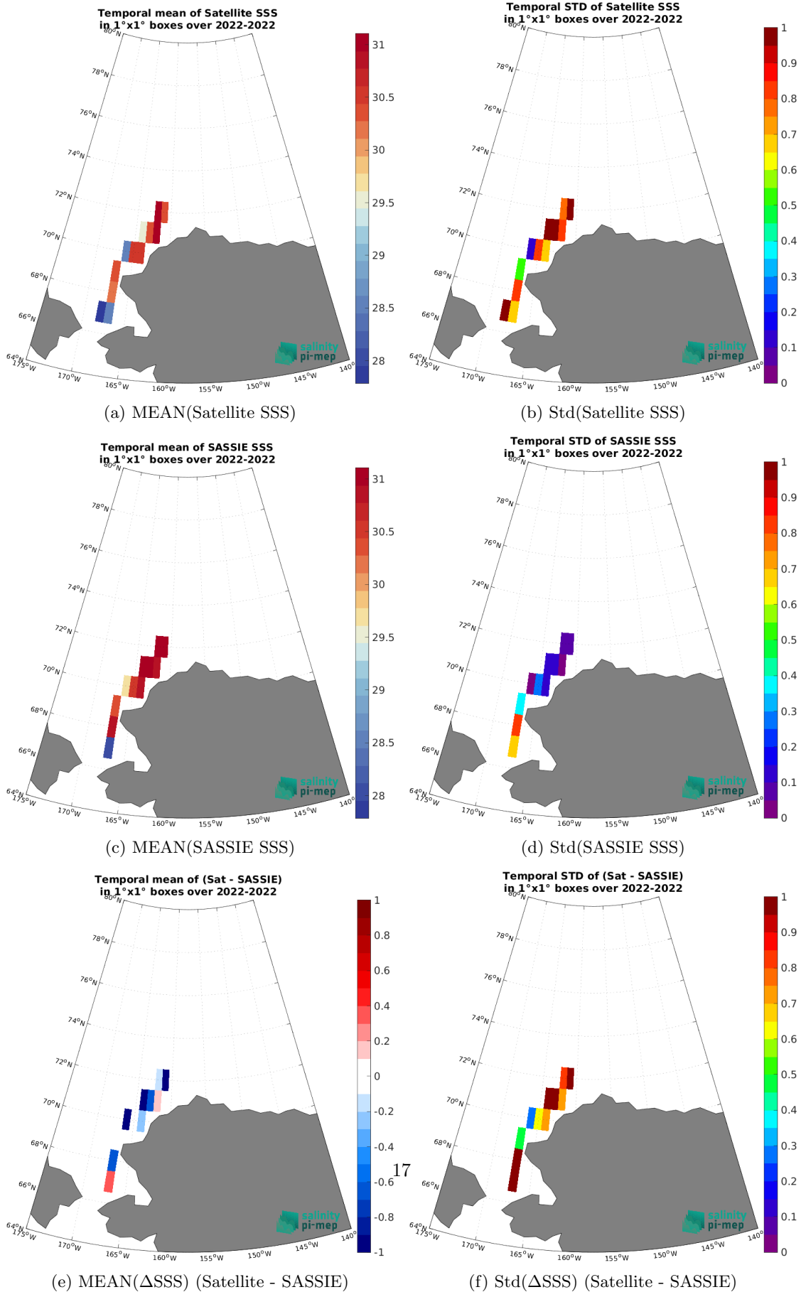
Figure 7: Temporal mean (left) and Std (right) of SSS from SMAP SSS L2 v5.3 (RSS) (top), SASSIE (middle), and of \Delta SSS (Satellite - SASSIE). Only match-up pairs are used to generate these maps.
