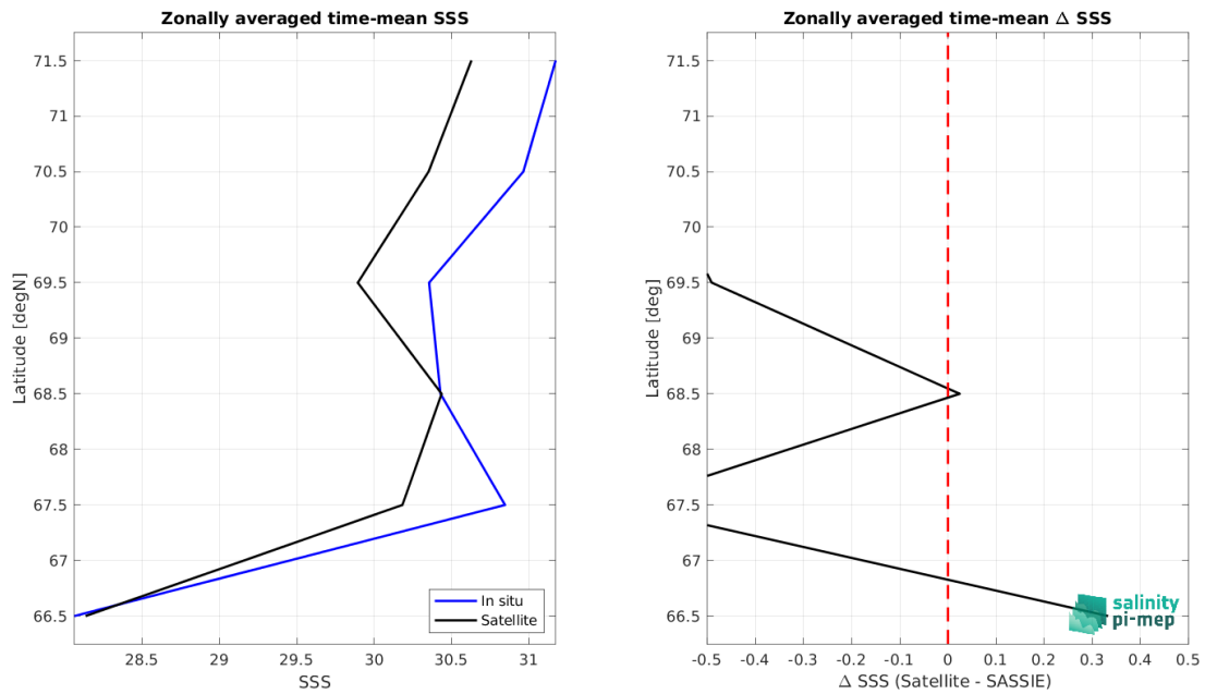
Figure 9: Left panel: Zonal mean SSS from SMAP SSS L2 v5.3 (RSS) satellite product (black) and from SASSIE (blue). Right panel: Zonal mean of \Delta SSS (Satellite - SASSIE) for all the collected Pi-MEP match-up pairs estimated over the full satellite product period.
