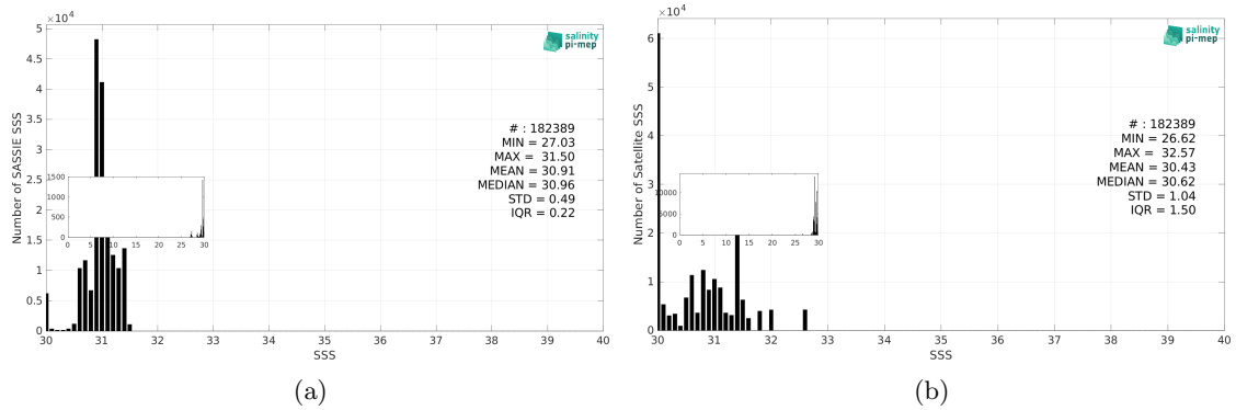
Figure 3: Histograms of SSS from SASSIE (a) and SMAP SSS L2 v5.3 (RSS) (b) considering all match-up pairs per bins of 0.1 over the Global Ocean Pi-MEP region and for the full satellite product period.
