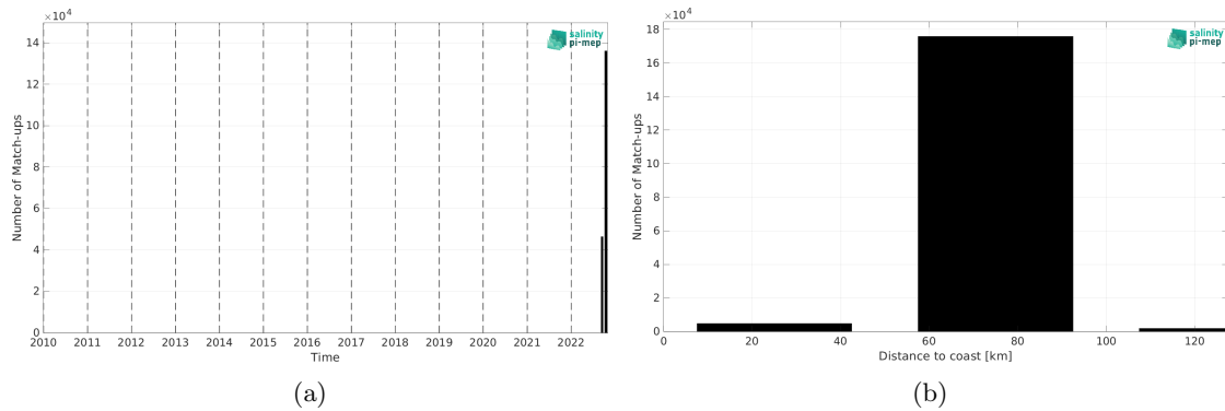
Figure 2: Number of match-ups between SASSIE and SMAP SSS L2 v5.3 (RSS) SSS as a function of time (a) and as function of the distance to coast (b) over the Global Ocean Pi-MEP region and for the full satellite product period.
