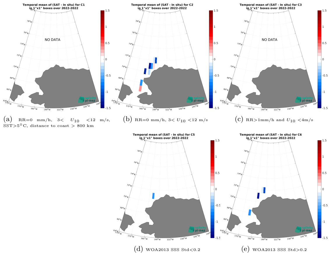
Figure 14: Temporal mean gridded over spatial boxes of size 1^\circ \times 1^\circ of \Delta\text{SSS} (SMAP SSS L2 v5.3 (RSS) - SASSIE) for 5 different subdatasets corresponding to:RR=0 mm/h, 3 < U_{10} < 12 m/s, SST>5°C, distance to coast > 800 km (a), RR=0 mm/h, 3 < U_{10} < 12 m/s (b), RR>1mm/h and U_{10} < 4 m/s (c), WOA2013 SSS Std<0.2 (d), WOA2013 SSS Std>0.2 (e).
