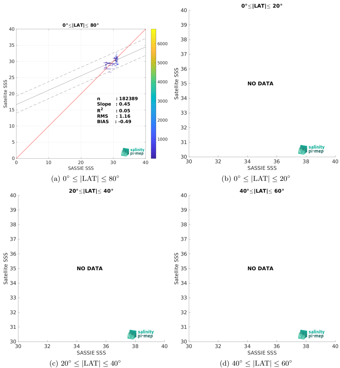
Figure 10: Contour maps of the concentration of SMAP SSS L2 v5.3 (RSS) SSS (y-axis) versus SASSIE SSS (x-axis) at match-up pairs for different latitude bands. For each plot, the red line shows x=y . The black thin and dashed lines indicate a linear fit through the data cloud and the \pm 95\% confidence levels, respectively. The number match-up pairs n , the slope and R^2 coefficient of the linear fit, the root mean square (RMS) and the mean bias between satellite and in situ data are indicated for each latitude band in each plots.
