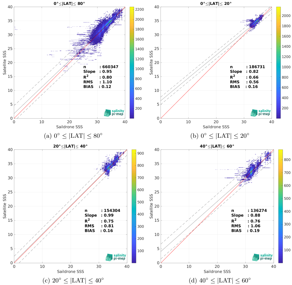
Figure 10: Contour maps of the concentration of SMAP SSS L2 v5.3 (RSS) SSS (y-axis) versus Saildrone SSS (x-axis) at match-up pairs for different latitude bands. For each plot, the red line shows x=y . The black thin and dashed lines indicate a linear fit through the data cloud and the \pm 95\% confidence levels, respectively. The number match-up pairs n , the slope and R^2 coefficient of the linear fit, the root mean square (RMS) and the mean bias between satellite and in situ data are indicated for each latitude band in each plots.
