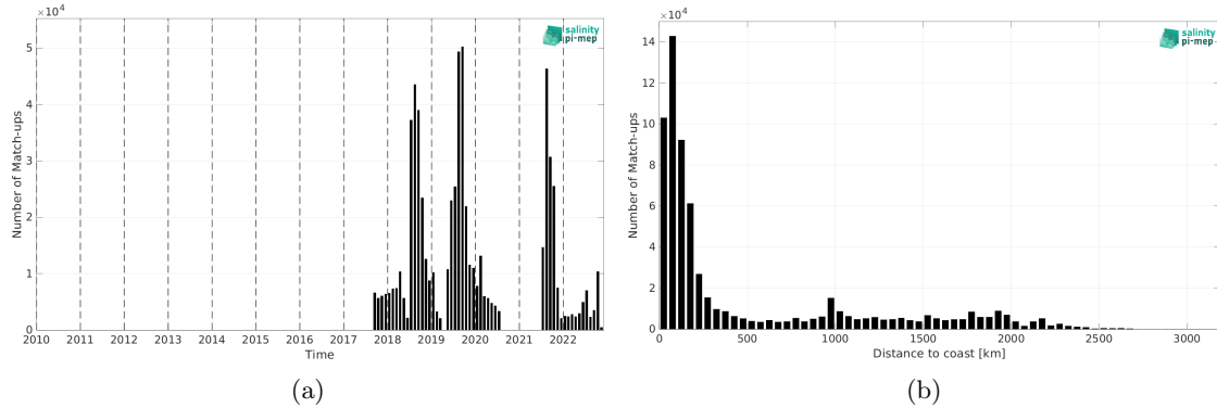
Figure 2: Number of match-ups between Saildrone and SMAP SSS L2 v5.3 (RSS) SSS as a function of time (a) and as function of the distance to coast (b) over the Global Ocean Pi-MEP region and for the full satellite product period.
