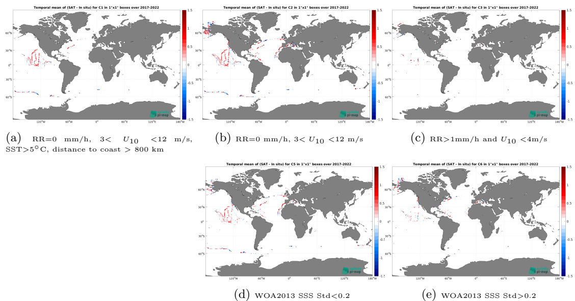
Figure 14: Temporal mean gridded over spatial boxes of size 1^\circ \times 1^\circ of \Delta SSS (SMAP SSS L2 v5.3 (RSS) - Saldrone) for 5 different subdatasets corresponding to:RR=0 mm/h, 3 < U_{10} < 12 m/s, SST > 5^\circ\text{C} , distance to coast > 800 km (a), RR=0 mm/h, 3 < U_{10} < 12 m/s (b), RR > 1 mm/h and U_{10} < 4 m/s (c), WOA2013 SSS Std < 0.2 (d), WOA2013 SSS Std > 0.2 (e).
