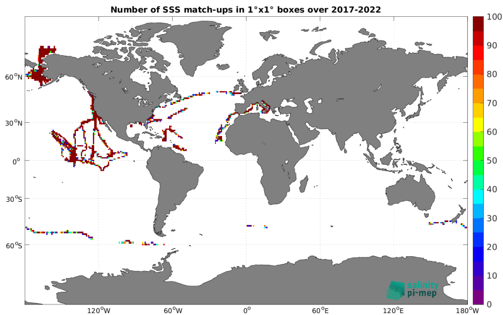
Figure 5: Number of SSS match-ups between Saildrone SSS and the SMAP SSS L2 v5.3 (RSS) SSS product for the Global Ocean Pi-MEP region over 1^\circ \times 1^\circ boxes and for the full satellite product period.
