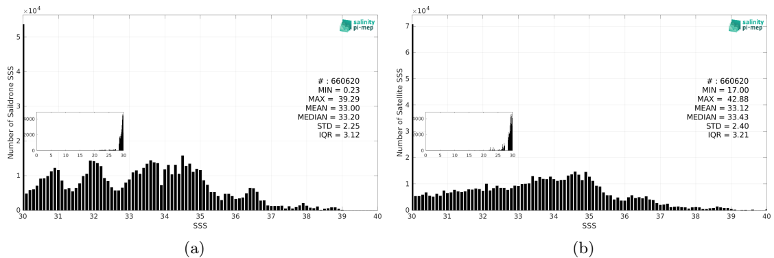
Figure 3: Histograms of SSS from Saildrone (a) and SMAP SSS L2 v5.3 (RSS) (b) considering all match-up pairs per bins of 0.1 over the Global Ocean Pi-MEP region and for the full satellite product period.
