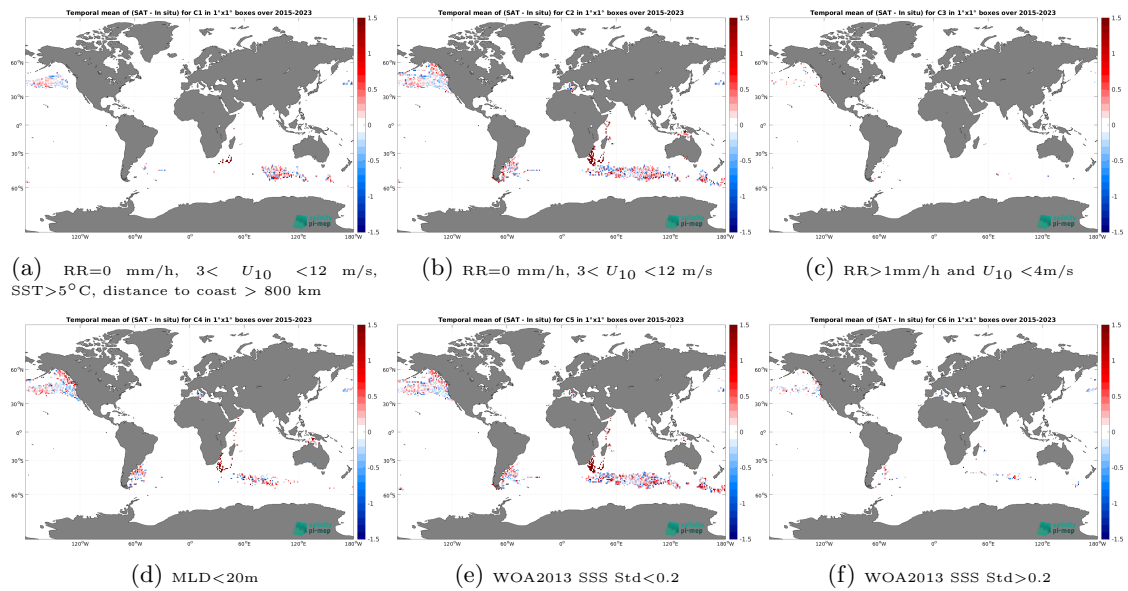
Figure 14: Temporal mean gridded over spatial boxes of size 1^\circ \times 1^\circ of \Delta SSS (SMAP SSS L2 v5.3 (RSS) - Marine mammals) for 6 different subdatasets corresponding to:RR=0 mm/h, 3 < U_{10} < 12 m/s, SST >5^\circ C, distance to coast > 800 km (a), RR=0 mm/h, 3 < U_{10} < 12 m/s (b), RR >1 mm/h and U_{10} < 4 m/s (c),MLD <20 m (d),WOA2013 SSS Std <0.2 (e),WOA2013 SSS Std >0.2 (f).
