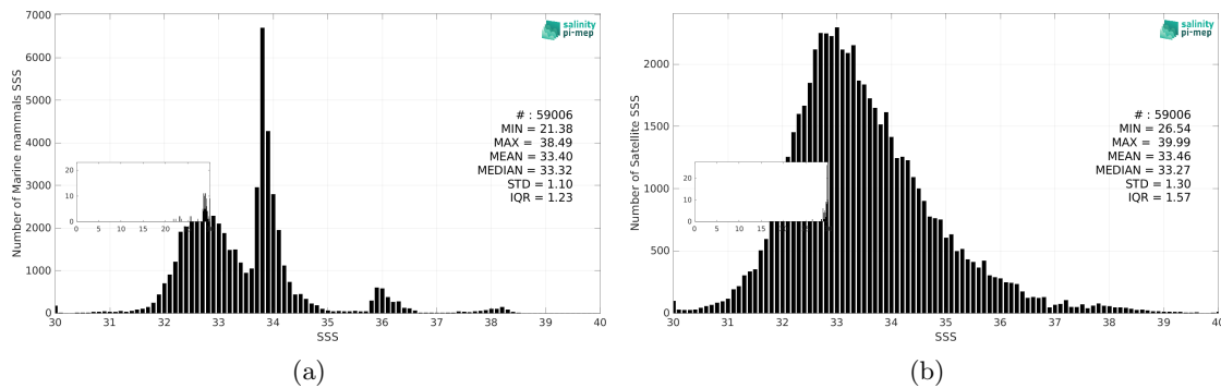
Figure 3: Histograms of SSS from Marine mammals (a) and SMAP SSS L2 v5.3 (RSS) (b) considering all match-up pairs per bins of 0.1 over the Global Ocean Pi-MEP region and for the full satellite product period.
