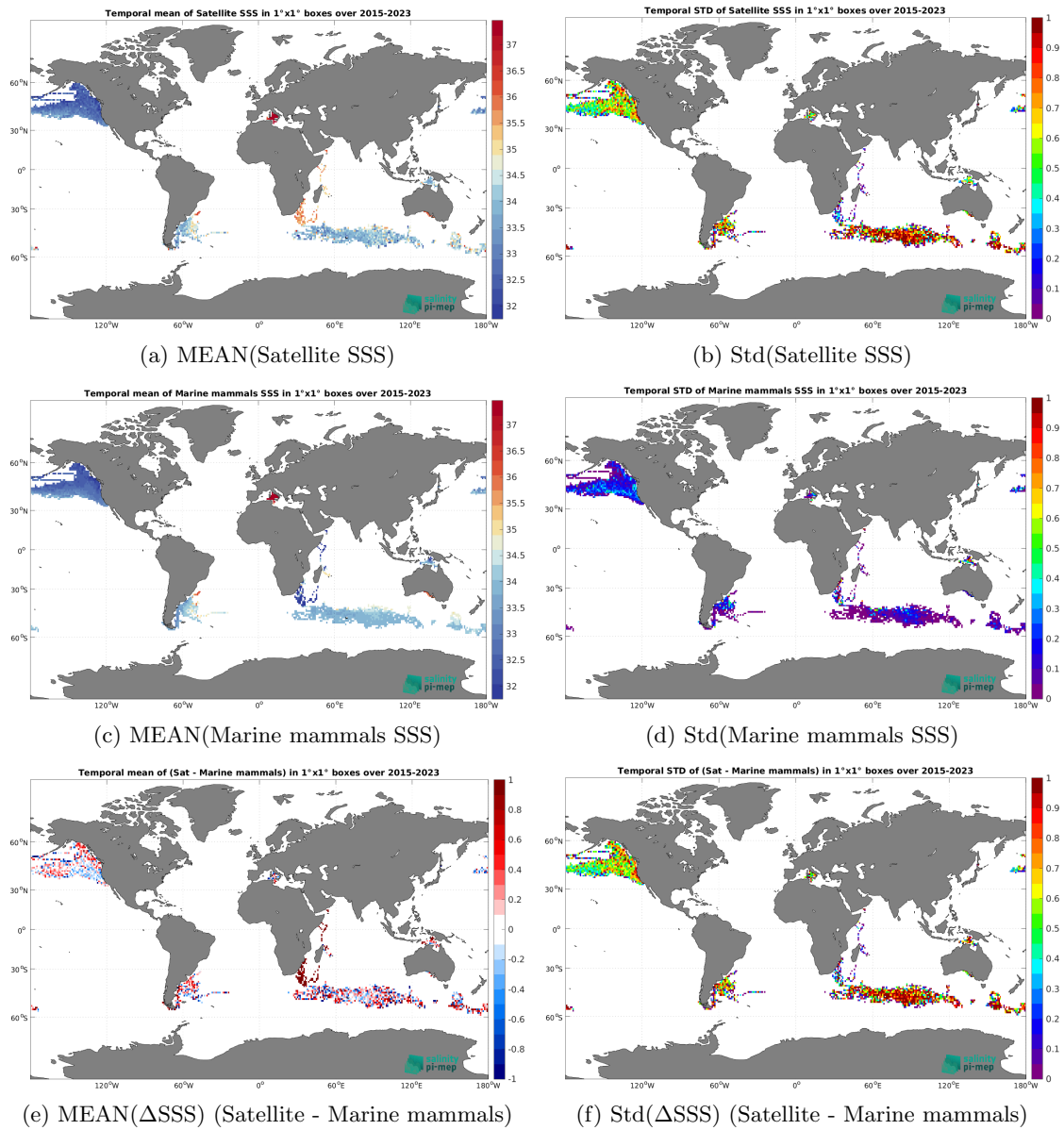
Figure 7: Temporal mean (left) and Std (right) of SSS from SMAP SSS L2 v5.3 (RSS) (top), Marine mammals (middle), and of \Delta SSS (Satellite - Marine mammals). Only match-up pairs are used to generate these maps.
