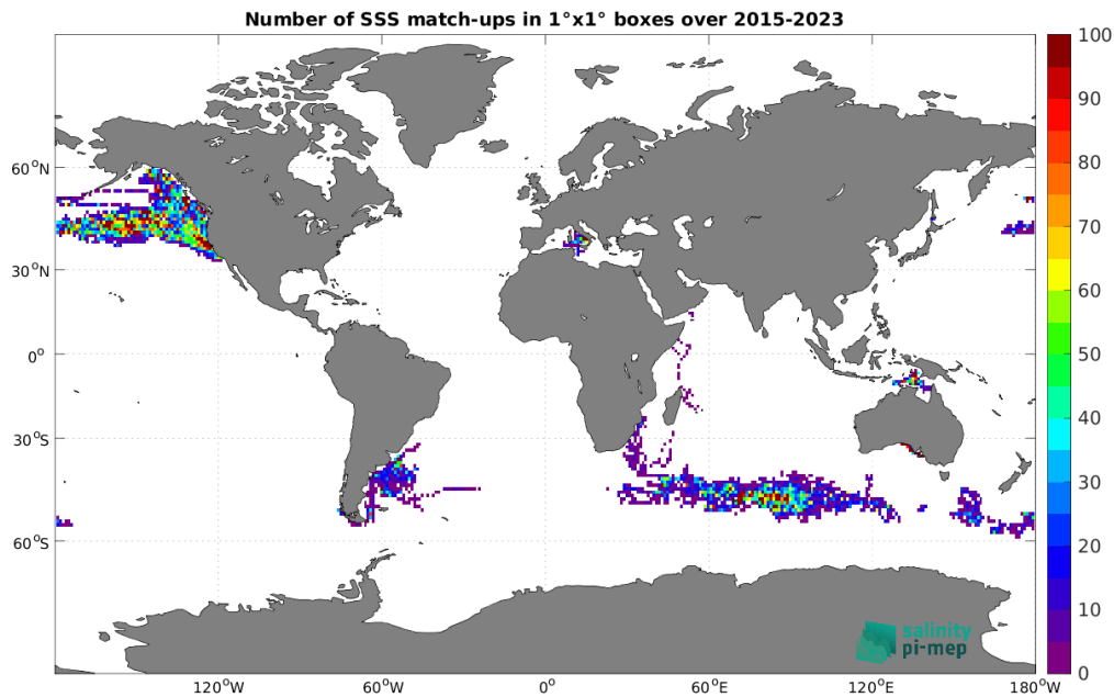
Figure 5: Number of SSS match-ups between Marine mammals SSS and the SMAP SSS L2 v5.3 (RSS) SSS product for the Global Ocean Pi-MEP region over 1^\circ \times 1^\circ boxes and for the full satellite product period.
