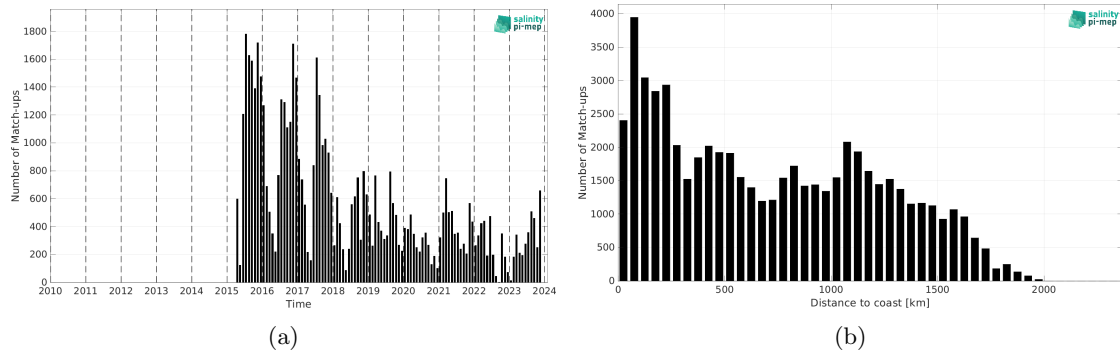
Figure 2: Number of match-ups between Marine mammals and SMAP SSS L2 v5.3 (RSS) SSS as a function of time (a) and as function of the distance to coast (b) over the Global Ocean Pi-MEP region and for the full satellite product period.
