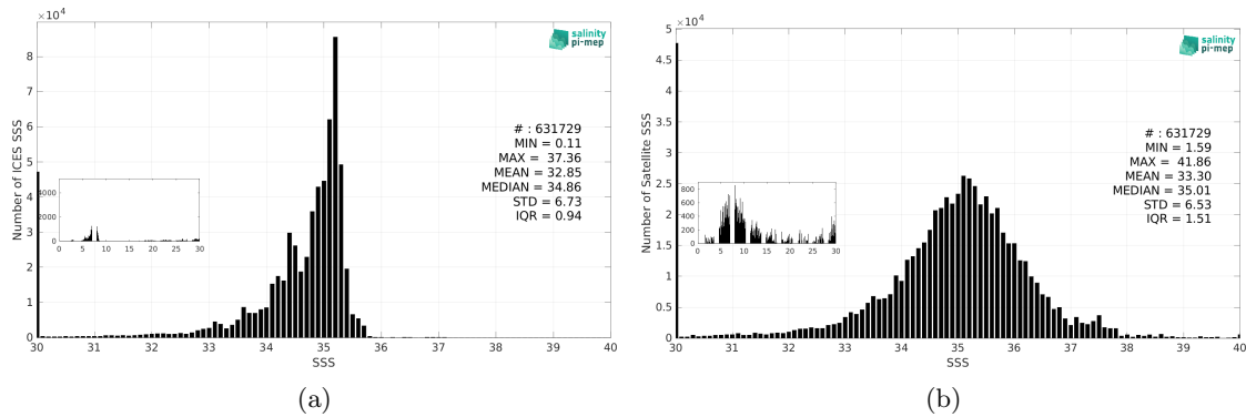
Figure 3: Histograms of SSS from ICES (a) and SMAP SSS L2 v5.3 (RSS) (b) considering all match-up pairs per bins of 0.1 over the Global Ocean Pi-MEP region and for the full satellite product period.
