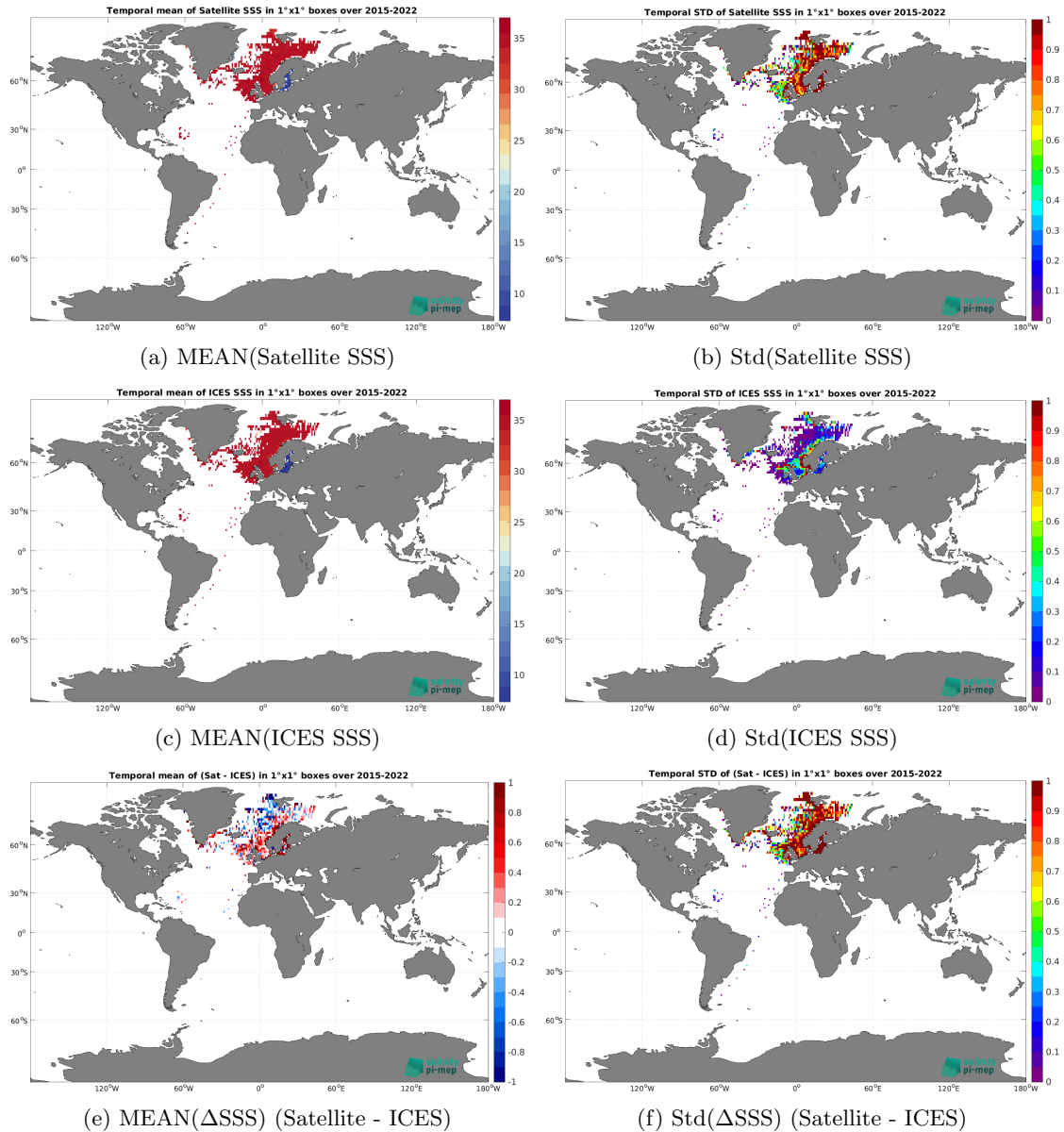
Figure 7: Temporal mean (left) and Std (right) of SSS from SMAP SSS L2 v5.3 (RSS) (top), ICES (middle), and of \Delta SSS (Satellite - ICES). Only match-up pairs are used to generate these maps.
