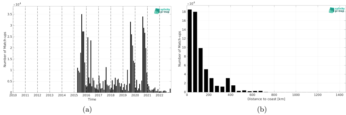
Figure 2: Number of match-ups between ICES and SMAP SSS L2 v5.3 (RSS) SSS as a function of time (a) and as function of the distance to coast (b) over the Global Ocean Pi-MEP region and for the full satellite product period.
