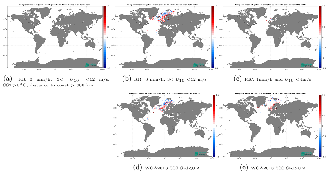
Figure 14: Temporal mean gridded over spatial boxes of size 1^\circ \times 1^\circ of \Delta SSS (SMAP SSS L2 v5.3 (RSS) - ICES) for 5 different subdatasets corresponding to:RR=0 mm/h, 3 < U_{10} < 12 m/s, SST > 5^\circ\text{C} , distance to coast > 800 km (a), RR=0 mm/h, 3 < U_{10} < 12 m/s (b), RR > 1 mm/h and U_{10} < 4 m/s (c), WOA2013 SSS Std < 0.2 (d), WOA2013 SSS Std > 0.2 (e).
