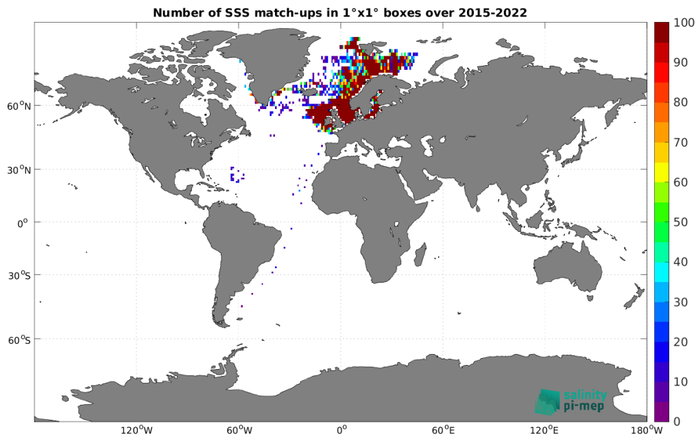
Figure 5: Number of SSS match-ups between ICES SSS and the SMAP SSS L2 v5.3 (RSS) SSS product for the Global Ocean Pi-MEP region over 1^\circ \times 1^\circ boxes and for the full satellite product period.
