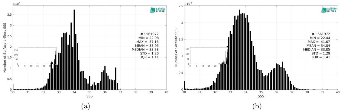
Figure 3: Histograms of SSS from Surface drifters (a) and SMAP SSS L2 v5.3 (RSS) (b) considering all match-up pairs per bins of 0.1 over the Global Ocean Pi-MEP region and for the full satellite product period.
