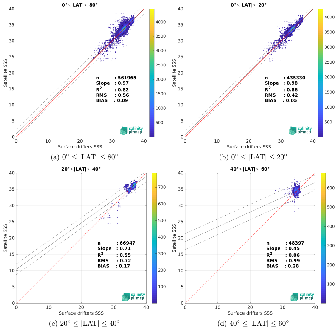
Figure 9: Contour maps of the concentration of SMAP SSS L2 v5.3 (RSS) SSS (y-axis) versus Surface drifters SSS (x-axis) at match-up pairs for different latitude bands. For each plot, the red line shows x=y . The black thin and dashed lines indicate a linear fit through the data cloud and the \pm 95\% confidence levels, respectively. The number match-up pairs n , the slope and R^2 coefficient of the linear fit, the root mean square (RMS) and the mean bias between satellite and in situ data are indicated for each latitude band in each plots.
