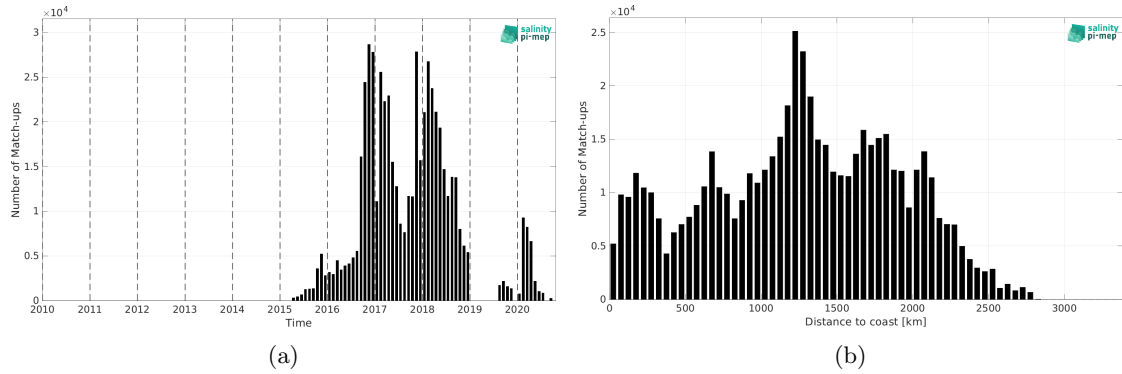
Figure 2: Number of match-ups between Surface drifters and SMAP SSS L2 v5.3 (RSS) SSS as a function of time (a) and as function of the distance to coast (b) over the Global Ocean Pi-MEP region and for the full satellite product period.
