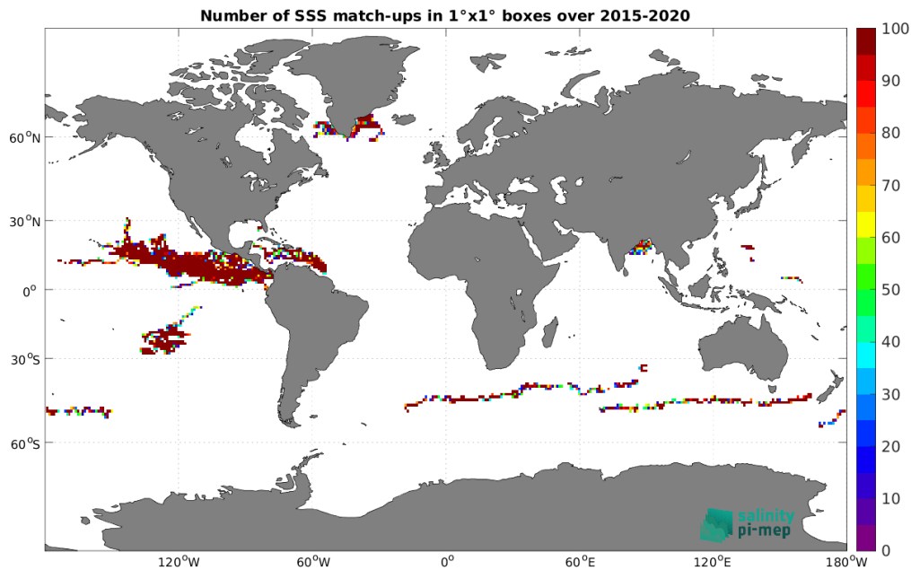
Figure 4: Number of SSS match-ups between Surface drifters SSS and the SMAP SSS L2 v5.3 (RSS) SSS product for the Global Ocean Pi-MEP region over 1^\circ \times 1^\circ boxes and for the full satellite product period.
