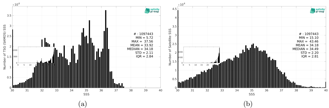
Figure 3: Histograms of SSS from TSG (SAMOS) (a) and SMAP SSS L2 v5.3 - 40 km (RSS) (b) considering all match-up pairs per bins of 0.1 over the Global Ocean Pi-MEP region and for the full satellite product period.
