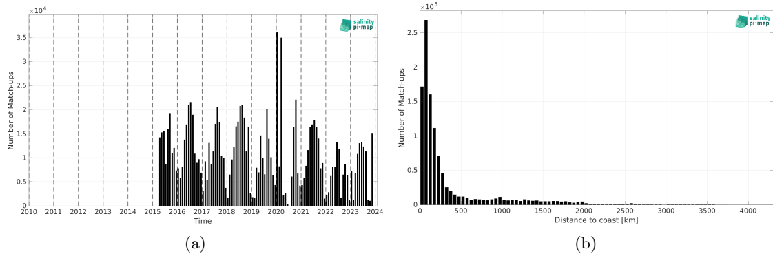
Figure 2: Number of match-ups between TSG (SAMOS) and SMAP SSS L2 v5.3 - 40 km (RSS) SSS as a function of time (a) and as function of the distance to coast (b) over the Global Ocean Pi-MEP region and for the full satellite product period.
