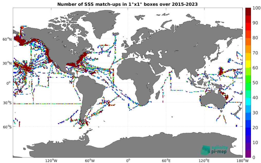
Figure 5: Number of SSS match-ups between TSG (SAMOS) SSS and the SMAP SSS L2 v5.3 - 40 km (RSS) SSS product for the Global Ocean Pi-MEP region over 1^\circ \times 1^\circ boxes and for the full satellite product period.
