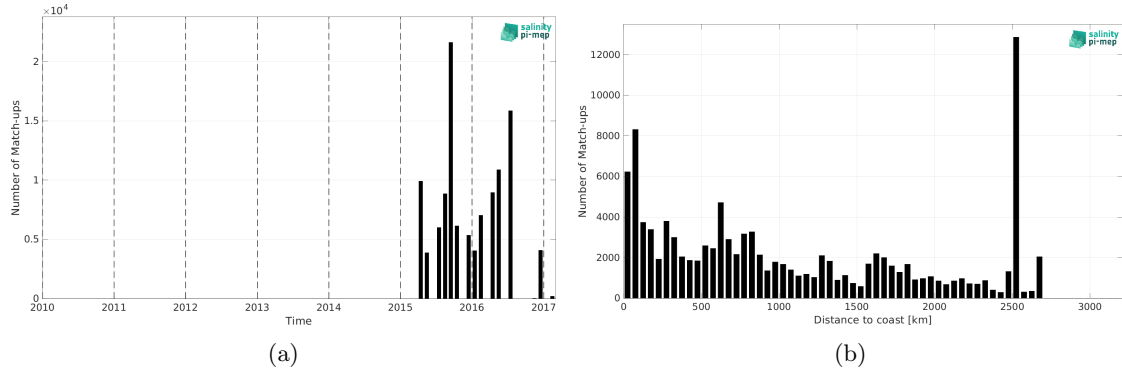
Figure 2: Number of match-ups between TSG (NCEI-0170743) and SMAP SSS L2 v5.3 - 40 km (RSS) SSS as a function of time (a) and as function of the distance to coast (b) over the Global Ocean Pi-MEP region and for the full satellite product period.
