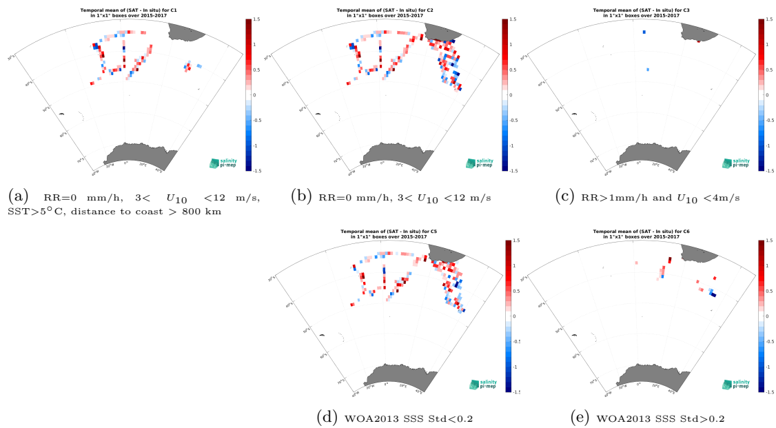
Figure 14: Temporal mean gridded over spatial boxes of size 1^\circ \times 1^\circ of \Delta SSS (SMAP SSS L2 v5.3 - 40 km (RSS) - TSG (NCEI-0170743)) for 5 different subdatasets corresponding to:RR=0 mm/h, 3 < U_{10} < 12 m/s, SST >5^\circ\text{C} , distance to coast > 800 km (a), RR=0 mm/h, 3 < U_{10} < 12 m/s (b), RR >1 mm/h and U_{10} < 4 m/s (c), WOA2013 SSS Std <0.2 (d), WOA2013 SSS Std >0.2 (e).
