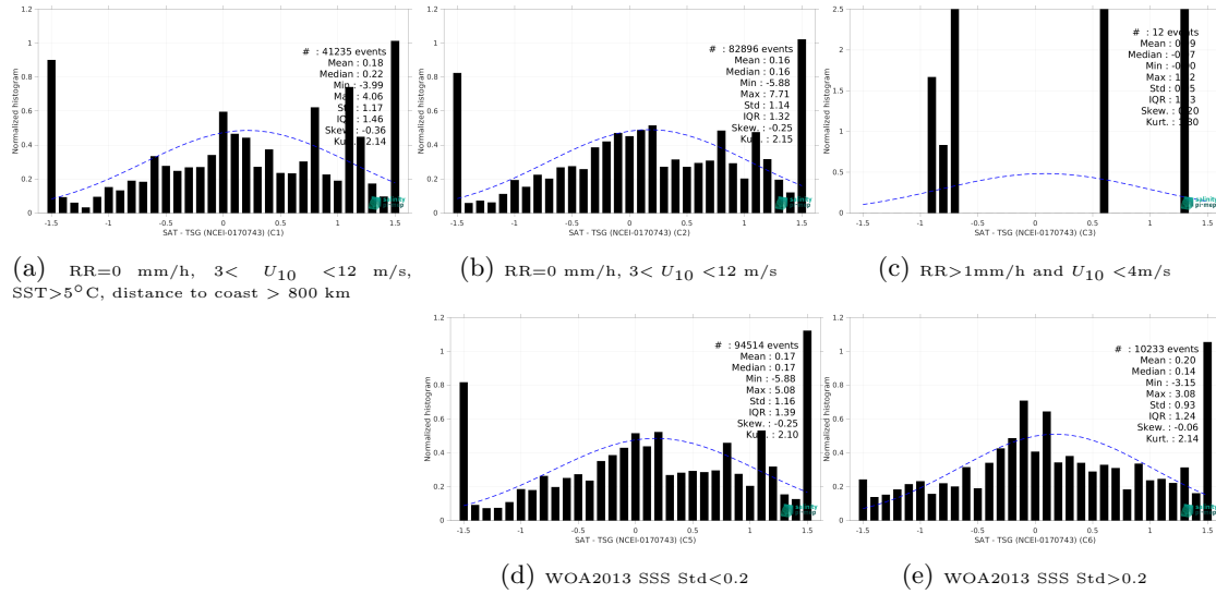
Figure 15: Normalized histogram of \Delta SSS (SMAP SSS L2 v5.3 - 40 km (RSS) - TSG (NCEI-0170743)) for 5 different subdatasets corresponding to: RR=0 mm/h, 3 < U_{10} < 12 m/s, SST > 5°C, distance to coast > 800 km (a), RR=0 mm/h, 3 < U_{10} < 12 m/s (b), RR > 1mm/h and U_{10} < 4 m/s (c), WOA2013 SSS Std < 0.2 (d), WOA2013 SSS Std > 0.2 (e).
