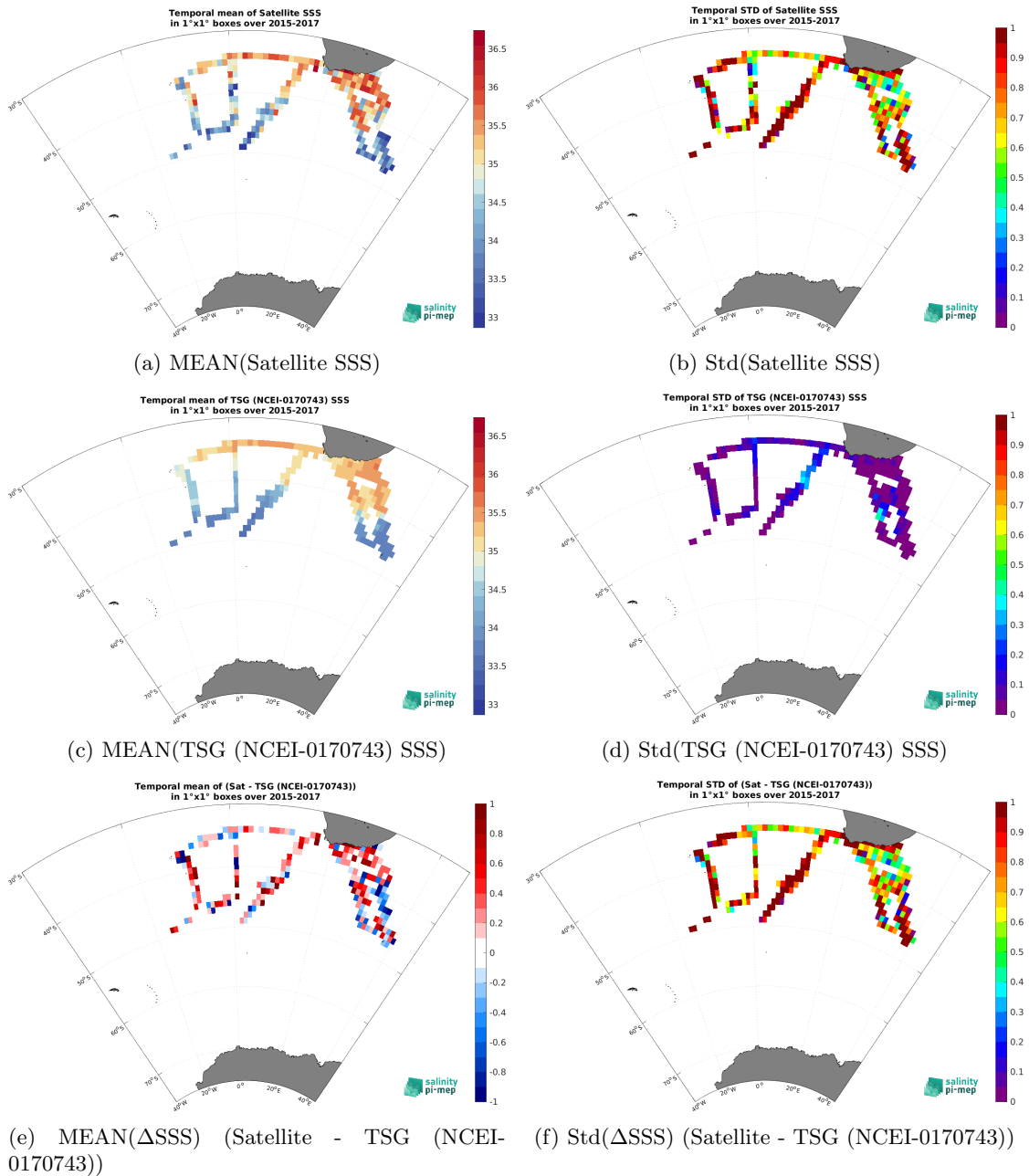
Figure 7: Temporal mean (left) and Std (right) of SSS from SMAP SSS L2 v5.3 - 40 km (RSS) (top), TSG (NCEI-0170743) (middle), and of \Delta SSS (Satellite - TSG (NCEI-0170743)). Only match-up pairs are used to generate these maps.
