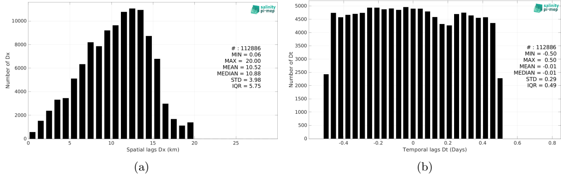
Figure 6: Histograms of the spatial (a) and temporal (b) lags between the location/time of the TSG (NCEI-0170743) measurement and the date of the corresponding SMAP SSS L2 v5.3 - 40 km (RSS) SSS pixel.
