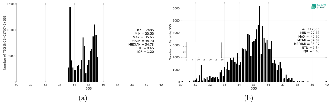
Figure 3: Histograms of SSS from TSG (NCEI-0170743) (a) and SMAP SSS L2 v5.3 - 40 km (RSS) (b) considering all match-up pairs per bins of 0.1 over the Global Ocean Pi-MEP region and for the full satellite product period.
