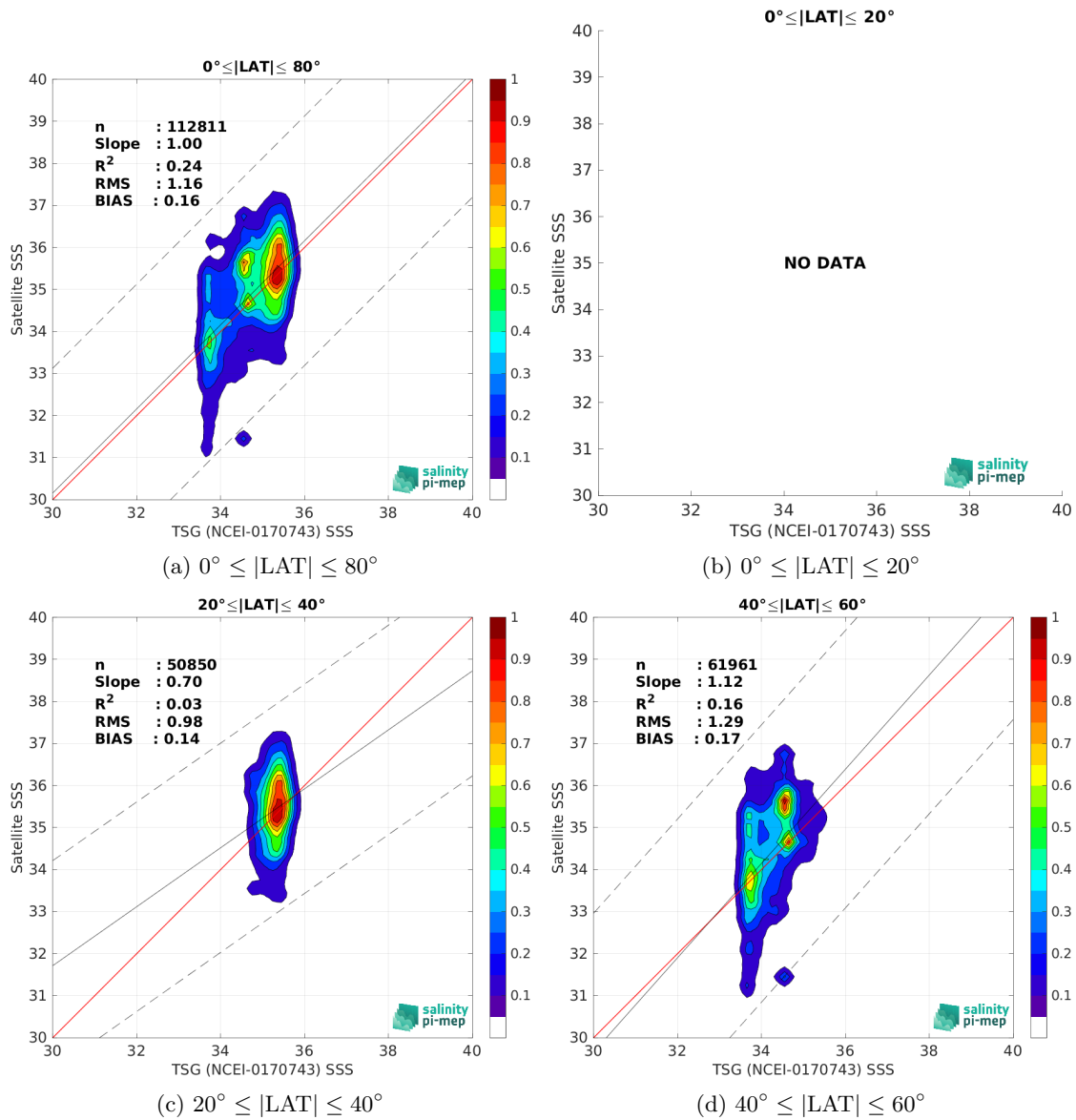
Figure 10: Contour maps of the concentration of SMAP SSS L2 v5.3 - 40 km (RSS) SSS (y-axis) versus TSG (NCEI-0170743) SSS (x-axis) at match-up pairs for different latitude bands. For each plot, the red line shows x=y . The black thin and dashed lines indicate a linear fit through the data cloud and the \pm 95\% confidence levels, respectively. The number match-up pairs n , the slope and R^2 coefficient of the linear fit, the root mean square (RMS) and the mean bias between satellite and in situ data are indicated for each latitude band in each plots.
