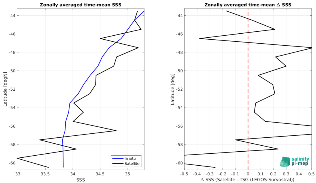
Figure 9: Left panel: Zonal mean SSS from SMAP SSS L2 v5.3 - 40 km (RSS) satellite product (black) and from TSG (LEGOS-Survostral) (blue). Right panel: Zonal mean of \Delta SSS (Satellite - TSG (LEGOS-Survostral)) for all the collected Pi-MEP match-up pairs estimated over the full satellite product period.
