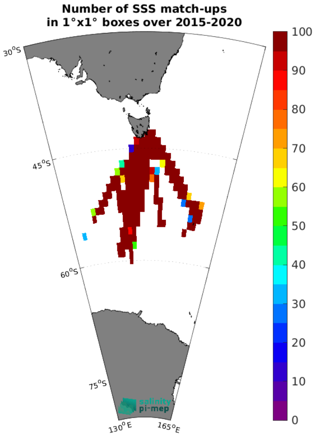
Figure 5: Number of SSS match-ups between TSG (LEGOS-Survostral) SSS and the SMAP SSS L2 v5.3 - 40 km (RSS) SSS product for the Global Ocean Pi-MEP region over 1°×1° boxes and for the full satellite product period.
