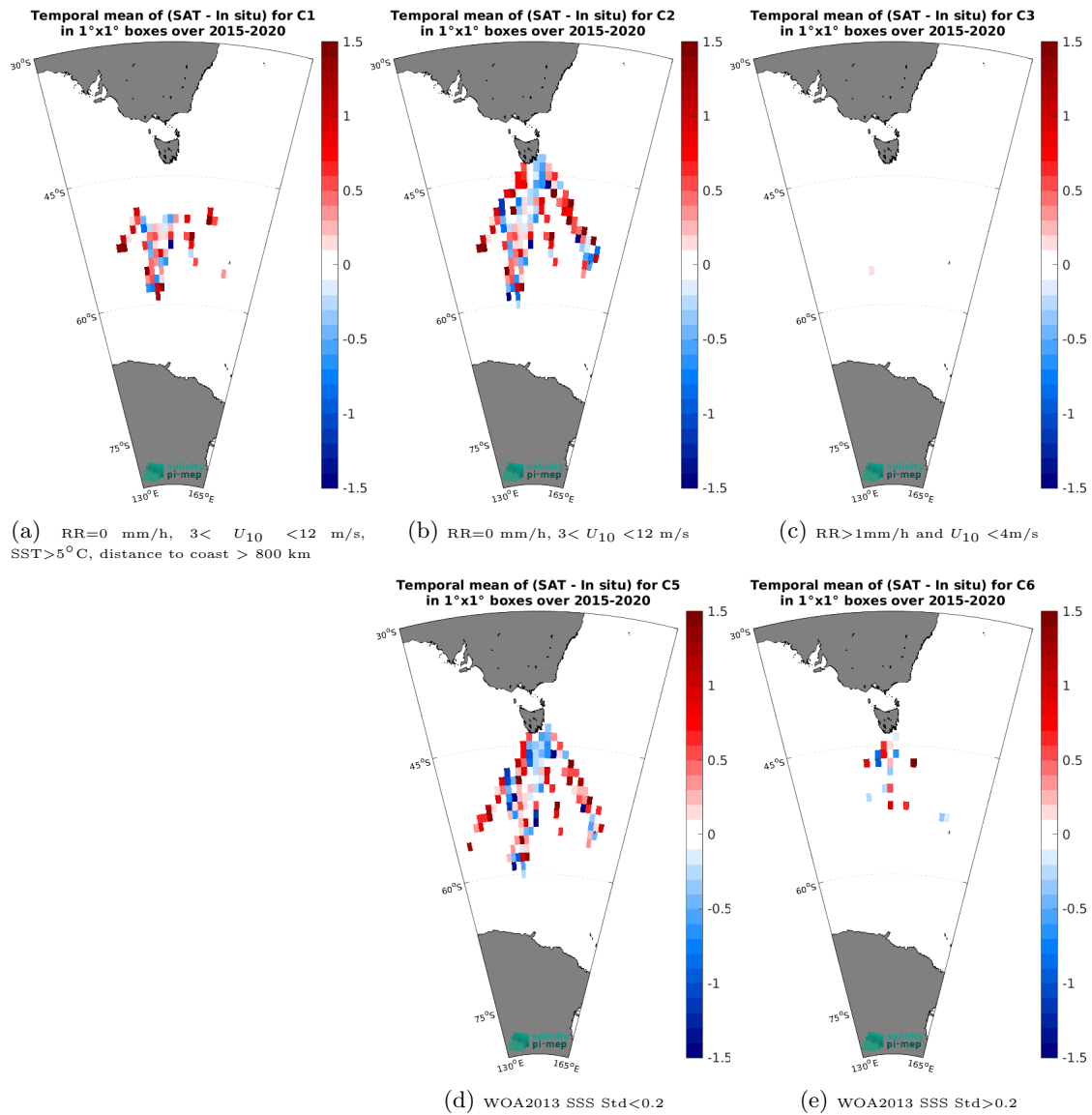
Figure 14: Temporal mean gridded over spatial boxes of size 1^\circ \times 1^\circ of \Delta\text{SSS} (SMAP SSS L2 v5.3 - 40 km (RSS) - TSG (LEGOS-Survostral)) for 5 different subdatasets corresponding to: RR=0 mm/h, 3 < U_{10} < 12 m/s, SST > 5^\circ\text{C} , distance to coast > 800 km (a), RR=0 mm/h, 3 < U_{10} < 12 m/s (b), RR > 1 mm/h and U_{10} < 4 m/s (c), WOA2013 SSS Std < 0.2 (d), WOA2013 SSS Std > 0.2 (e).
