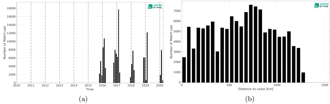
Figure 2: Number of match-ups between TSG (LEGOS-Survostral) and SMAP SSS L2 v5.3 - 40 km (RSS) SSS as a function of time (a) and as function of the distance to coast (b) over the Global Ocean Pi-MEP region and for the full satellite product period.
