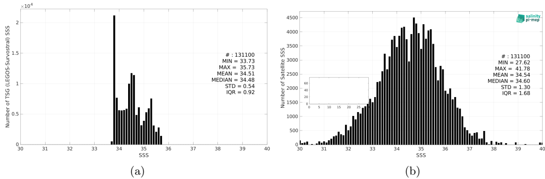
Figure 3: Histograms of SSS from TSG (LEGOS-Survostral) (a) and SMAP SSS L2 v5.3 - 40 km (RSS) (b) considering all match-up pairs per bins of 0.1 over the Global Ocean Pi-MEP region and for the full satellite product period.
