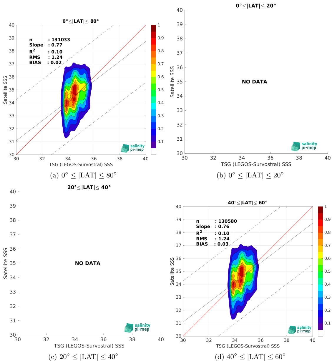
Figure 10: Contour maps of the concentration of SMAP SSS L2 v5.3 - 40 km (RSS) SSS (y-axis) versus TSG (LEGOS-Survostral) SSS (x-axis) at match-up pairs for different latitude bands. For each plot, the red line shows x=y . The black thin and dashed lines indicate a linear fit through the data cloud and the \pm 95\% confidence levels, respectively. The number match-up pairs n , the slope and R^2 coefficient of the linear fit, the root mean square (RMS) and the mean bias between satellite and in situ data are indicated for each latitude band in each plot.
