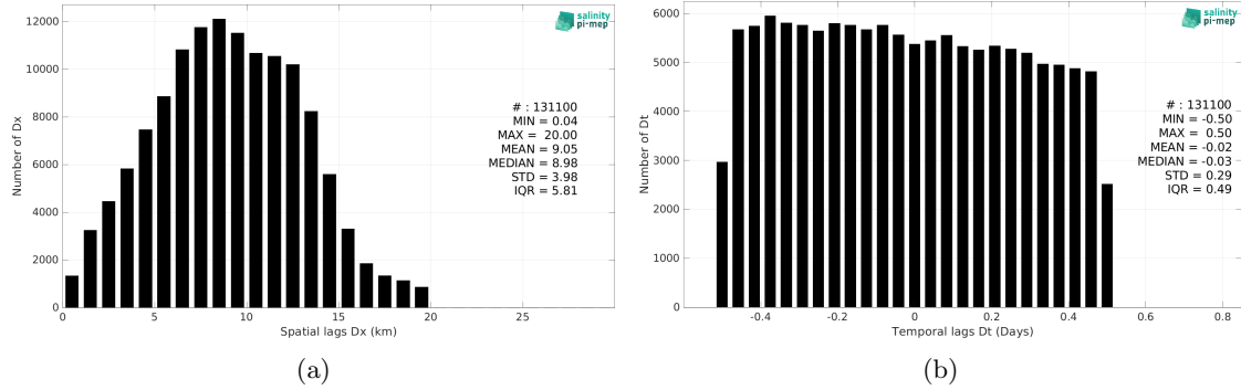
Figure 6: Histograms of the spatial (a) and temporal (b) lags between the location/time of the TSG (LEGOS-Survostral) measurement and the date of the corresponding SMAP SSS L2 v5.3 - 40 km (RSS) SSS pixel.
