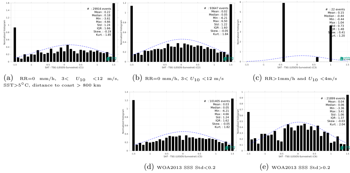
Figure 15: Normalized histogram of \Delta SSS (SMAP SSS L2 v5.3 - 40 km (RSS) - TSG (LEGOs-Survostral)) for 5 different subdatasets corresponding to: RR=0 mm/h, 3 < U_{10} < 12 m/s, SST > 5°C, distance to coast > 800 km (a), RR=0 mm/h, 3 < U_{10} < 12 m/s (b), RR > 1mm/h and U_{10} < 4 m/s (c), WOA2013 SSS Std < 0.2 (d), WOA2013 SSS Std > 0.2 (e).
