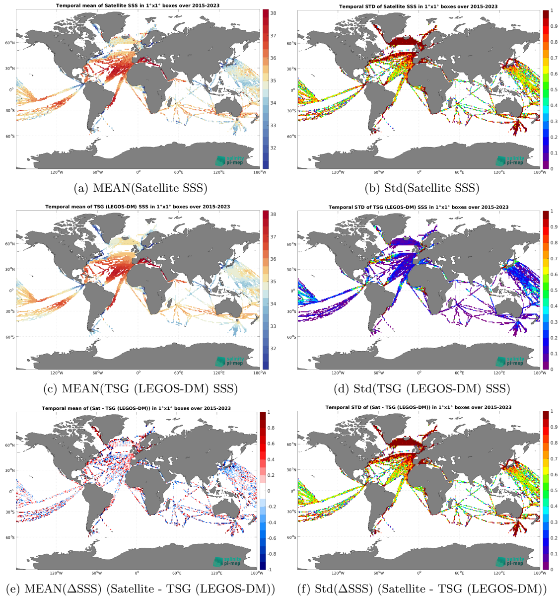
Figure 7: Temporal mean (left) and Std (right) of SSS from SMAP SSS L2 v5.3 - 40 km (RSS) (top), TSG (LEGOS-DM) (middle), and of \Delta SSS (Satellite - TSG (LEGOS-DM)). Only match-pair are used to generate these maps.
