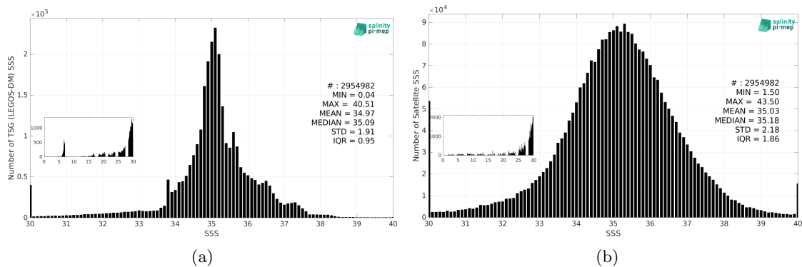
Figure 3: Histograms of SSS from TSG (LEGOS-DM) (a) and SMAP SSS L2 v5.3 - 40 km (RSS) (b) considering all match-up pairs per bins of 0.1 over the Global Ocean Pi-MEP region and for the full satellite product period.
