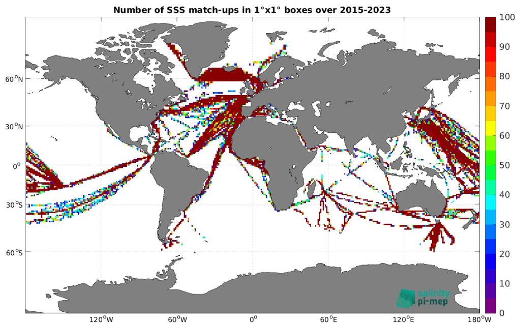
Figure 5: Number of SSS match-ups between TSG (LEGOS-DM) SSS and the SMAP SSS L2 v5.3 - 40 km (RSS) SSS product for the Global Ocean Pi-MEP region over 1^\circ \times 1^\circ boxes and for the full satellite product period.
