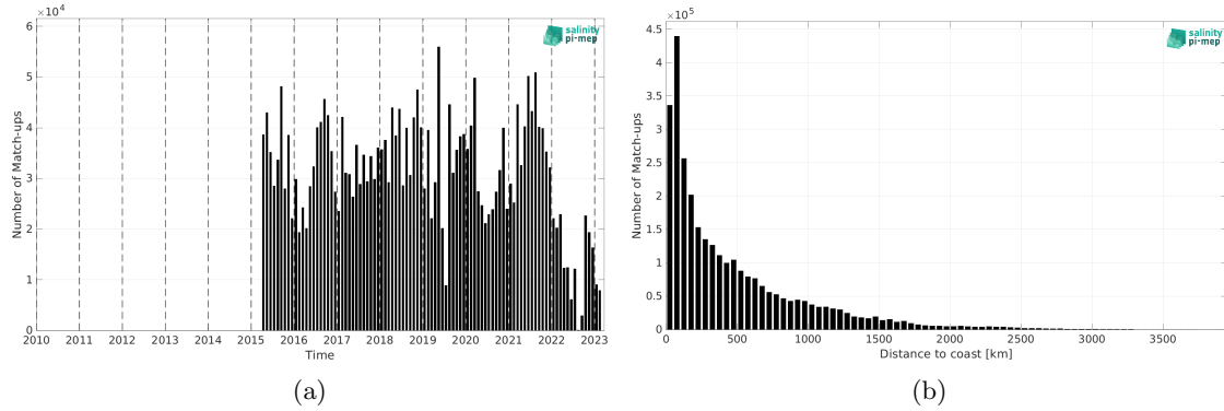
Figure 2: Number of match-ups between TSG (LEGOS-DM) and SMAP SSS L2 v5.3 - 40 km (RSS) SSS as a function of time (a) and as function of the distance to coast (b) over the Global Ocean Pi-MEP region and for the full satellite product period.
