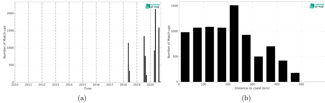
Figure 2: Number of match-ups between TSG (Lauge-Koch) and SMAP SSS L2 v5.3 - 40 km (RSS) SSS as a function of time (a) and as function of the distance to coast (b) over the Global Ocean Pi-MEP region and for the full satellite product period.
