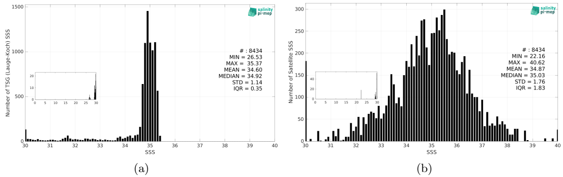
Figure 3: Histograms of SSS from TSG (Lauge-Koch) (a) and SMAP SSS L2 v5.3 - 40 km (RSS) (b) considering all match-up pairs per bins of 0.1 over the Global Ocean Pi-MEP region and for the full satellite product period.
