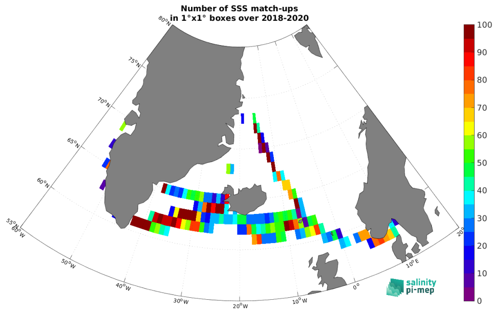
Figure 5: Number of SSS match-ups between TSG (Lauge-Koch) SSS and the SMAP SSS L2 v5.3 - 40 km (RSS) SSS product for the Global Ocean Pi-MEP region over 1^\circ \times 1^\circ boxes and for the full satellite product period.
