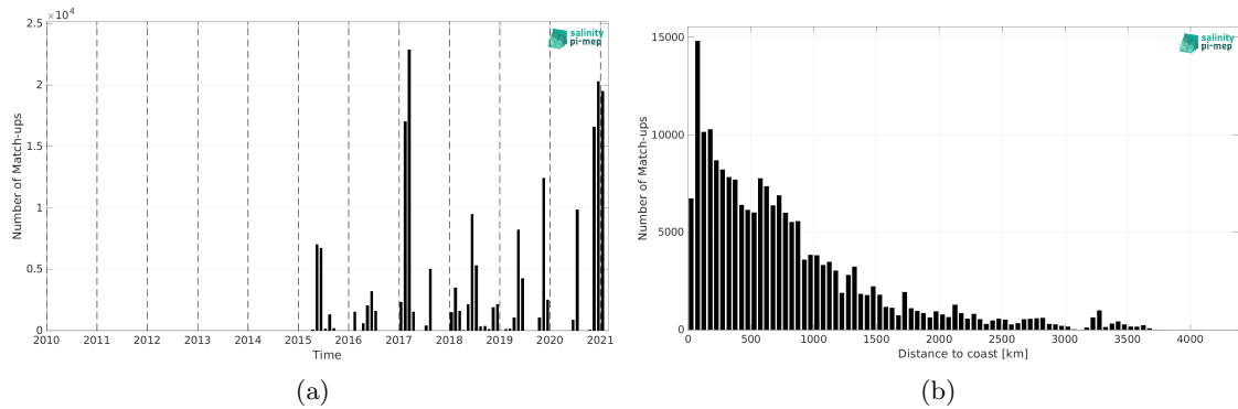
Figure 2: Number of match-ups between TSG (GOSUD-Sailing-ship) and SMAP SSS L2 v5.3 - 40 km (RSS) SSS as a function of time (a) and as function of the distance to coast (b) over the Global Ocean Pi-MEP region and for the full satellite product period.
