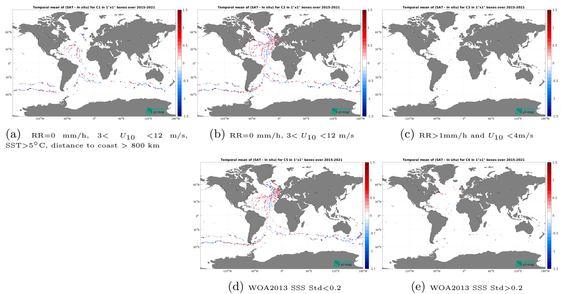
Figure 14: Temporal mean gridded over spatial boxes of size 1^\circ \times 1^\circ of \Delta\text{SSS} (SMAP SSS L2 v5.3 - 40 km (RSS) - TSG (GOSUD-Sailing-ship)) for 5 different subdatasets corresponding to: RR=0 mm/h, 3 < U_{10} < 12 m/s, SST > 5°C, distance to coast > 800 km (a), RR=0 mm/h, 3 < U_{10} < 12 m/s (b), RR > 1mm/h and U_{10} < 4 m/s (c), WOA2013 SSS Std < 0.2 (d), WOA2013 SSS Std > 0.2 (e).
