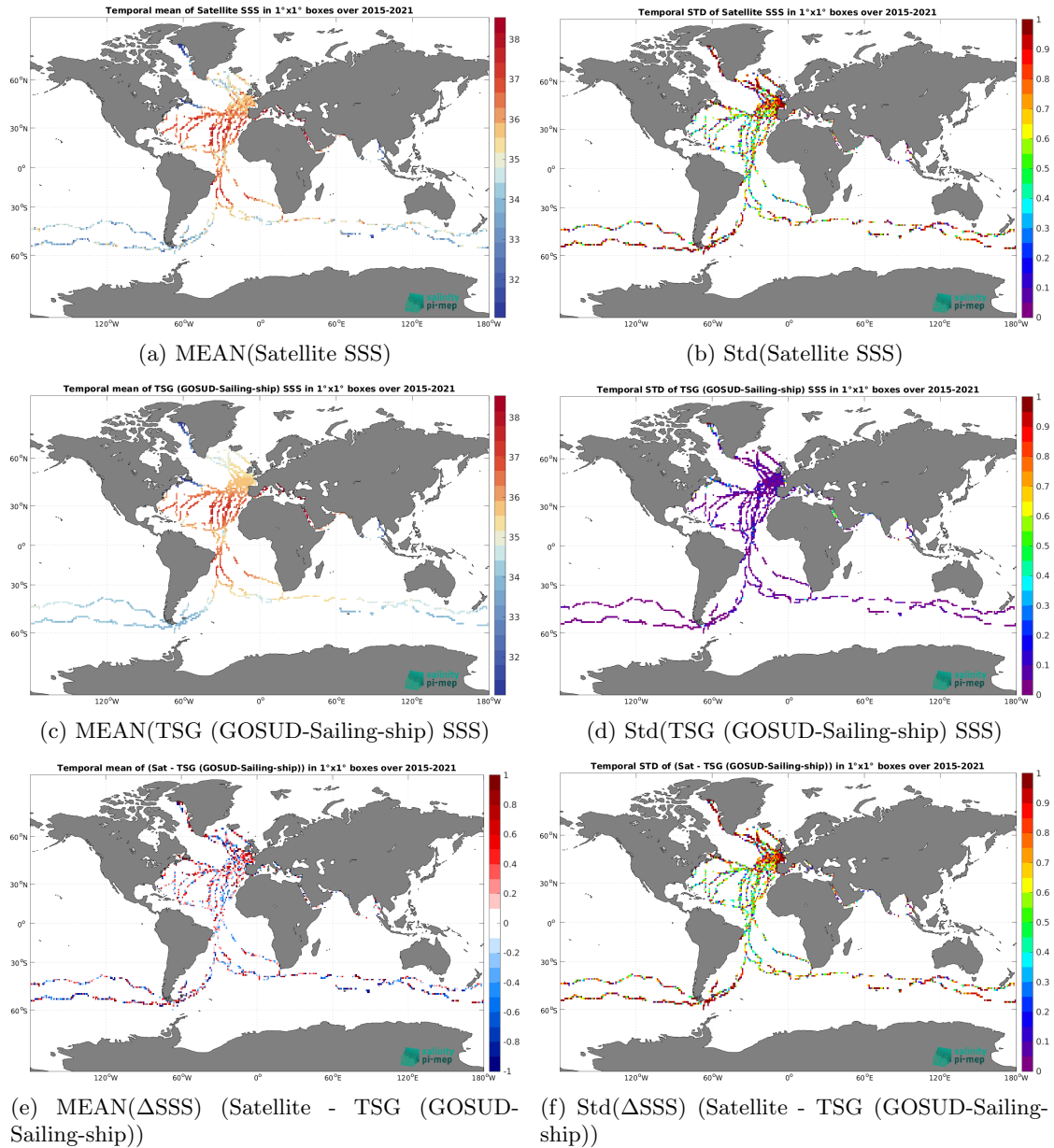
Figure 7: Temporal mean (left) and Std (right) of SSS from SMAP SSS L2 v5.3 - 40 km (RSS) (top), TSG (GOSUD-Sailing-ship) (middle), and of \Delta SSS (Satellite - TSG (GOSUD-Sailing-ship)). Only match-up pairs are used to generate these maps.
