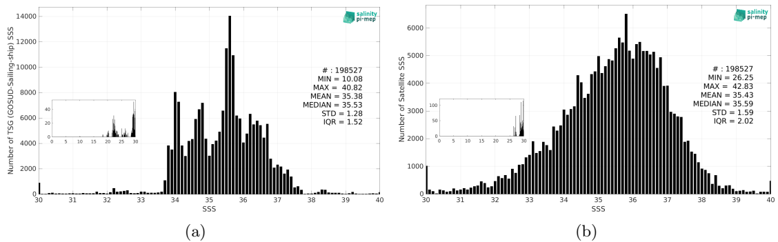
Figure 3: Histograms of SSS from TSG (GOSUD-Sailing-ship) (a) and SMAP SSS L2 v5.3 - 40 km (RSS) (b) considering all match-up pairs per bins of 0.1 over the Global Ocean Pi-MEP region and for the full satellite product period.
