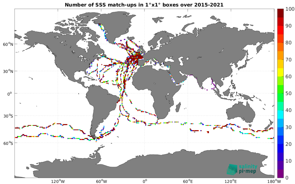
Figure 5: Number of SSS match-ups between TSG (GOSUD-Sailing-ship) SSS and the SMAP SSS L2 v5.3 - 40 km (RSS) SSS product for the Global Ocean Pi-MEP region over 1^\circ \times 1^\circ boxes and for the full satellite product period.
