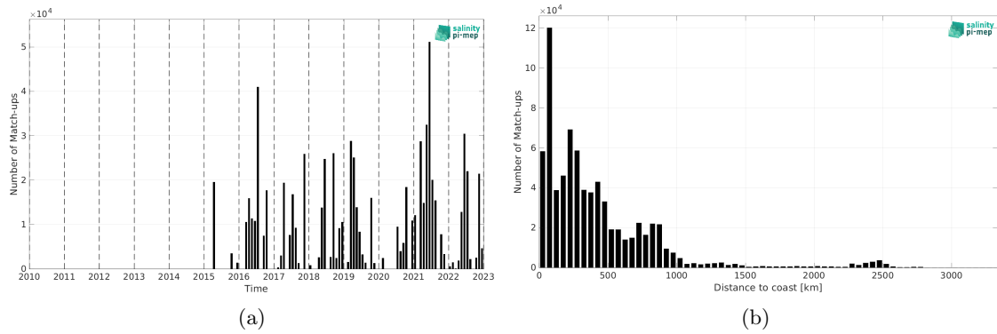
Figure 2: Number of match-ups between TSG (CSIC-UTM) and SMAP SSS L2 v5.3 - 40 km (RSS) SSS as a function of time (a) and as function of the distance to coast (b) over the Global Ocean Pi-MEP region and for the full satellite product period.
