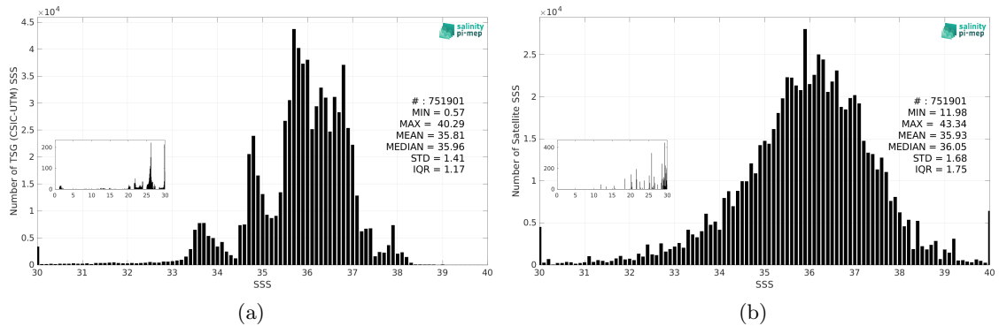
Figure 3: Histograms of SSS from TSG (CSIC-UTM) (a) and SMAP SSS L2 v5.3 - 40 km (RSS) (b) considering all match-up pairs per bins of 0.1 over the Global Ocean Pi-MEP region and for the full satellite product period.
