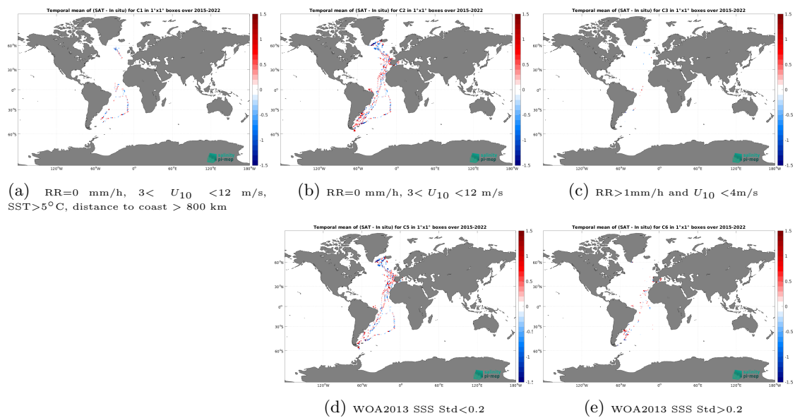
Figure 14: Temporal mean gridded over spatial boxes of size 1^\circ \times 1^\circ of \Delta\text{SSS} (SMAP SSS L2 v5.3 - 40 km (RSS) - TSG (CSIC-UTM)) for 5 different subdatasets corresponding to:RR=0 mm/h, 3 < U_{10} < 12 m/s, SST > 5^\circ\text{C} , distance to coast > 800 km (a), RR=0 mm/h, 3 < U_{10} < 12 m/s (b), RR > 1 mm/h and U_{10} < 4 m/s (c), WOA2013 SSS Std < 0.2 (d), WOA2013 SSS Std > 0.2 (e).
